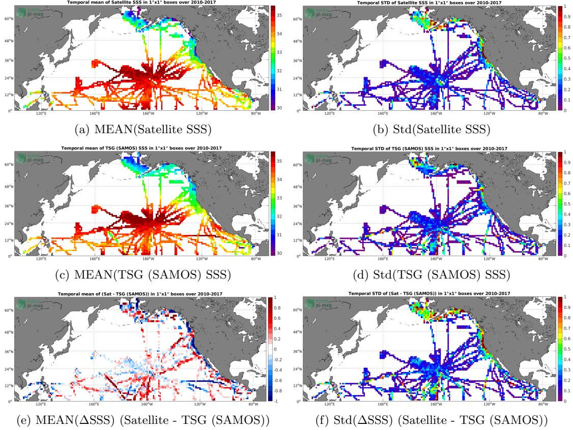
Figure 6: Temporal mean (left) and Std (right) of SSS from SMOS SSS L3 v2 - Monthly - 0.25 Deg (CATDS-CECOS-IFREMER) (top), TSG (SAMOS) (middle), and of \Delta SSS (Satellite - TSG (SAMOS)). Only match-up pairs are used to generate these maps.
