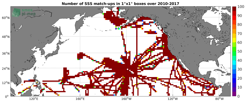
Figure 4: Number of SSS match-ups between TSG (SAMOS) SSS and the SMOS SSS L3 v2 - Monthly - 0.25 Deg (CATDS-CECOS-IFREMER) SSS product for the North Pacific Ocean Pi-MEP region over 1^\circ \times 1^\circ boxes and for the full satellite product period.
