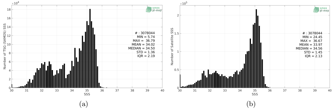
Figure 2: Histograms of SSS from TSG (SAMOS) (a) and SMOS SSS L3 v2 - Monthly - 0.25 Deg (CATDS-CECOS-IFREMER) (b) considering all match-up pairs per bins of 0.1 over the North Pacific Ocean Pi-MEP region and for the full satellite product period.
