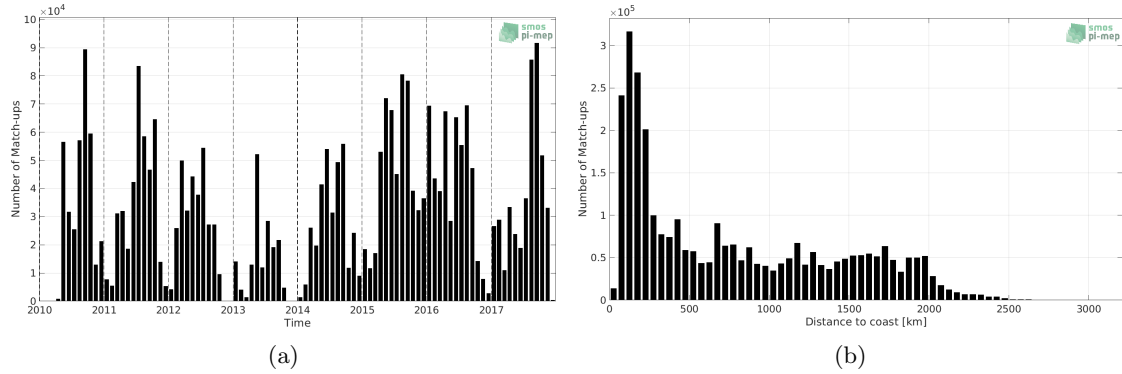
Figure 1: Number of match-ups between TSG (SAMOS) and SMOS SSS L3 v2 - Monthly - 0.25 Deg (CATDS-CECOS-IFREMER) SSS as a function of time (a) and as function of the distance to coast (b) over the North Pacific Ocean Pi-MEP region and for the full satellite product period.
