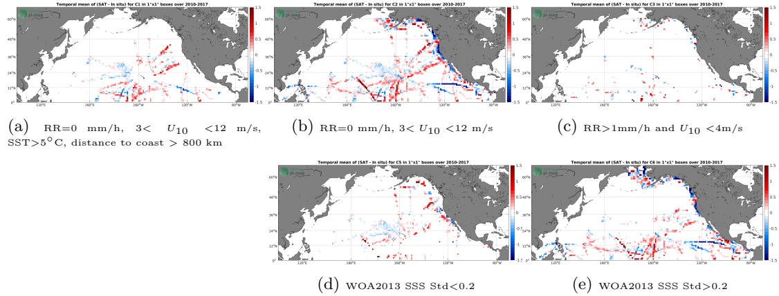
Figure 12: Temporal mean gridded over spatial boxes of size 1^\circ \times 1^\circ of \Delta SSS (SMOS SSS L3 v2 - Monthly - 0.25 Deg (CATDS-CECOS-IFREMER) - TSG (SAMOS)) for 5 different subdatasets corresponding to: RR=0 mm/h, 3 < U_{10} < 12 m/s, SST > 5^\circ\text{C} , distance to coast > 800 km (a), RR=0 mm/h, 3 < U_{10} < 12 m/s (b), RR > 1 mm/h and U_{10} < 4 m/s (c), WOA2013 SSS Std < 0.2 (d), WOA2013 SSS Std > 0.2 (e).
