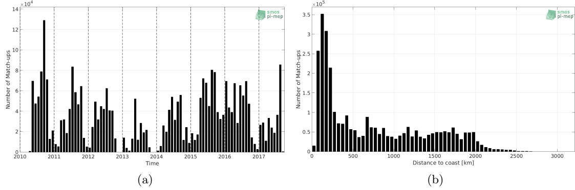
Figure 1: Number of match-ups between TSG-SAMOS and SMOS L3 v2 - Monthly - 0.25 Deg (CATDS-CECOS-IFREMER) SSS as a function of time (a) and as function of the distance to coast (b) over the North Pacific Ocean Pi-MEP region and for the full satellite product period.
