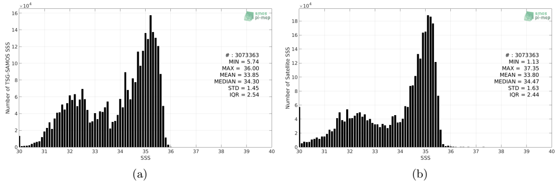
Figure 2: Histograms of SSS from TSG-SAMOS (a) and SMOS L3 v2 - Monthly - 0.25 Deg (CATDS-CECOS-IFREMER) (b) considering all match-up pairs per bins of 0.1 over the North Pacific Ocean Pi-MEP region and for the full satellite product period.
