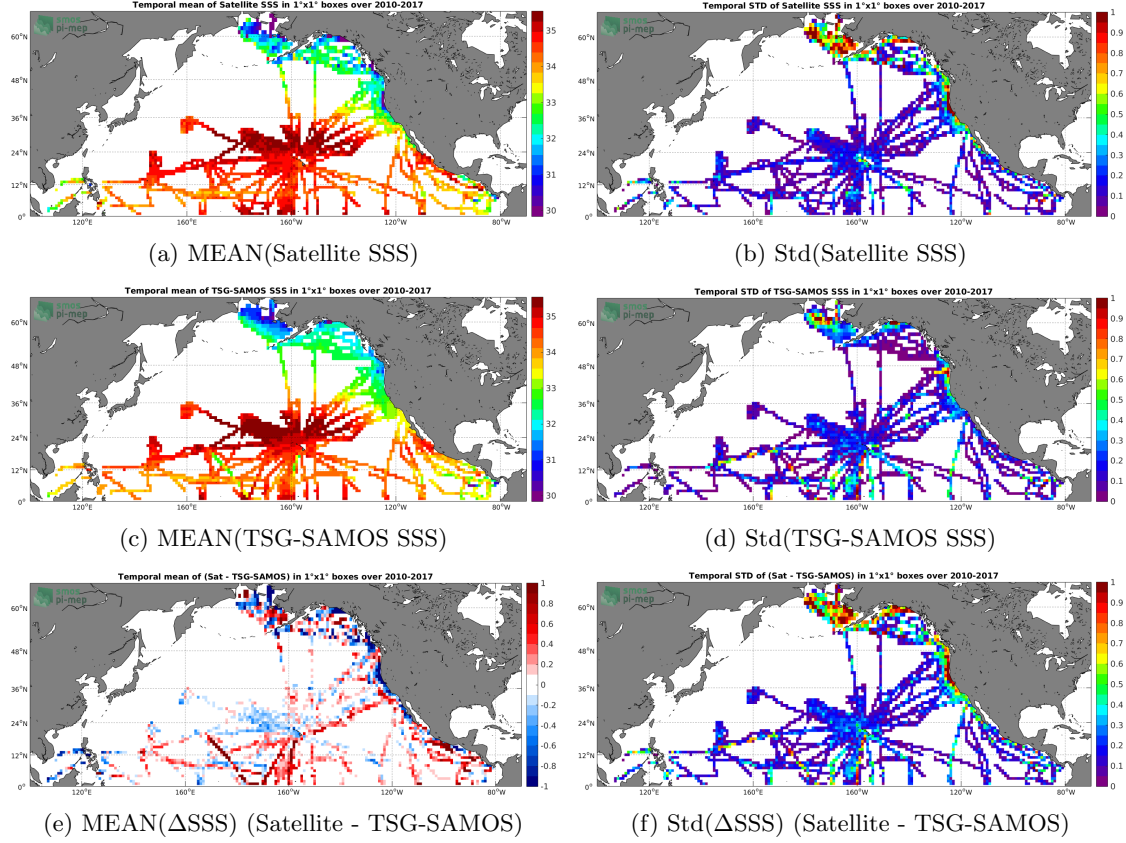
Figure 6: Temporal mean (left) and Std (right) of SSS from SMOS L3 v2 - Monthly - 0.25 Deg (CATDS-CECOS-IFREMER) (top), TSG-SAMOS (middle), and of \Delta SSS (Satellite - TSG-SAMOS). Only match-up pairs are used to generate these maps.
