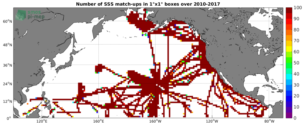
Figure 4: Number of SSS match-ups between TSG-SAMOS SSS and the SMOS L3 v2 - Monthly - 0.25 Deg (CATDS-CECOS-IFREMER) SSS product for the North Pacific Ocean Pi-MEP region over 1°x1° boxes and for the full satellite product period.
