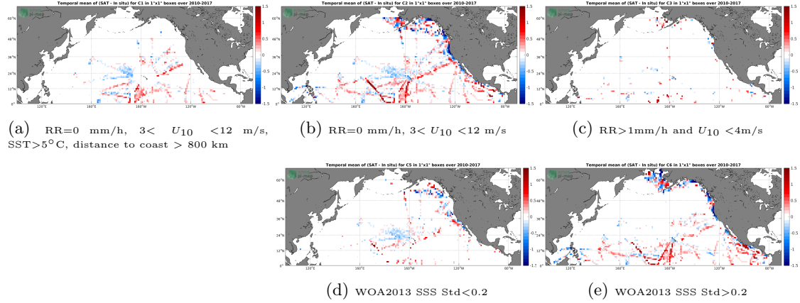
Figure 12: Temporal mean gridded over spatial boxes of size 1^\circ \times 1^\circ of \Delta SSS (SMOS L3 v2 - Monthly - 0.25 Deg (CATDS-CECOS-IFREMER) - TSG-SAMOS) for 5 different subdatasets corresponding to: RR=0 mm/h, 3 < U_{10} < 12 m/s, SST > 5^\circ C , distance to coast > 800 km (a), RR=0 mm/h, 3 < U_{10} < 12 m/s (b), RR > 1 mm/h and U_{10} < 4 m/s (c), WOA2013 SSS Std < 0.2 (d), WOA2013 SSS Std > 0.2 (e).
