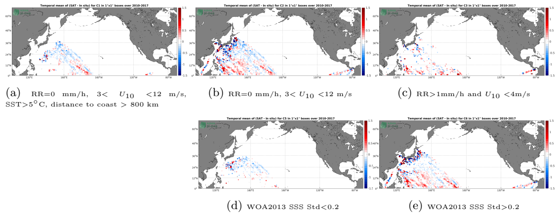
Figure 12: Temporal mean gridded over spatial boxes of size 1^\circ \times 1^\circ of \Delta SSS (SMOS SSS L3 v2 - Monthly - 0.25 Deg (CATDS-CECOS-IFREMER) - TSG (LEGOS-DM)) for 5 different subdatasets corresponding to:RR=0 mm/h, 3 < U_{10} < 12 m/s, SST >5^\circ\text{C} , distance to coast > 800 km (a), RR=0 mm/h, 3 < U_{10} < 12 m/s (b), RR >1 mm/h and U_{10} < 4 m/s (c), WOA2013 SSS Std <0.2 (d), WOA2013 SSS Std >0.2 (e).
