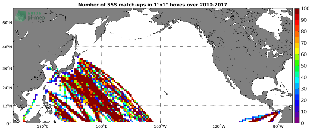
Figure 4: Number of SSS match-ups between TSG (LEGOS-DM) SSS and the SMOS SSS L3 v2 - Monthly - 0.25 Deg (CATDS-CECOS-IFREMER) SSS product for the North Pacific Ocean Pi-MEP region over 1°x1° boxes and for the full satellite product period.
