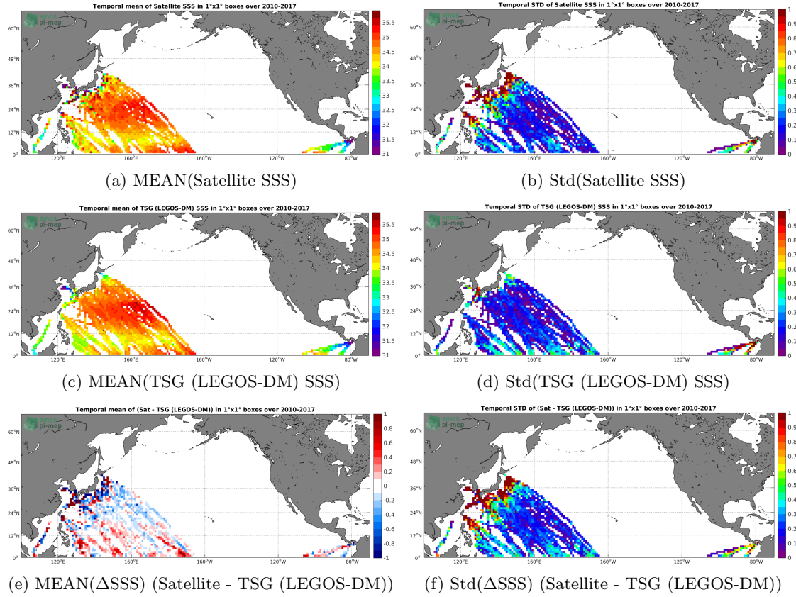
Figure 6: Temporal mean (left) and Std (right) of SSS from SMOS SSS L3 v2 - Monthly - 0.25 Deg (CATDS-CECOS-IFREMER) (top), TSG (LEGOS-DM) (middle), and of \Delta SSS (Satellite - TSG (LEGOS-DM)). Only match-up pairs are used to generate these maps.
