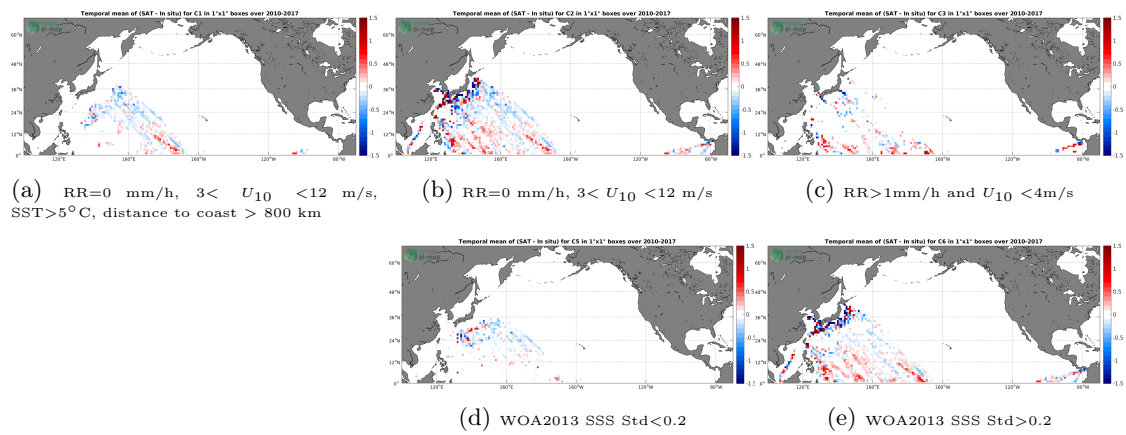
Figure 12: Temporal mean gridded over spatial boxes of size 1^\circ \times 1^\circ of \Delta\text{SSS} (SMOS SSS L3 v2 - Monthly - 0.25 Deg (CATDS-CECOS-IFREMER) - TSG (LEGOS-DM)) for 5 different subdatasets corresponding to:RR=0 mm/h, 3 < U_{10} < 12 m/s, SST >5^\circ\text{C} , distance to coast > 800 km (a), RR=0 mm/h, 3 < U_{10} < 12 m/s (b), RR >1 mm/h and U_{10} < 4 m/s (c), WOA2013 SSS Std <0.2 (d), WOA2013 SSS Std >0.2 (e).
