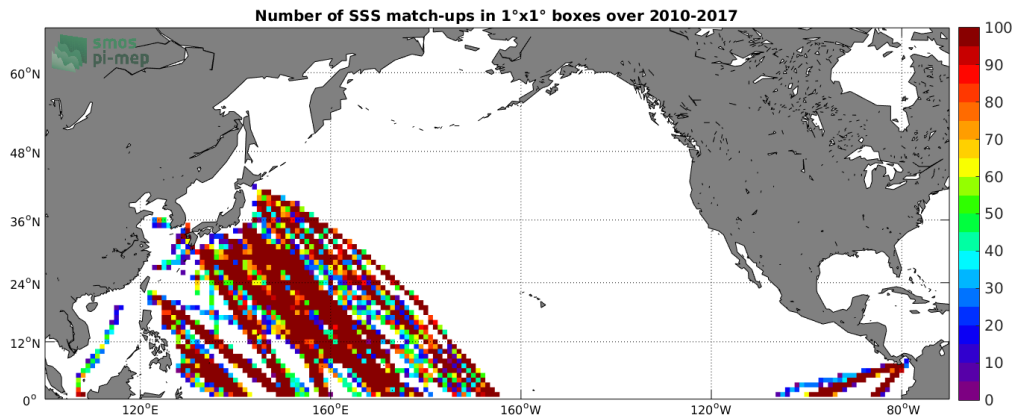
Figure 4: Number of SSS match-ups between TSG (LEGOS-DM) SSS and the SMOS SSS L3 v2 - Monthly - 0.25 Deg (CATDS-CECOS-IFREMER) SSS product for the North Pacific Ocean Pi-MEP region over 1^\circ \times 1^\circ boxes and for the full satellite product period.
