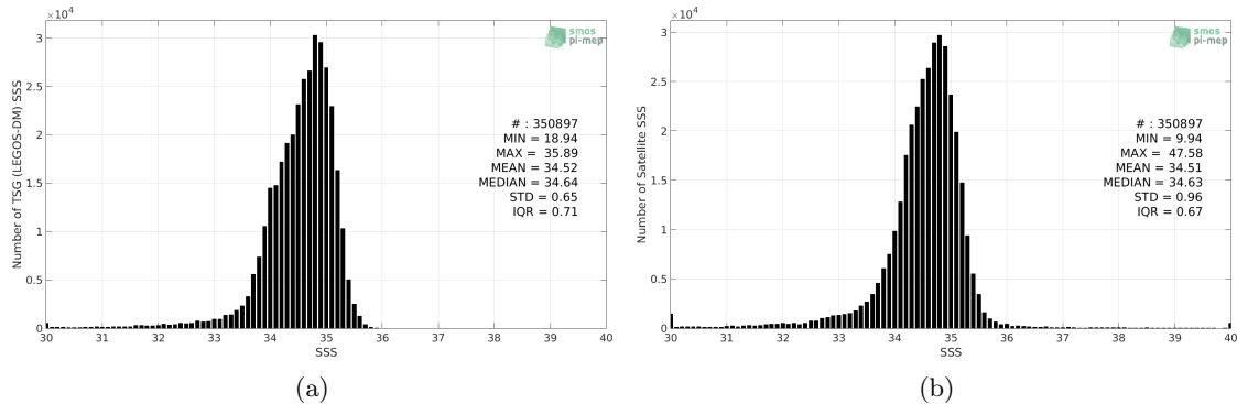
Figure 2: Histograms of SSS from TSG (LEGOS-DM) (a) and SMOS SSS L3 v2 - Monthly - 0.25 Deg (CATDS-CECOS-IFREMER) (b) considering all match-up pairs per bins of 0.1 over the North Pacific Ocean Pi-MEP region and for the full satellite product period.
