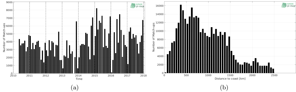
Figure 1: Number of match-ups between TSG (LEGOS-DM) and SMOS SSS L3 v2 - Monthly - 0.25 Deg (CATDS-CECOS-IFREMER) SSS as a function of time (a) and as function of the distance to coast (b) over the North Pacific Ocean Pi-MEP region and for the full satellite product period.
