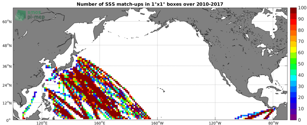
Figure 4: Number of SSS match-ups between TSG-LEGOS-DM SSS and the SMOS L3 v2 - Monthly - 0.25 Deg (CATDS-CECOS-IFREMER) SSS product for the North Pacific Ocean Pi-MEP region over 1°x1° boxes and for the full satellite product period.
