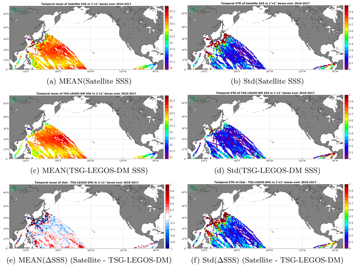
Figure 6: Temporal mean (left) and Std (right) of SSS from SMOS L3 v2 - Monthly - 0.25 Deg (CATDS-CECOS-IFREMER) (top), TSG-LEGOS-DM (middle), and of \Delta SSS (Satellite - TSG-LEGOS-DM). Only match-up pairs are used to generate these maps.
