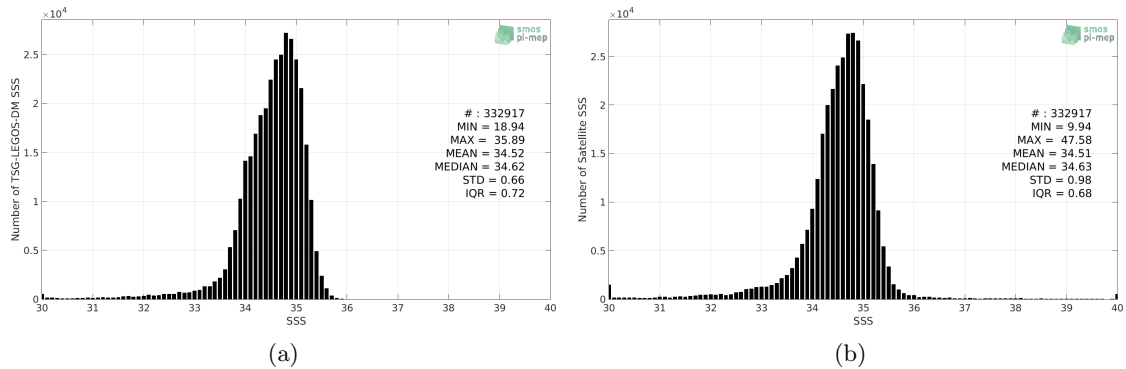
Figure 2: Histograms of SSS from TSG-LEGOS-DM (a) and SMOS L3 v2 - Monthly - 0.25 Deg (CATDS-CECOS-IFREMER) (b) considering all match-up pairs per bins of 0.1 over the North Pacific Ocean Pi-MEP region and for the full satellite product period.
