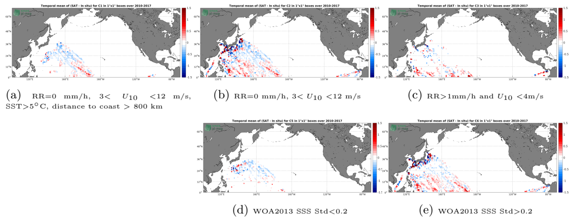
Figure 12: Temporal mean gridded over spatial boxes of size 1^\circ \times 1^\circ of \Delta SSS (SMOS L3 v2 - Monthly - 0.25 Deg (CATDS-CECOS-IFREMER) - TSG-LEGOS-DM) for 5 different subdatasets corresponding to:RR=0 mm/h, 3 < U_{10} < 12 m/s, SST >5^\circ\text{C} , distance to coast > 800 km (a), RR=0 mm/h, 3 < U_{10} < 12 m/s (b), RR >1 mm/h and U_{10} < 4 m/s (c), WOA2013 SSS Std <0.2 (d), WOA2013 SSS Std >0.2 (e).
