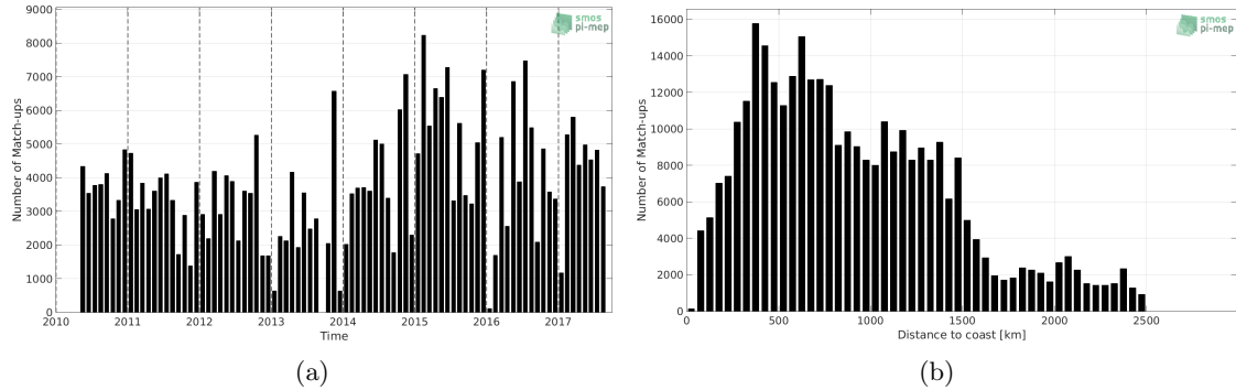
Figure 1: Number of match-ups between TSG-LEGOS-DM and SMOS L3 v2 - Monthly - 0.25 Deg (CATDS-CECOS-IFREMER) SSS as a function of time (a) and as function of the distance to coast (b) over the North Pacific Ocean Pi-MEP region and for the full satellite product period.
