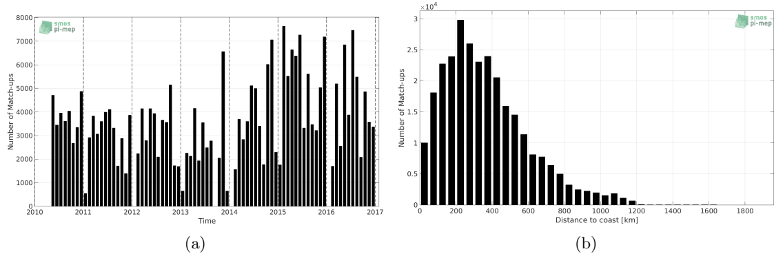
Figure 1: Number of match-ups between TSG-LEGOS-DM and SMOS-L3-CATDS-IFREMER-CECOS-V2-MONTHLY-0.25DEG SSS as a function of time (a) and as function of the distance to coast (b) over the North Pacific Ocean Pi-MEP region and for the full satellite product period.
