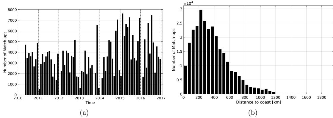
Figure 1: Number of match-ups between TSG-LEGOS-DM and SMOS-L3-CATDS-IFREMER-CECOS-V2-MONTHLY-0.25DEG SSS as a function of time (a) and as function of the distance to coast (b) over the North Pacific Ocean Pi-MEP region and for the full satellite product period.
