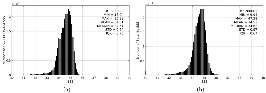
Figure 2: Histograms of SSS from TSG-LEGOS-DM (a) and SMOS-L3-CATDS-IFREMER-CECOS-V2-MONTHLY-0.25DEG (b) considering all match-up pairs per bins of 0.1 over the North Pacific Ocean Pi-MEP region and for the full satellite product period.
