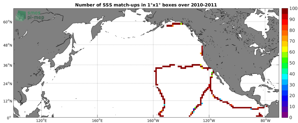
Figure 4: Number of SSS match-ups between TSG-GOSUD-Sailing-ship SSS and the SMOS L3 v2 - Monthly - 0.25 Deg (CATDS-CECOS-IFREMER) SSS product for the North Pacific Ocean Pi-MEP region over 1^\circ \times 1^\circ boxes and for the full satellite product period.
