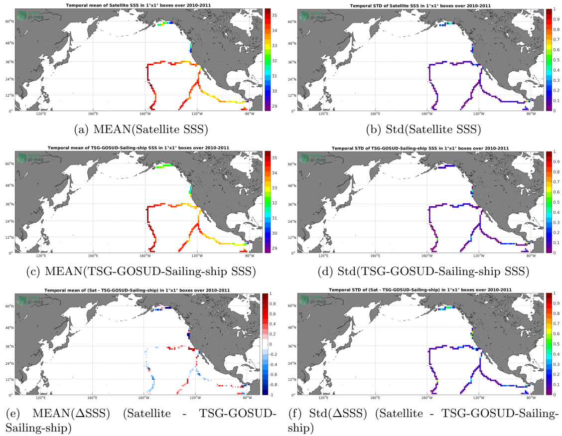
Figure 6: Temporal mean (left) and Std (right) of SSS from SMOS L3 v2 - Monthly - 0.25 Deg (CATDS-CECOS-IFREMER) (top), TSG-GOSUD-Sailing-ship (middle), and of \Delta SSS (Satellite - TSG-GOSUD-Sailing-ship). Only match-up pairs are used to generate these maps.
