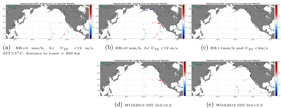
Figure 12: Temporal mean gridded over spatial boxes of size 1^\circ \times 1^\circ of \Delta SSS (SMOS L3 v2 - Monthly - 0.25 Deg (CATDS-CECOS-IFREMER) - TSG-GOSUD-Sailing-ship) for 5 different subdatasets corresponding to:RR=0 mm/h, 3 < U_{10} < 12 m/s, SST>5°C, distance to coast > 800 km (a), RR=0 mm/h, 3 < U_{10} < 12 m/s (b), RR>1mm/h and U_{10} < 4 m/s (c), WOA2013 SSS Std<0.2 (d), WOA2013 SSS Std>0.2 (e).
