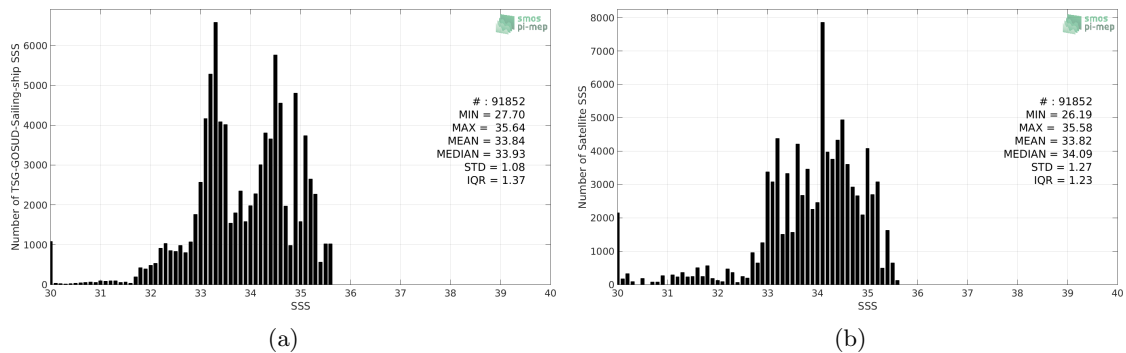
Figure 2: Histograms of SSS from TSG-GOSUD-Sailing-ship (a) and SMOS L3 v2 - Monthly - 0.25 Deg (CATDS-CECOS-IFREMER) (b) considering all match-up pairs per bins of 0.1 over the North Pacific Ocean Pi-MEP region and for the full satellite product period.
