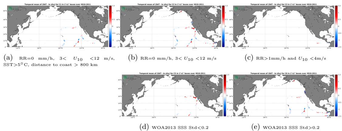
Figure 12: Temporal mean gridded over spatial boxes of size 1^\circ \times 1^\circ of \Delta SSS (SMOS-L3-CATDS-IFREMER-CECOS-V2-MONTHLY-0.25DEG - TSG-GOSUD-Sailing-ship) for 5 different sub-datasets corresponding to:RR=0 mm/h, 3 < U_{10} < 12 m/s, SST >5^\circ C, distance to coast > 800 km (a), RR=0 mm/h, 3 < U_{10} < 12 m/s (b), RR >1 mm/h and U_{10} < 4 m/s (c), WOA2013 SSS Std <0.2 (d), WOA2013 SSS Std >0.2 (e).
