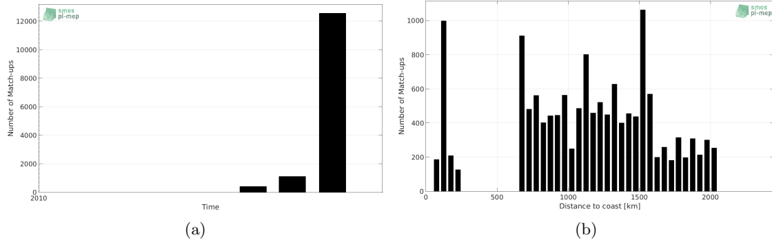
Figure 1: Number of match-ups between TSG-GOSUD-Sailing-ship and SMOS-L3-CATDS-IFREMER-CECOS-V2-MONTHLY-0.25DEG SSS as a function of time (a) and as function of the distance to coast (b) over the North Pacific Ocean Pi-MEP region and for the full satellite product period.
