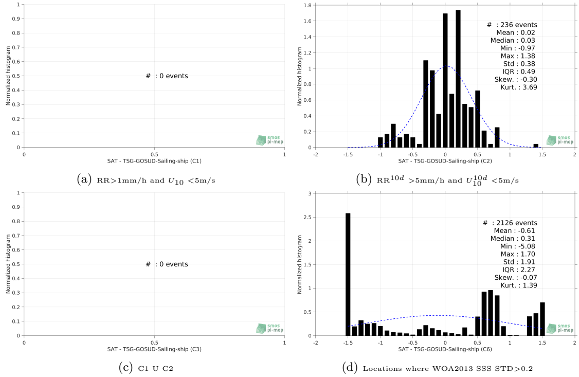
Figure 13: Normalized histogram of \Delta SSS (SMOS-L3-CATDS-IFREMER-CECOS-V2-MONTHLY-0.25DEG - TSG-GOSUD-Sailing-ship) for 6 different subdatasets corresponding to: RR > 1\text{mm/h} and U_{10} < 5\text{m/s} (a), RR^{10d} > 5\text{mm/h} and U_{10}^{10d} < 5\text{m/s} (b), C1 \cup C2 (c), Locations where WOA2013 SSS STD > 0.2 (d).
