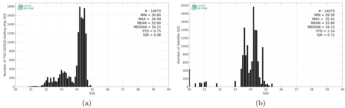
Figure 2: Histograms of SSS from TSG-GOSUD-Sailing-ship (a) and SMOS-L3-CATDS-IFREMER-CECOS-V2-MONTHLY-0.25DEG (b) considering all match-up pairs per bins of 0.1 over the North Pacific Ocean Pi-MEP region and for the full satellite product period.
