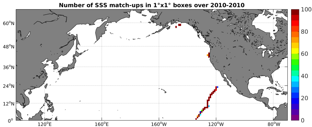
Figure 4: Number of SSS match-ups between TSG-GOSUD-Sailing-ship SSS and the SMOS-L3-CATDS-IFREMER-CECOS-V2-MONTHLY-0.25DEG SSS product for the North Pacific Ocean Pi-MEP region over 1^\circ \times 1^\circ boxes and for the full satellite product period.
