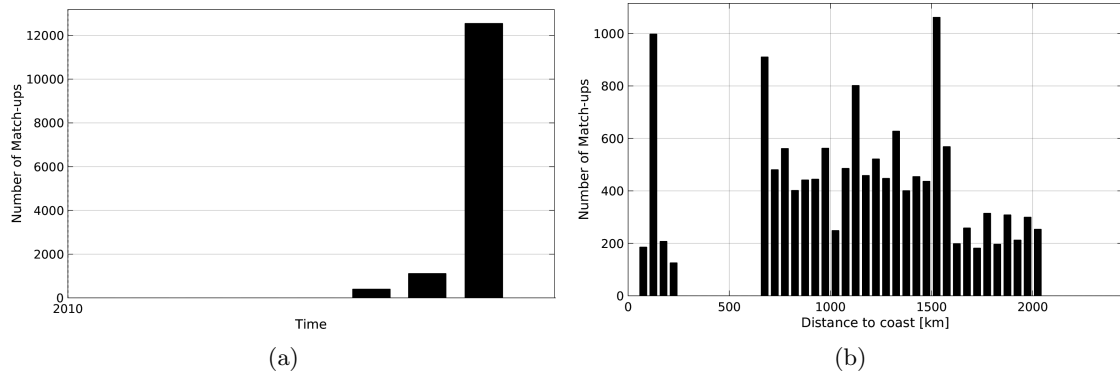
Figure 1: Number of match-ups between TSG-GOSUD-Sailing-ship and SMOS-L3-CATDS-IFREMER-CECOS-V2-MONTHLY-0.25DEG SSS as a function of time (a) and as function of the distance to coast (b) over the North Pacific Ocean Pi-MEP region and for the full satellite product period.
