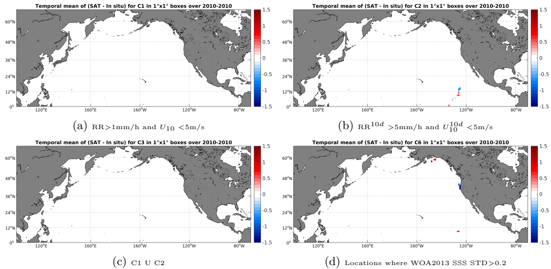
Figure 12: Temporal mean gridded over spatial boxes of size 1^\circ \times 1^\circ of \Delta SSS (SMOS-L3-CATDS-IFREMER-CECOS-V2-MONTHLY-0.25DEG - TSG-GOSUD-Sailing-ship) for 4 different sub-datasets corresponding to: RR > 1\text{mm/h} and U_{10} < 5\text{m/s} (a), RR^{10d} > 5\text{mm/h} and U_{10}^{10d} < 5\text{m/s} (b), C1 U C2 (c), Locations where WOA2013 SSS STD > 0.2 (d).
