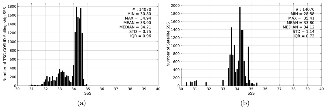
Figure 2: Histograms of SSS from TSG-GOSUD-Sailing-ship (a) and SMOS-L3-CATDS-IFREMER-CECOS-V2-MONTHLY-0.25DEG (b) considering all match-up pairs per bins of 0.1 over the North Pacific Ocean Pi-MEP region and for the full satellite product period.
