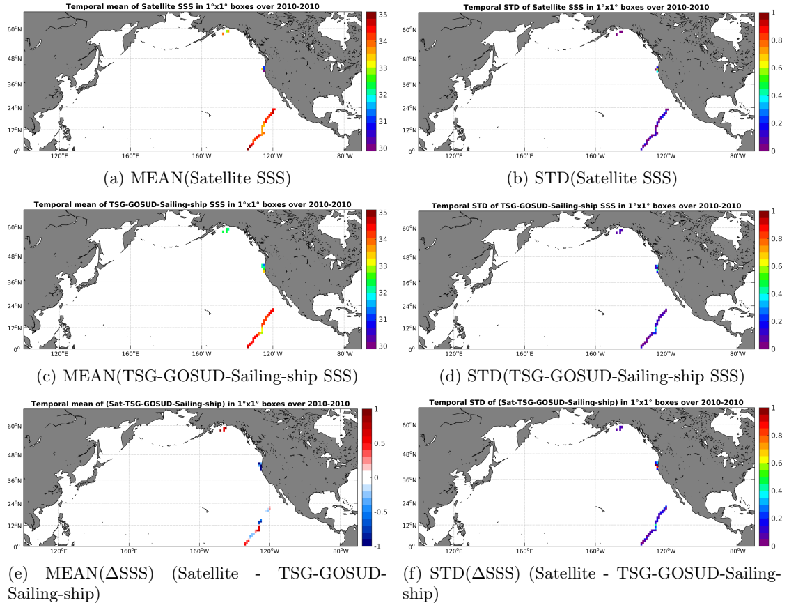
Figure 6: Temporal mean (left) and STD (right) of SSS from SMOS-L3-CATDS-IFREMER-CECOS-V2-MONTHLY-0.25DEG (top), TSG-GOSUD-Sailing-ship (middle), and of \Delta SSS (Satellite - TSG-GOSUD-Sailing-ship). Only match-up pairs are used to generate these maps.
