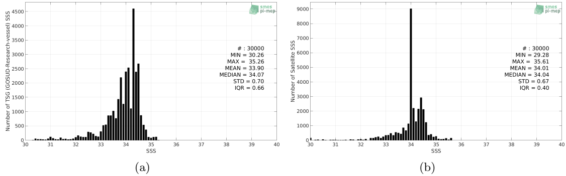
Figure 2: Histograms of SSS from TSG (GOSUD-Research-vessel) (a) and SMOS SSS L3 v2 - Monthly - 0.25 Deg (CATDS-CECOS-IFREMER) (b) considering all match-up pairs per bins of 0.1 over the North Pacific Ocean Pi-MEP region and for the full satellite product period.
