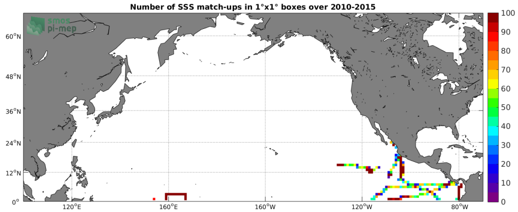
Figure 4: Number of SSS match-ups between TSG (GOSUD-Research-vessel) SSS and the SMOS SSS L3 v2 - Monthly - 0.25 Deg (CATDS-CECOS-IFREMER) SSS product for the North Pacific Ocean Pi-MEP region over 1°x1° boxes and for the full satellite product period.
