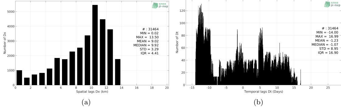
Figure 5: Histograms of the spatial (a) and temporal (b) lags between the time of the TSG-GOSUD-Research-vessel measurements and the date of the corresponding SMOS L3 v2 - Monthly - 0.25 Deg (CATDS-CECOS-IFREMER) SSS product.
