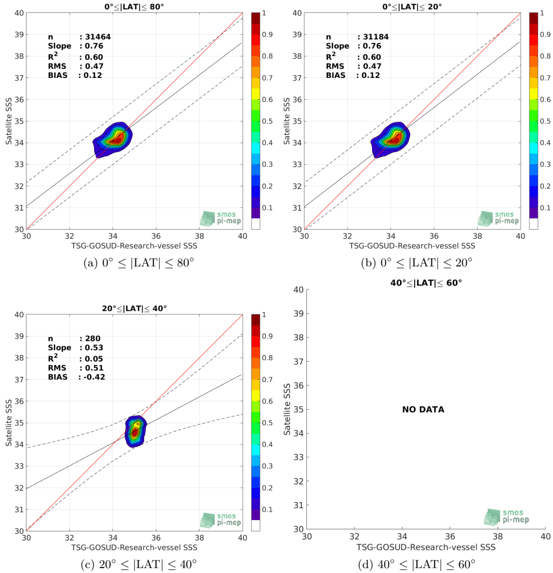
Figure 9: Contour maps of the concentration of SMOS L3 v2 - Monthly - 0.25 Deg (CATDS-CECOS-IFREMER) SSS (y-axis) versus TSG-GOSUD-Research-vessel SSS (x-axis) at match-up pairs for different latitude bands. For each plot, the red line shows x=y . The black thin and dashed lines indicate a linear fit through the data cloud and the \pm 95\% confidence levels, respectively. The number match-up pairs n , the slope and R^2 coefficient of the linear fit, the root mean square (RMS) and the mean bias between satellite and in situ data are indicated for each latitude band in each plots.
