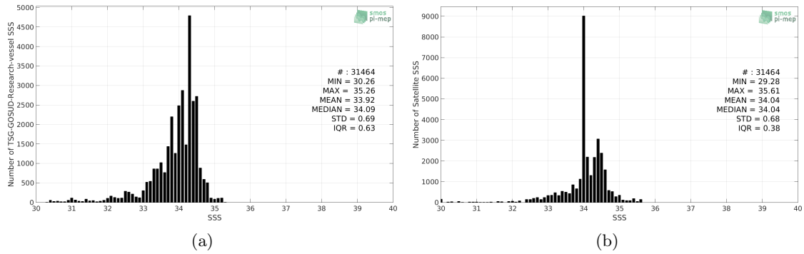
Figure 2: Histograms of SSS from TSG-GOSUD-Research-vessel (a) and SMOS L3 v2 - Monthly - 0.25 Deg (CATDS-CECOS-IFREMER) (b) considering all match-up pairs per bins of 0.1 over the North Pacific Ocean Pi-MEP region and for the full satellite product period.
