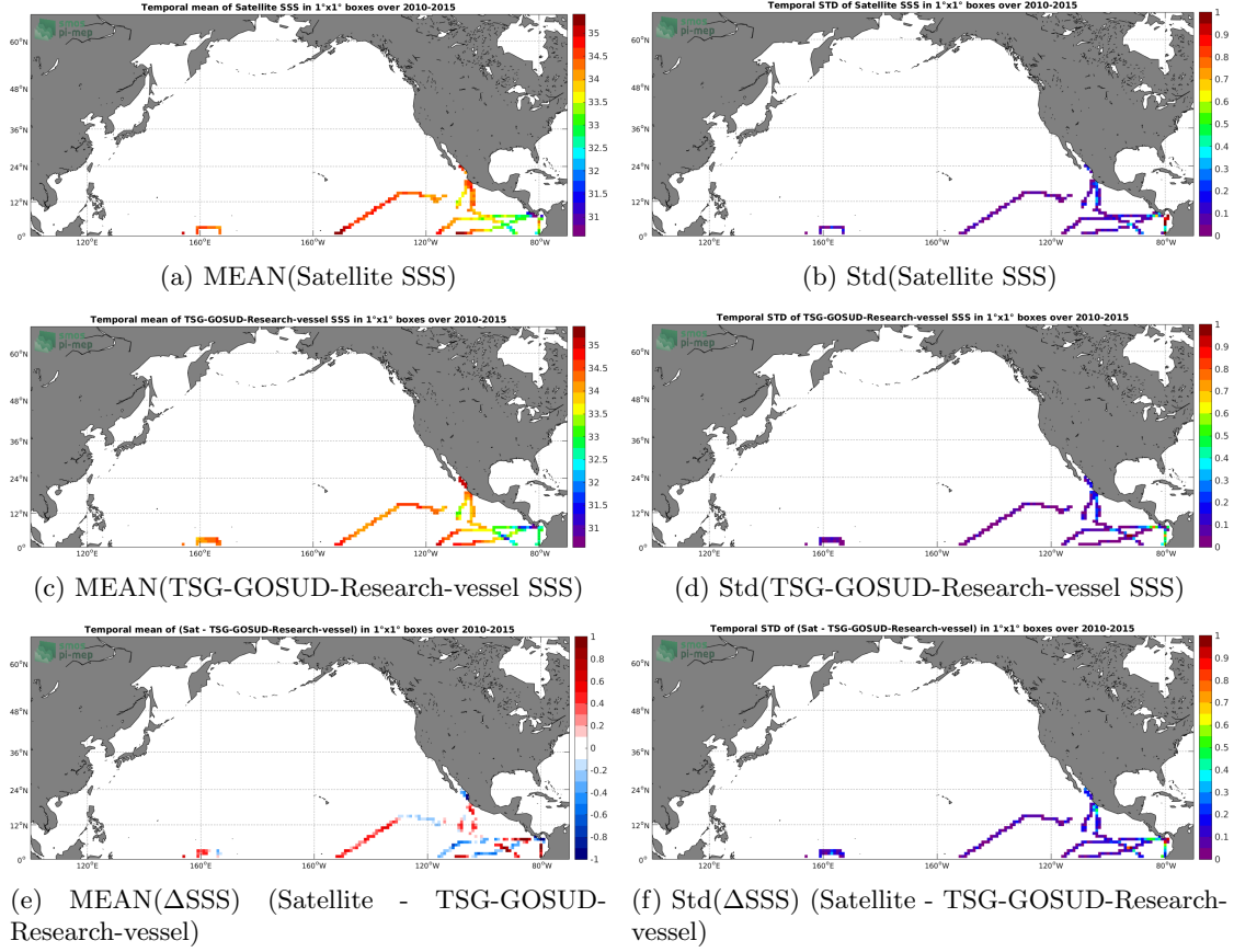
Figure 6: Temporal mean (left) and Std (right) of SSS from SMOS L3 v2 - Monthly - 0.25 Deg (CATDS-CECOS-IFREMER) (top), TSG-GOSUD-Research-vessel (middle), and of \Delta SSS (Satellite - TSG-GOSUD-Research-vessel). Only match-up pairs are used to generate these maps.
