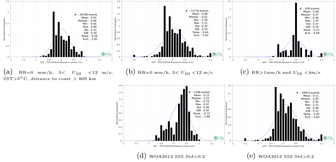
Figure 13: Normalized histogram of \Delta SSS (SMOS L3 v2 - Monthly - 0.25 Deg (CATDS-CECOS-IFREMER) - TSG-GOSUD-Research-vessel) for 5 different subdatasets corresponding to: RR=0 mm/h, 3 < U_{10} < 12 m/s, SST > 5°C, distance to coast > 800 km (a), RR=0 mm/h, 3 < U_{10} < 12 m/s (b), RR > 1 mm/h and U_{10} < 4 m/s (c), WOA2013 SSS Std < 0.2 (d), WOA2013 SSS Std > 0.2 (e).
