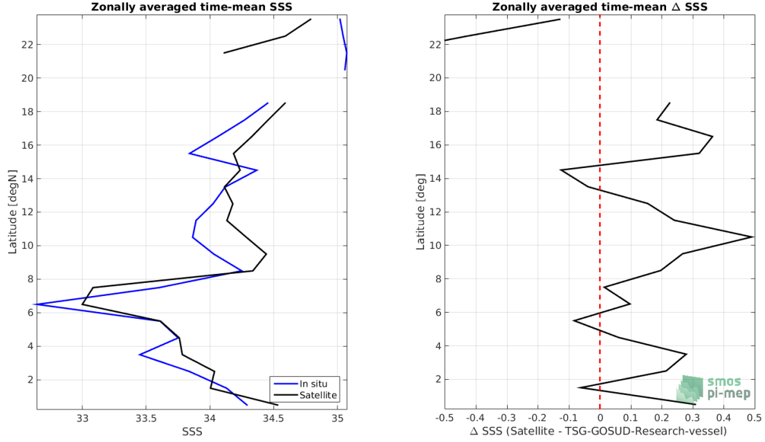
Figure 8: Left panel: Zonal mean SSS from SMOS L3 v2 - Monthly - 0.25 Deg (CATDS-CECOS-IFREMER) satellite product (black) and from TSG-GOSUD-Research-vessel (blue). Right panel: Zonal mean of \Delta SSS (Satellite - TSG-GOSUD-Research-vessel) for all the collected Pi-MEP match-up pairs estimated over the full satellite product period.
