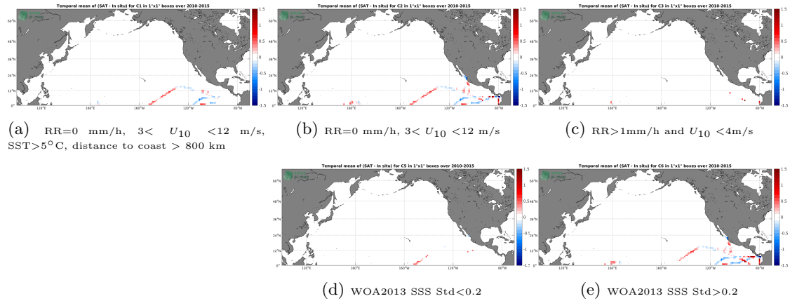
Figure 12: Temporal mean gridded over spatial boxes of size 1^\circ \times 1^\circ of \Delta SSS (SMOS L3 v2 - Monthly - 0.25 Deg (CATDS-CECOS-IFREMER) - TSG-GOSUD-Research-vessel) for 5 different subdatasets corresponding to: RR=0 mm/h, 3 < U_{10} < 12 m/s, SST >5^\circ\text{C} , distance to coast > 800 km (a), RR=0 mm/h, 3 < U_{10} < 12 m/s (b), RR >1 mm/h and U_{10} < 4 m/s (c), WOA2013 SSS Std <0.2 (d), WOA2013 SSS Std >0.2 (e).
