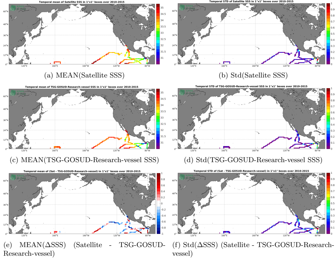
Figure 6: Temporal mean (left) and Std (right) of SSS from SMOS-L3-CATDS-IFREMER-CECOS-V2-MONTHLY-0.25DEG (top), TSG-GOSUD-Research-vessel (middle), and of \Delta SSS (Satellite - TSG-GOSUD-Research-vessel). Only match-up pairs are used to generate these maps.
