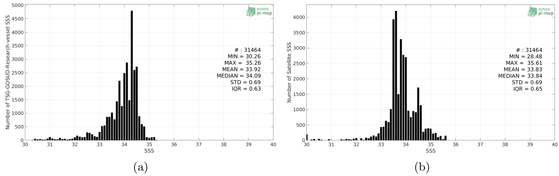
Figure 2: Histograms of SSS from TSG-GOSUD-Research-vessel (a) and SMOS-L3-CATDS-IFREMER-CECOS-V2-MONTHLY-0.25DEG (b) considering all match-up pairs per bins of 0.1 over the North Pacific Ocean Pi-MEP region and for the full satellite product period.
