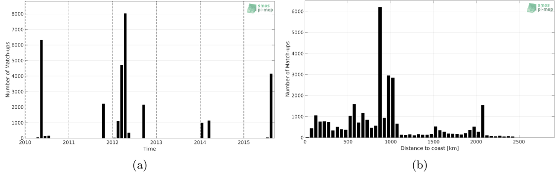
Figure 1: Number of match-ups between TSG-GOSUD-Research-vessel and SMOS-L3-CATDS-IFREMER-CECOS-V2-MONTHLY-0.25DEG SSS as a function of time (a) and as function of the distance to coast (b) over the North Pacific Ocean Pi-MEP region and for the full satellite product period.
