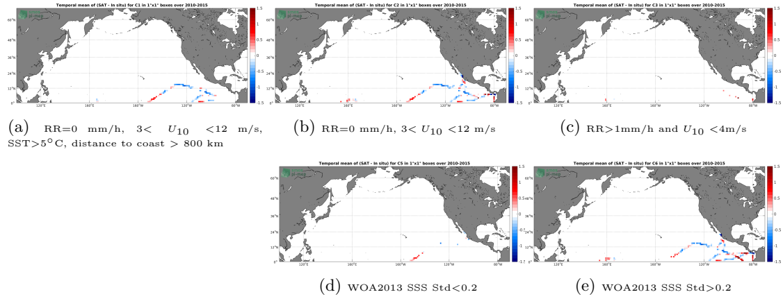
Figure 12: Temporal mean gridded over spatial boxes of size 1^\circ \times 1^\circ of \Delta SSS (SMOS-L3-CATDS-IFREMER-CECOS-V2-MONTHLY-0.25DEG - TSG-GOSUD-Research-vessel) for 5 different subdatasets corresponding to:RR=0 mm/h, 3 < U_{10} < 12 m/s, SST >5^\circ\text{C} , distance to coast > 800 km (a), RR=0 mm/h, 3 < U_{10} < 12 m/s (b), RR >1 mm/h and U_{10} < 4 m/s (c), WOA2013 SSS Std <0.2 (d), WOA2013 SSS Std >0.2 (e).
