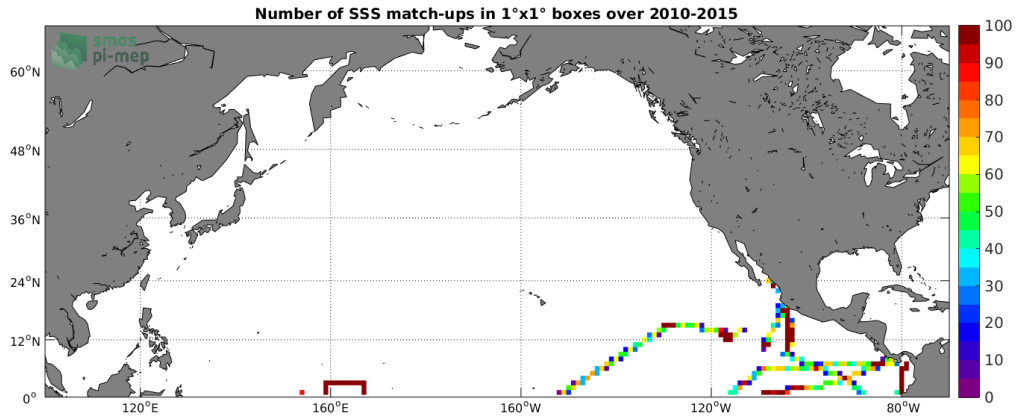
Figure 4: Number of SSS match-ups between TSG-GOSUD-Research-vessel SSS and the SMOS-L3-CATDS-IFREMER-CECOS-V2-MONTHLY-0.25DEG SSS product for the North Pacific Ocean Pi-MEP region over 1°x1° boxes and for the full satellite product period.
