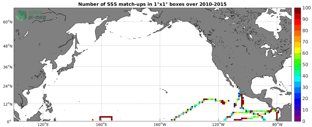
Figure 4: Number of SSS match-ups between TSG-GOSUD-Research-vessel SSS and the SMOS-L3-CATDS-IFREMER-CECOS-V2-MONTHLY-0.25DEG SSS product for the North Pacific Ocean Pi-MEP region over 1^\circ \times 1^\circ boxes and for the full satellite product period.
