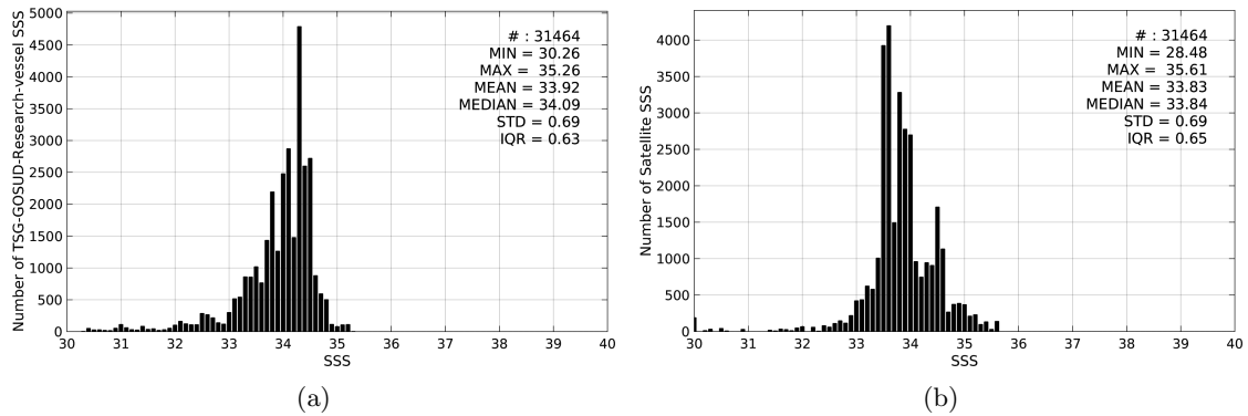
Figure 2: Histograms of SSS from TSG-GOSUD-Research-vessel (a) and SMOS-L3-CATDS-IFREMER-CECOS-V2-MONTHLY-0.25DEG (b) considering all match-up pairs per bins of 0.1 over the North Pacific Ocean Pi-MEP region and for the full satellite product period.
