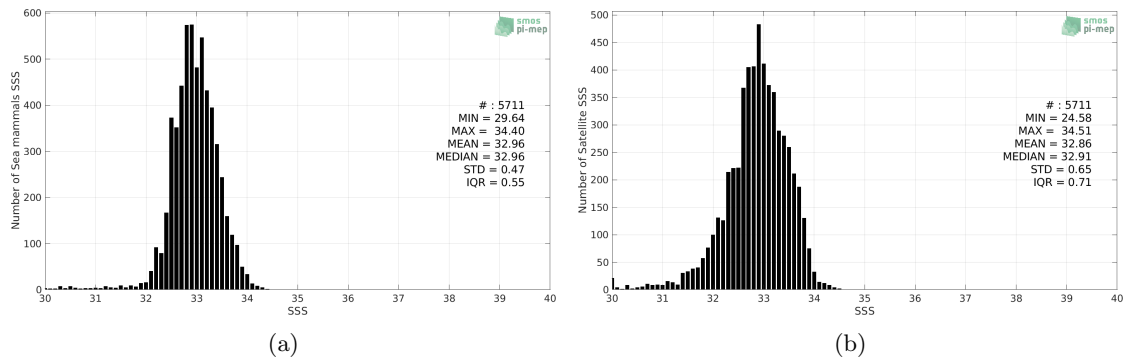
Figure 2: Histograms of SSS from Sea mammals (a) and SMOS SSS L3 v2 - Monthly - 0.25 Deg (CATDS-CECOS-IFREMER) (b) considering all match-up pairs per bins of 0.1 over the North Pacific Ocean Pi-MEP region and for the full satellite product period.
