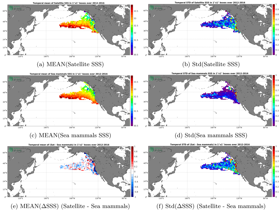
Figure 6: Temporal mean (left) and Std (right) of SSS from SMOS SSS L3 v2 - Monthly - 0.25 Deg (CATDS-CECOS-IFREMER) (top), Sea mammals (middle), and of \Delta SSS (Satellite - Sea mammals). Only match-up pairs are used to generate these maps.
