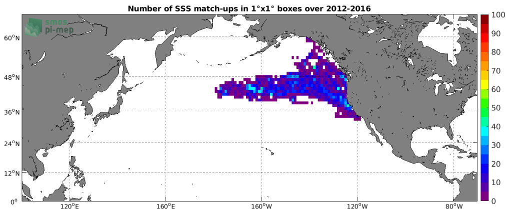
Figure 4: Number of SSS match-ups between Sea mammals SSS and the SMOS SSS L3 v2 - Monthly - 0.25 Deg (CATDS-CECOS-IFREMER) SSS product for the North Pacific Ocean Pi-MEP region over 1^\circ \times 1^\circ boxes and for the full satellite product period.
