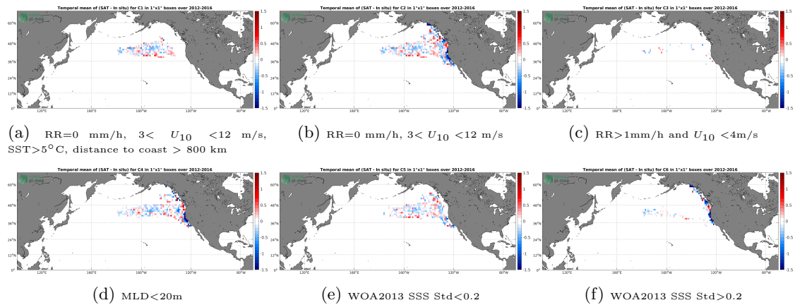
Figure 12: Temporal mean gridded over spatial boxes of size 1^{\circ}\times 1^{\circ} of \Delta\text{SSS} (SMOS SSS L3 v2 - Monthly - 0.25 Deg (CATDS-CECOS-IFREMER) - Sea mammals) for 6 different subdatasets corresponding to:RR=0 mm/h, 3 < U_{10} < 12 m/s, SST >5^{\circ}\text{C} , distance to coast > 800 km (a), RR=0 mm/h, 3 < U_{10} < 12 m/s (b), RR >1 mm/h and U_{10} < 4 m/s (c),MLD <20 m (d),WOA2013 SSS Std <0.2 (e),WOA2013 SSS Std >0.2 (f).
