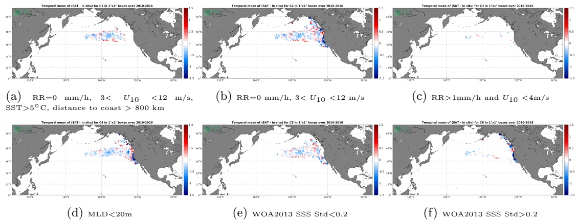
Figure 12: Temporal mean gridded over spatial boxes of size 1^{\circ}\times 1^{\circ} of \Delta\text{SSS} (SMOS L3 v2 - Monthly - 0.25 Deg (CATDS-CECOS-IFREMER) - Sea mammals) for 6 different subdatasets corresponding to: RR=0 mm/h, 3 < U_{10} < 12 m/s, SST > 5^{\circ}\text{C} , distance to coast > 800 km (a), RR=0 mm/h, 3 < U_{10} < 12 m/s (b), RR > 1\text{mm/h} and U_{10} < 4\text{m/s} (c), MLD < 20\text{m} (d), WOA2013 SSS Std < 0.2 (e), WOA2013 SSS Std > 0.2 (f).
