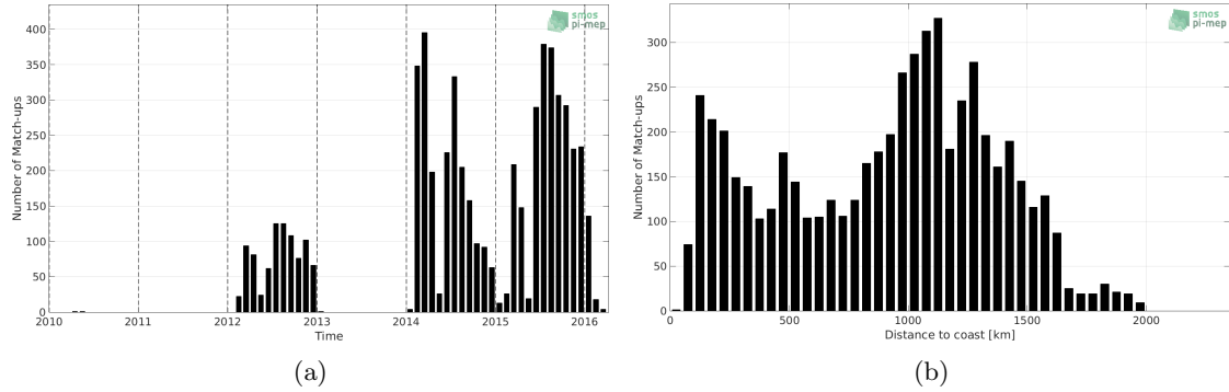
Figure 1: Number of match-ups between Sea mammals and SMOS L3 v2 - Monthly - 0.25 Deg (CATDS-CECOS-IFREMER) SSS as a function of time (a) and as function of the distance to coast (b) over the North Pacific Ocean Pi-MEP region and for the full satellite product period.
