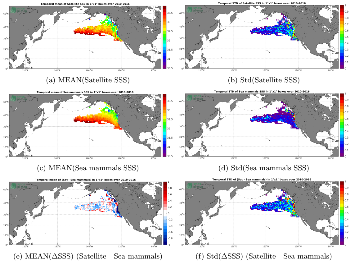
Figure 6: Temporal mean (left) and Std (right) of SSS from SMOS L3 v2 - Monthly - 0.25 Deg (CATDS-CECOS-IFREMER) (top), Sea mammals (middle), and of \Delta SSS (Satellite - Sea mammals). Only match-up pairs are used to generate these maps.
