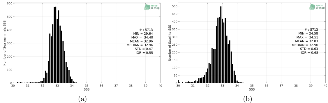
Figure 2: Histograms of SSS from Sea mammals (a) and SMOS L3 v2 - Monthly - 0.25 Deg (CATDS-CECOS-IFREMER) (b) considering all match-up pairs per bins of 0.1 over the North Pacific Ocean Pi-MEP region and for the full satellite product period.
