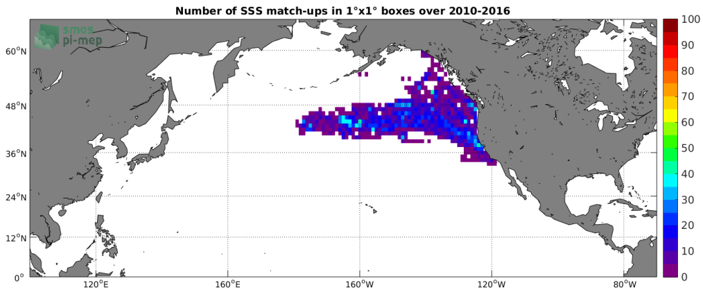
Figure 4: Number of SSS match-ups between Sea mammals SSS and the SMOS L3 v2 - Monthly - 0.25 Deg (CATDS-CECOS-IFREMER) SSS product for the North Pacific Ocean Pi-MEP region over 1°x1° boxes and for the full satellite product period.
