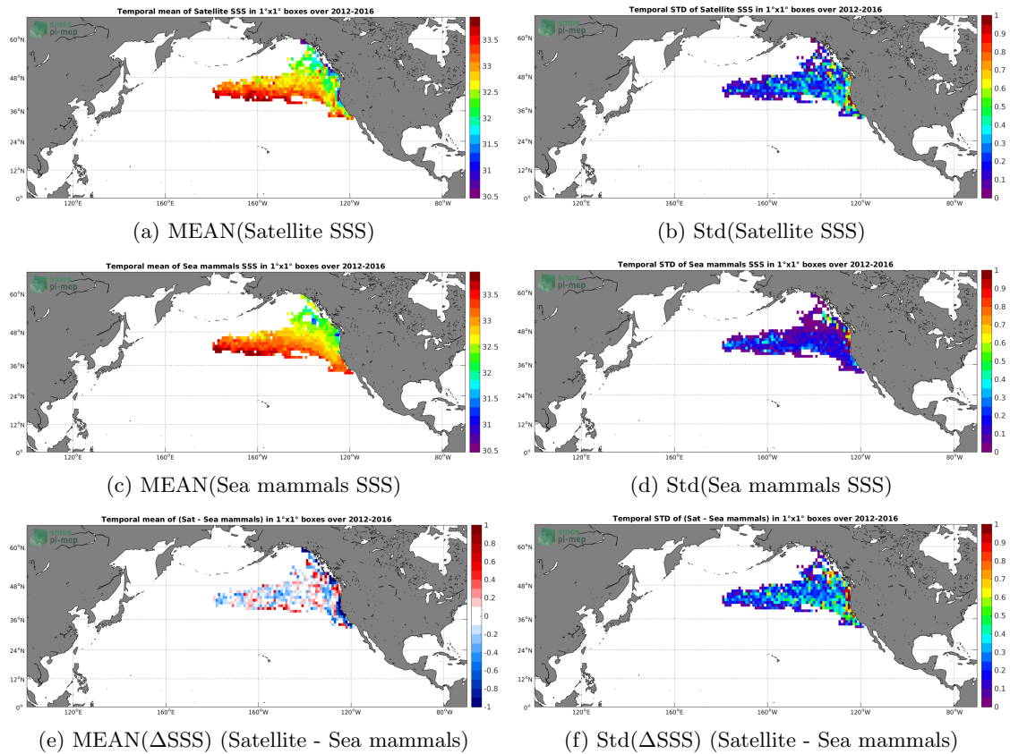
Figure 6: Temporal mean (left) and Std (right) of SSS from SMOS-L3-CATDS-IFREMER-CECOS-V2-MONTHLY-0.25DEG (top), Sea mammals (middle), and of \Delta SSS (Satellite - Sea mammals). Only match-up pairs are used to generate these maps.
