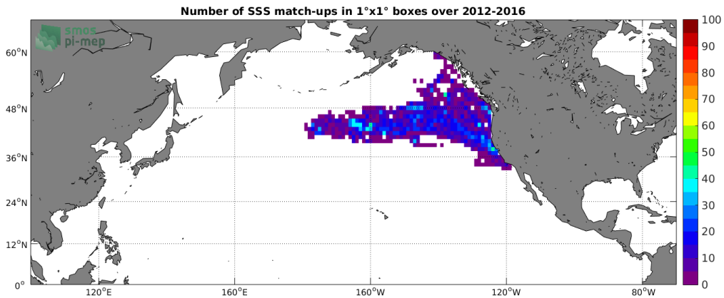
Figure 4: Number of SSS match-ups between Sea mammals SSS and the SMOS-L3-CATDS-IFREMER-CECOS-V2-MONTHLY-0.25DEG SSS product for the North Pacific Ocean Pi-MEP region over 1^\circ \times 1^\circ boxes and for the full satellite product period.
