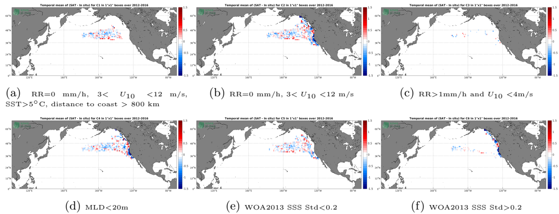
Figure 12: Temporal mean gridded over spatial boxes of size 1^\circ \times 1^\circ of \Delta SSS (SMOS-L3-CATDS-IFREMER-CECOS-V2-MONTHLY-0.25DEG - Sea mammals) for 6 different subdatasets corresponding to:RR=0 mm/h, 3 < U_{10} < 12 m/s, SST >5^\circ C, distance to coast > 800 km (a), RR=0 mm/h, 3 < U_{10} < 12 m/s (b), RR >1 mm/h and U_{10} < 4 m/s (c),MLD <20 m (d),WOA2013 SSS Std <0.2 (e),WOA2013 SSS Std >0.2 (f).
