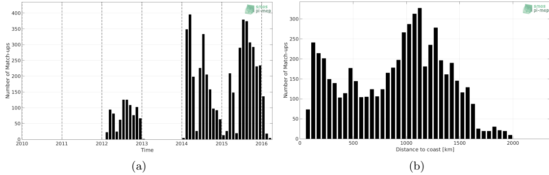
Figure 1: Number of match-ups between Sea mammals and SMOS-L3-CATDS-IFREMER-CECOS-V2-MONTHLY-0.25DEG SSS as a function of time (a) and as function of the distance to coast (b) over the North Pacific Ocean Pi-MEP region and for the full satellite product period.
