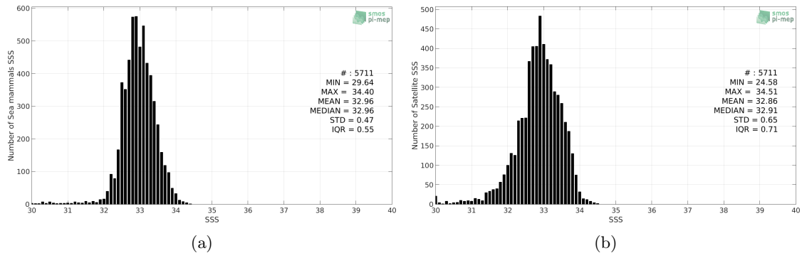
Figure 2: Histograms of SSS from Sea mammals (a) and SMOS-L3-CATDS-IFREMER-CECOS-V2-MONTHLY-0.25DEG (b) considering all match-up pairs per bins of 0.1 over the North Pacific Ocean Pi-MEP region and for the full satellite product period.
