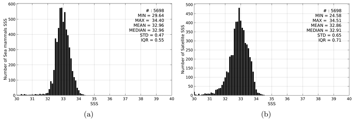
Figure 2: Histograms of SSS from Sea mammals (a) and SMOS-L3-CATDS-IFREMER-CECOS-V2-MONTHLY-0.25DEG (b) considering all match-up pairs per bins of 0.1 over the North Pacific Ocean Pi-MEP region and for the full satellite product period.
