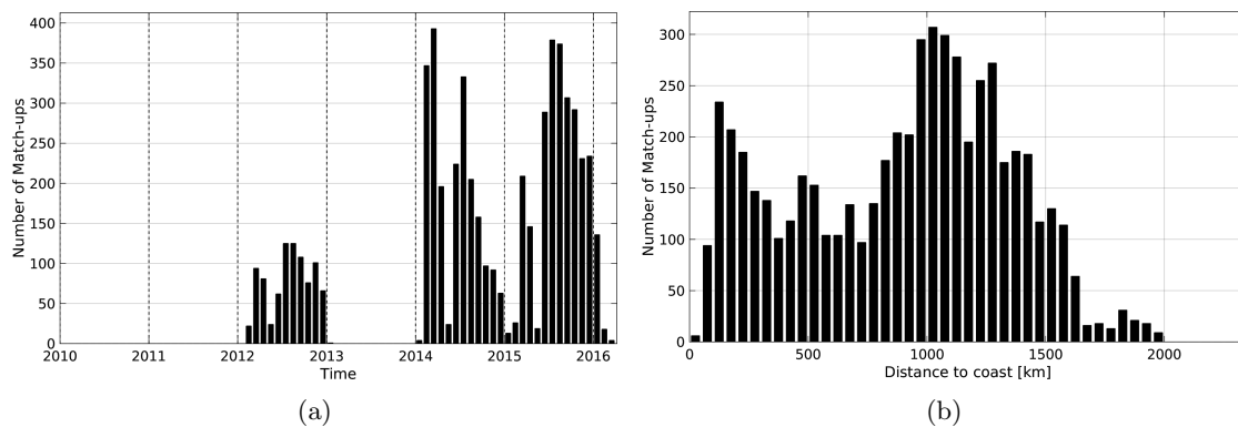
Figure 1: Number of match-ups between Sea mammals and SMOS-L3-CATDS-IFREMER-CECOS-V2-MONTHLY-0.25DEG SSS as a function of time (a) and as function of the distance to coast (b) over the North Pacific Ocean Pi-MEP region and for the full satellite product period.
