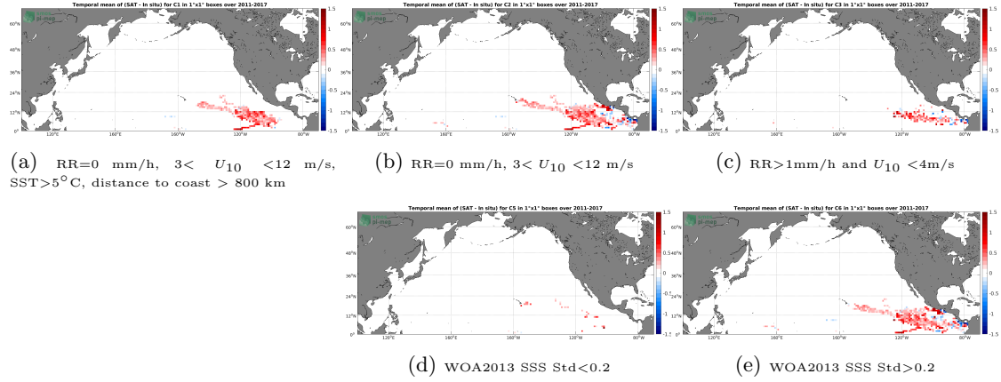
Figure 11: Temporal mean gridded over spatial boxes of size 1^{\circ}\times 1^{\circ} of \Delta\text{SSS} (SMOS SSS L3 v2 - Monthly - 0.25 Deg (CATDS-CECOS-IFREMER) - Surface drifters) for 5 different subdatasets corresponding to: RR=0 mm/h, 3 < U_{10} < 12 m/s, SST >5^{\circ}\text{C} , distance to coast > 800 km (a), RR=0 mm/h, 3 < U_{10} < 12 m/s (b), RR >1\text{mm/h} and U_{10} < 4\text{m/s} (c), WOA2013 SSS Std <0.2 (d), WOA2013 SSS Std >0.2 (e).
