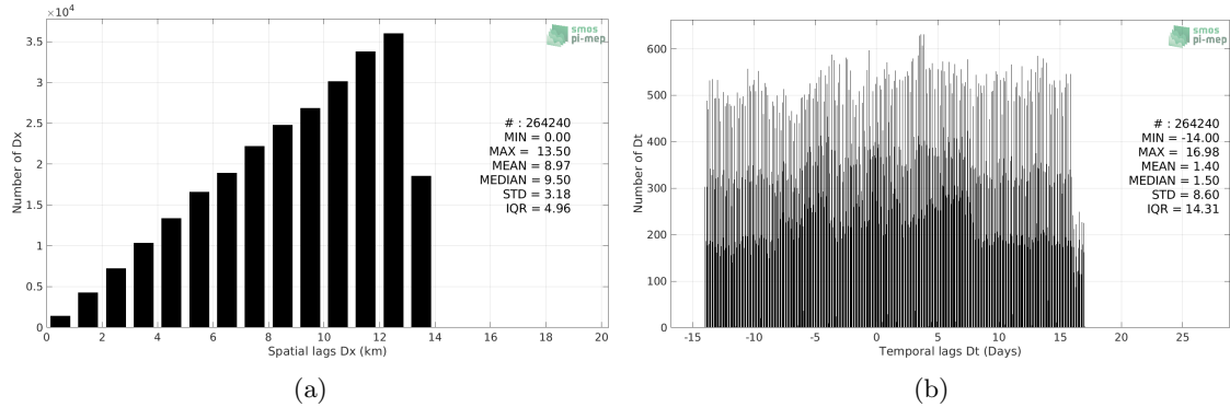
Figure 4: Histograms of the spatial (a) and temporal (b) lags between the location/time of the Surface drifters measurement and the date of the corresponding SMOS SSS L3 v2 - Monthly - 0.25 Deg (CATDS-CECOS-IFREMER) SSS pixel.
