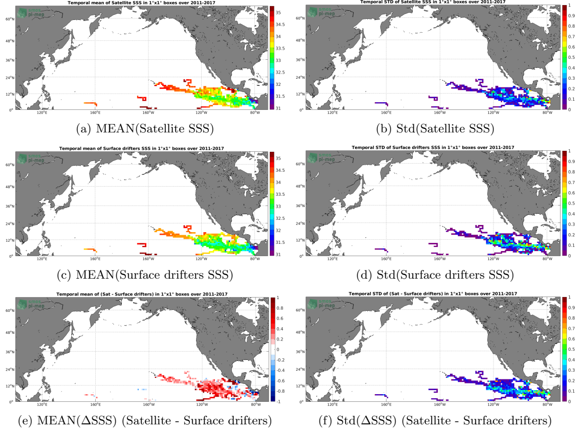
Figure 5: Temporal mean (left) and Std (right) of SSS from SMOS SSS L3 v2 - Monthly - 0.25 Deg (CATDS-CECOS-IFREMER) (top), Surface drifters (middle), and of \Delta SSS (Satellite - Surface drifters). Only match-up pairs are used to generate these maps.
