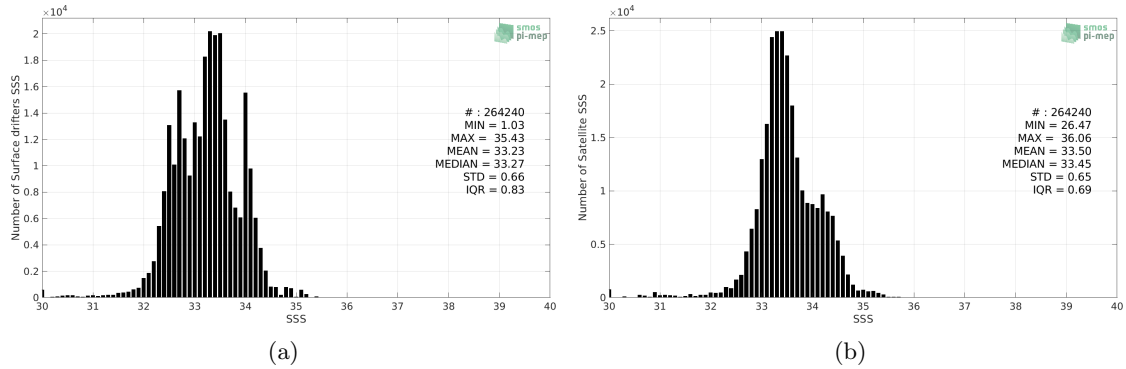
Figure 2: Histograms of SSS from Surface drifters (a) and SMOS SSS L3 v2 - Monthly - 0.25 Deg (CATDS-CECOS-IFREMER) (b) considering all match-up pairs per bins of 0.1 over the North Pacific Ocean Pi-MEP region and for the full satellite product period.
