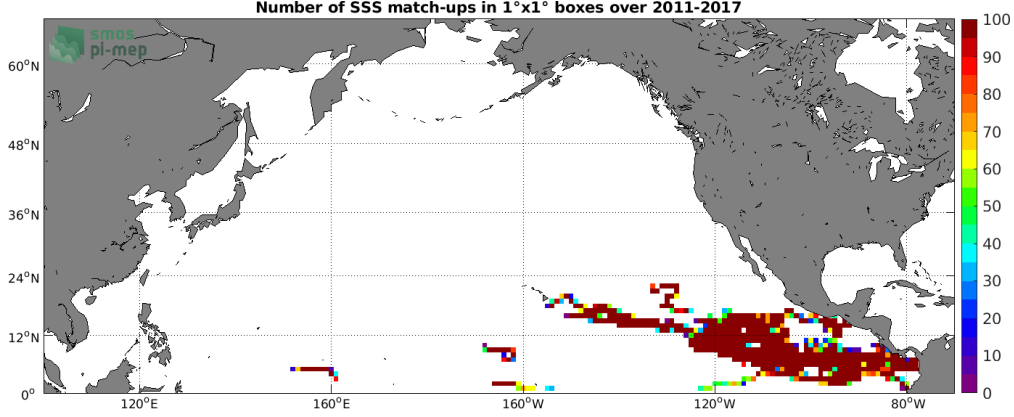
Figure 3: Number of SSS match-ups between Surface drifters SSS and the SMOS SSS L3 v2 - Monthly - 0.25 Deg (CATDS-CECOS-IFREMER) SSS product for the North Pacific Ocean Pi-MEP region over 1^\circ \times 1^\circ boxes and for the full satellite product period.
