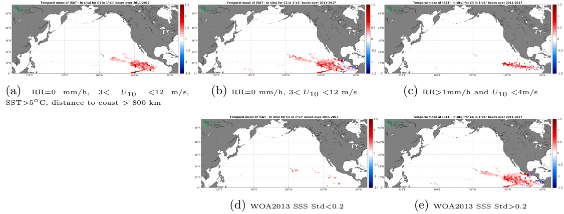
Figure 11: Temporal mean gridded over spatial boxes of size 1^{\circ}\times 1^{\circ} of \Delta\text{SSS} (SMOS L3 v2 - Monthly - 0.25 Deg (CATDS-CECOS-IFREMER) - Surface drifters) for 5 different subdatasets corresponding to: RR=0 mm/h, 3 < U_{10} < 12 m/s, SST > 5^{\circ}\text{C} , distance to coast > 800 km (a), RR=0 mm/h, 3 < U_{10} < 12 m/s (b), RR > 1 mm/h and U_{10} < 4 m/s (c), WOA2013 SSS Std < 0.2 (d), WOA2013 SSS Std > 0.2 (e).
