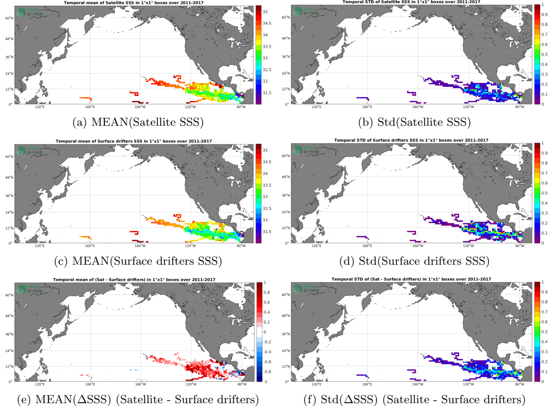
Figure 5: Temporal mean (left) and Std (right) of SSS from SMOS L3 v2 - Monthly - 0.25 Deg (CATDS-CECOS-IFREMER) (top), Surface drifters (middle), and of \Delta SSS (Satellite - Surface drifters). Only match-up pairs are used to generate these maps.
