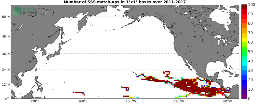
Figure 3: Number of SSS match-ups between Surface drifters SSS and the SMOS L3 v2 - Monthly - 0.25 Deg (CATDS-CECOS-IFREMER) SSS product for the North Pacific Ocean Pi-MEP region over 1^\circ \times 1^\circ boxes and for the full satellite product period.
