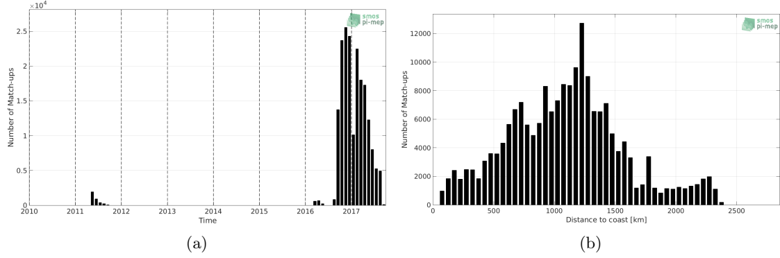
Figure 1: Number of match-ups between Surface drifters and SMOS L3 v2 - Monthly - 0.25 Deg (CATDS-CECOS-IFREMER) SSS as a function of time (a) and as function of the distance to coast (b) over the North Pacific Ocean Pi-MEP region and for the full satellite product period.
