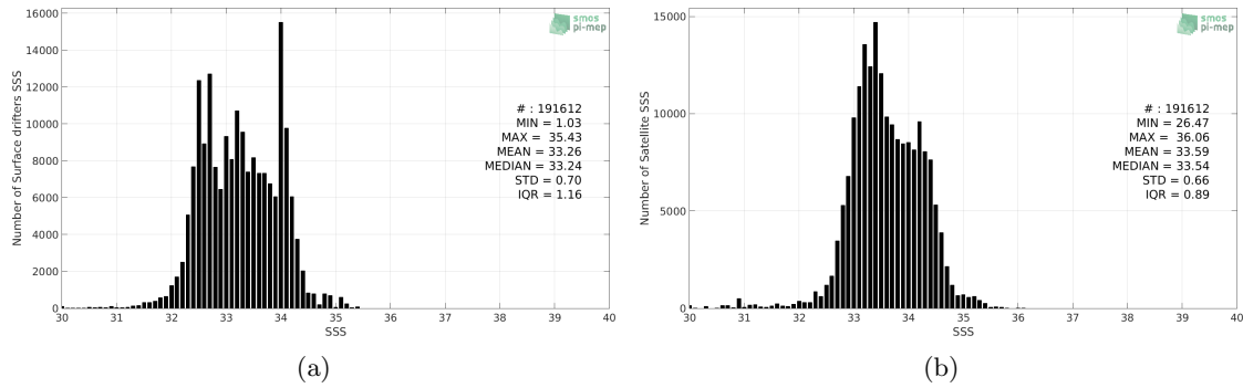
Figure 2: Histograms of SSS from Surface drifters (a) and SMOS L3 v2 - Monthly - 0.25 Deg (CATDS-CECOS-IFREMER) (b) considering all match-up pairs per bins of 0.1 over the North Pacific Ocean Pi-MEP region and for the full satellite product period.
