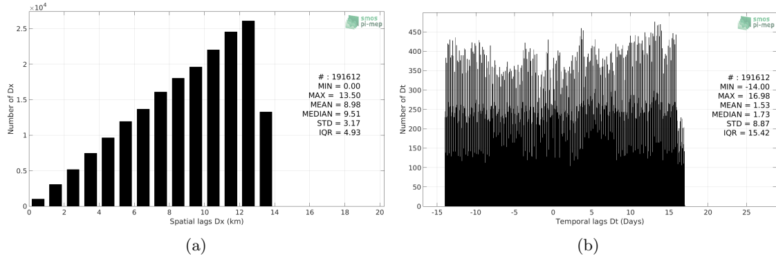
Figure 4: Histograms of the spatial (a) and temporal (b) lags between the time of the Surface drifters measurements and the date of the corresponding SMOS L3 v2 - Monthly - 0.25 Deg (CATDS-CECOS-IFREMER) SSS product.
