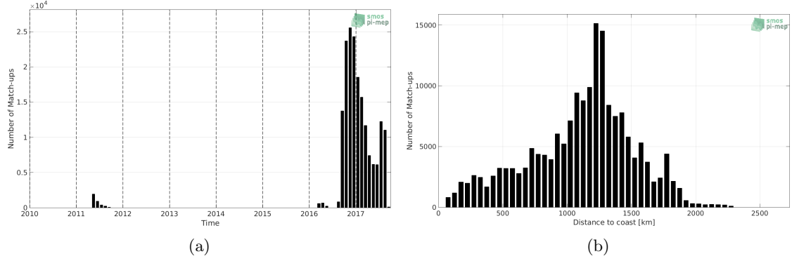
Figure 1: Number of match-ups between Surface drifters and SMOS-L3-CATDS-IFREMER-CECOS-V2-MONTHLY-0.25DEG SSS as a function of time (a) and as function of the distance to coast (b) over the North Pacific Ocean Pi-MEP region and for the full satellite product period.
