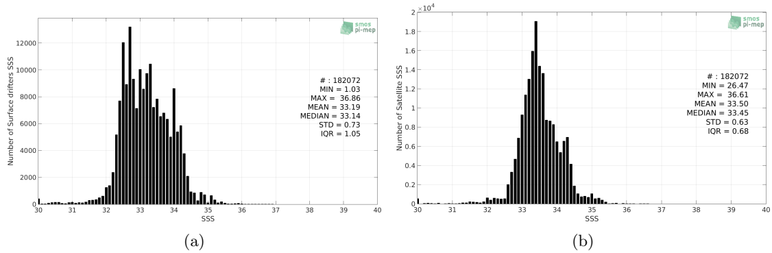
Figure 2: Histograms of SSS from Surface drifters (a) and SMOS-L3-CATDS-IFREMER-CECOS-V2-MONTHLY-0.25DEG (b) considering all match-up pairs per bins of 0.1 over the North Pacific Ocean Pi-MEP region and for the full satellite product period.
