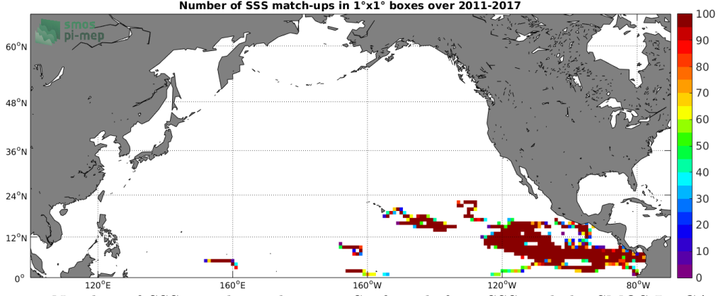
Figure 3: Number of SSS match-ups between Surface drifters SSS and the SMOS-L3-CATDS-IFREMER-CECOS-V2-MONTHLY-0.25DEG SSS product for the North Pacific Ocean Pi-MEP region over 1^\circ \times 1^\circ boxes and for the full satellite product period.
