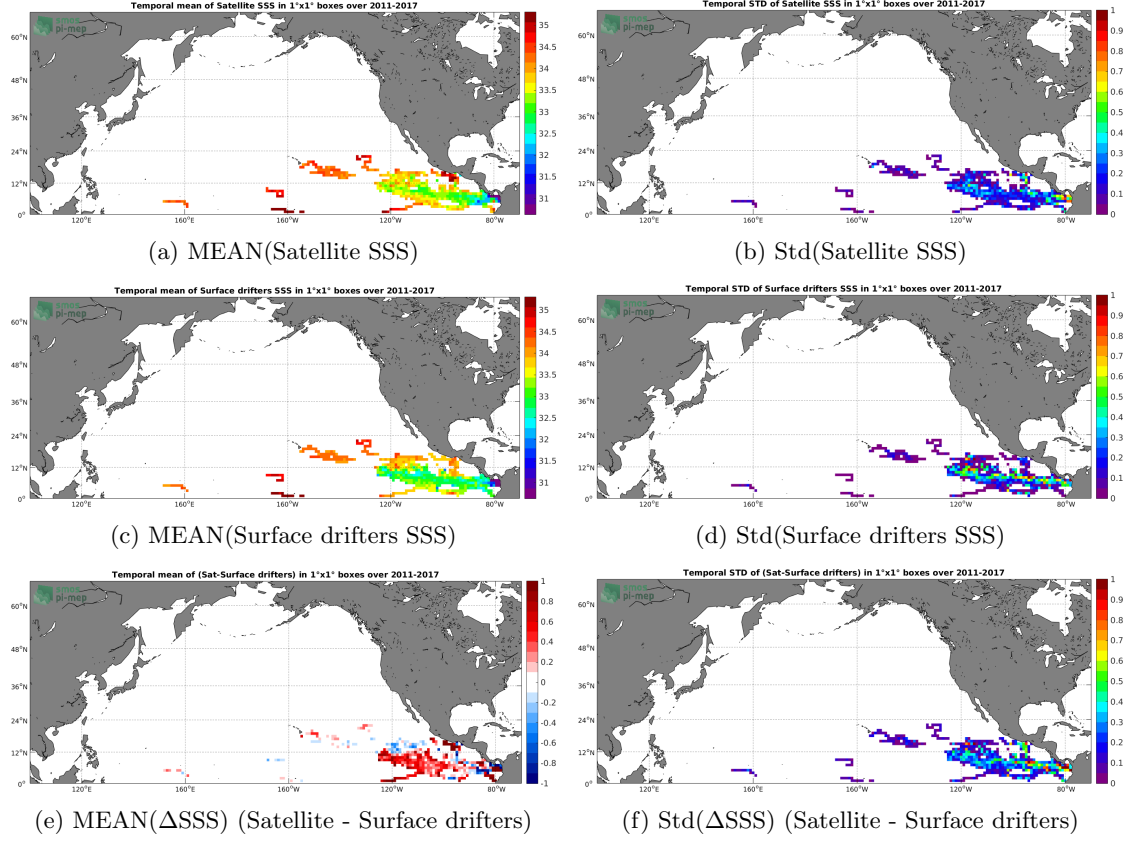
Figure 5: Temporal mean (left) and Std (right) of SSS from SMOS-L3-CATDS-IFREMER-CECOS-V2-MONTHLY-0.25DEG (top), Surface drifters (middle), and of \Delta SSS (Satellite - Surface drifters). Only match-up pairs are used to generate these maps.
