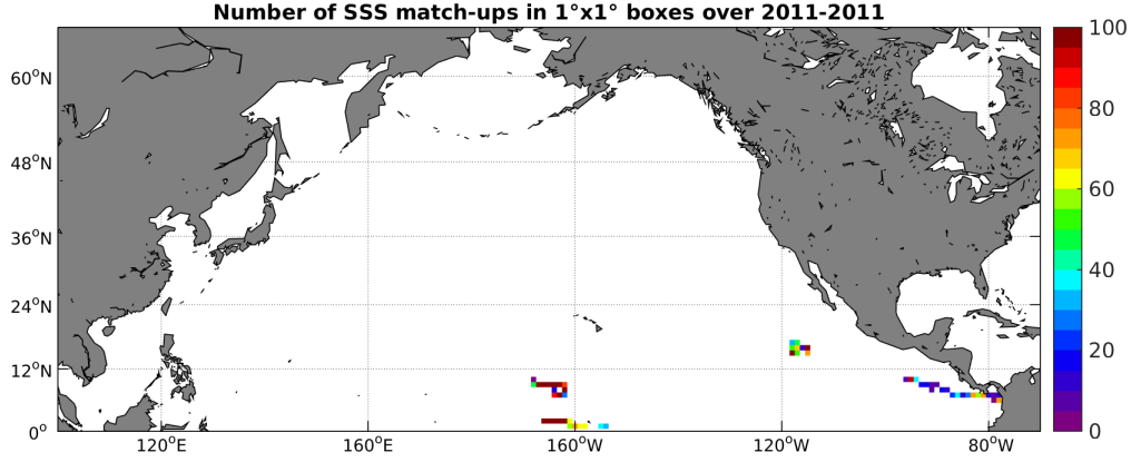
Figure 3: Number of SSS match-ups between Surface drifters SSS and the SMOS-L3-CATDS-IFREMER-CECOS-V2-MONTHLY-0.25DEG SSS product for the North Pacific Ocean Pi-MEP region over 1°x1° boxes and for the full satellite product period.
