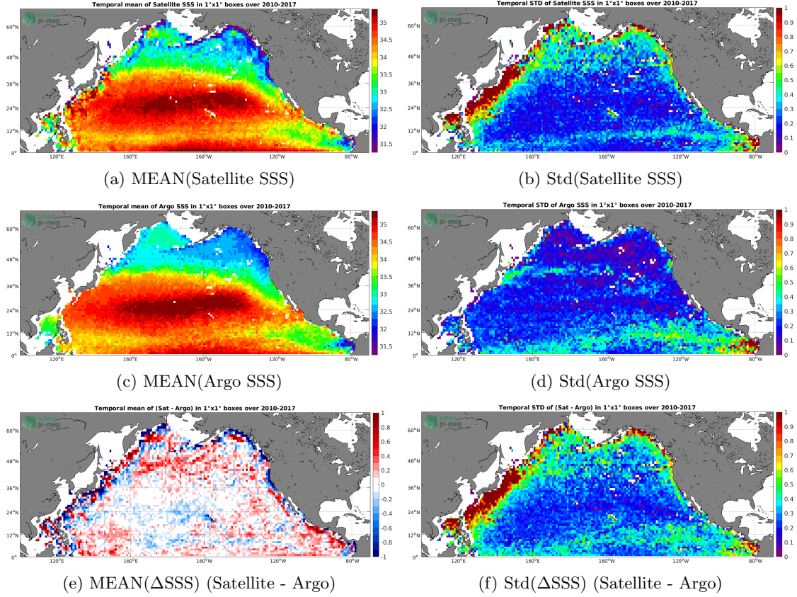
Figure 6: Temporal mean (left) and Std (right) of SSS from SMOS SSS L3 v2 - Monthly - 0.25 Deg (CATDS-CECOS-IFREMER) (top), Argo (middle), and of \Delta SSS (Satellite - Argo). Only match-up pairs are used to generate these maps.
