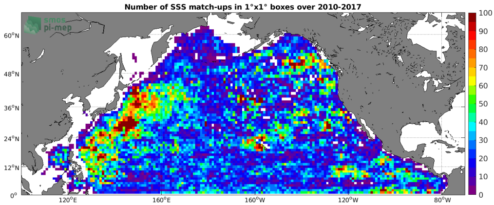
Figure 4: Number of SSS match-ups between Argo SSS and the SMOS SSS L3 v2 - Monthly - 0.25 Deg (CATDS-CECOS-IFREMER) SSS product for the North Pacific Ocean Pi-MEP region over 1^\circ \times 1^\circ boxes and for the full satellite product period.
