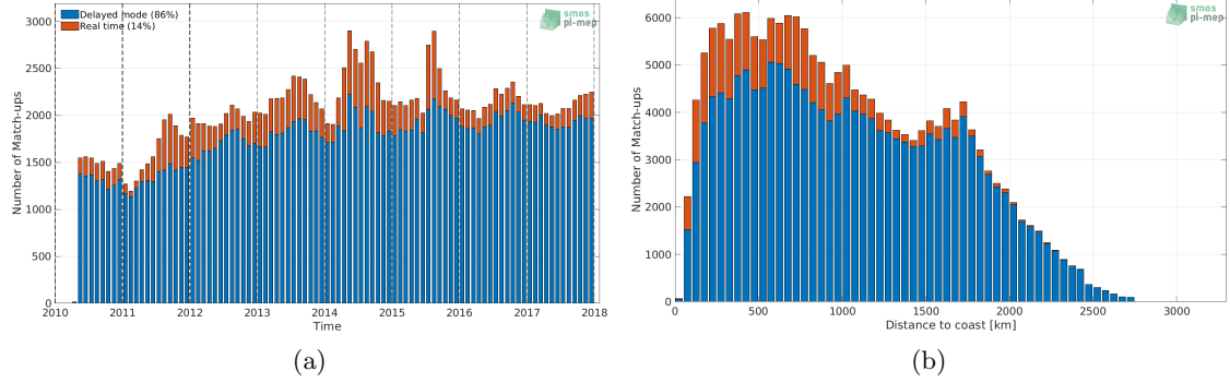
Figure 1: Number of match-ups between Argo and SMOS SSS L3 v2 - Monthly - 0.25 Deg (CATDS-CECOS-IFREMER) SSS as a function of time (a) and as function of the distance to coast (b) over the North Pacific Ocean Pi-MEP region and for the full satellite product period.
