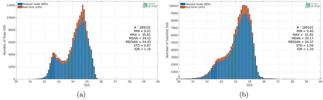
Figure 2: Histograms of SSS from Argo (a) and SMOS SSS L3 v2 - Monthly - 0.25 Deg (CATDS-CECOS-IFREMER) (b) considering all match-up pairs per bins of 0.1 over the North Pacific Ocean Pi-MEP region and for the full satellite product period.
