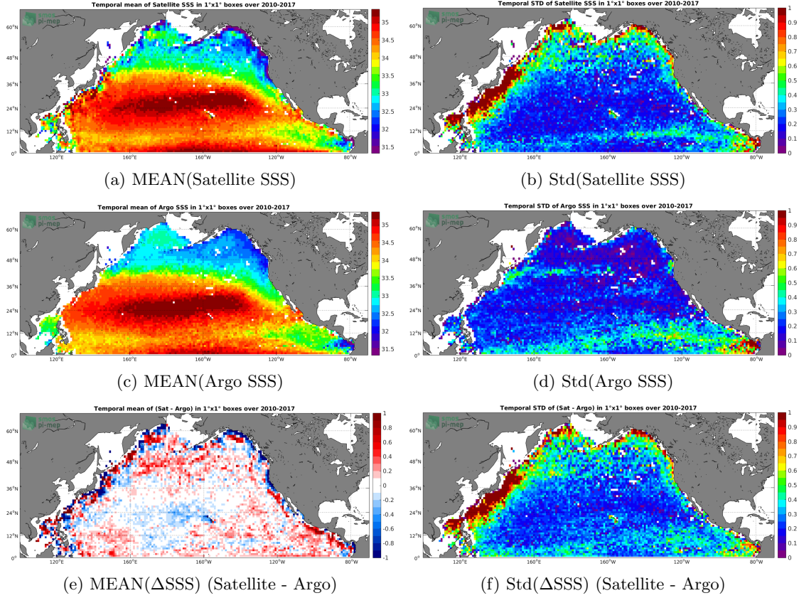
Figure 6: Temporal mean (left) and Std (right) of SSS from SMOS L3 v2 - Monthly - 0.25 Deg (CATDS-CECOS-IFREMER) (top), Argo (middle), and of \Delta SSS (Satellite - Argo). Only match-up pairs are used to generate these maps.
