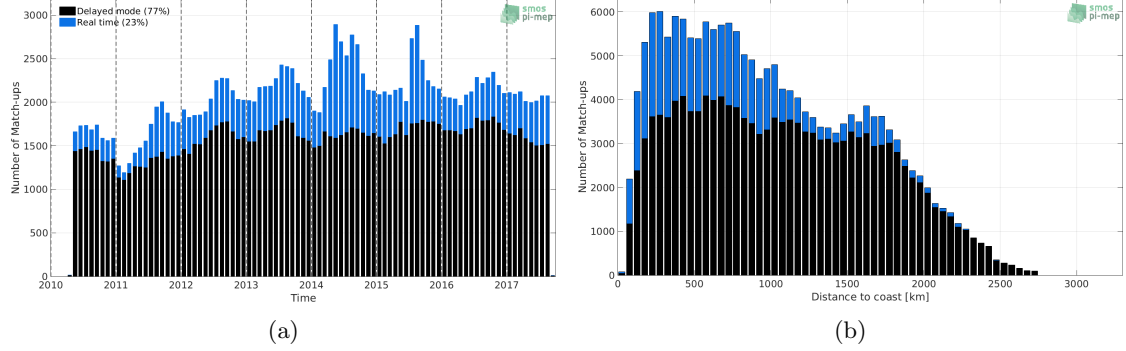
Figure 1: Number of match-ups between Argo and SMOS L3 v2 - Monthly - 0.25 Deg (CATDS-CECOS-IFREMER) SSS as a function of time (a) and as function of the distance to coast (b) over the North Pacific Ocean Pi-MEP region and for the full satellite product period.
