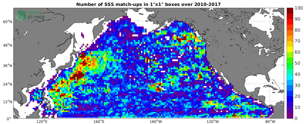
Figure 4: Number of SSS match-ups between Argo SSS and the SMOS L3 v2 - Monthly - 0.25 Deg (CATDS-CECOS-IFREMER) SSS product for the North Pacific Ocean Pi-MEP region over 1°x1° boxes and for the full satellite product period.
