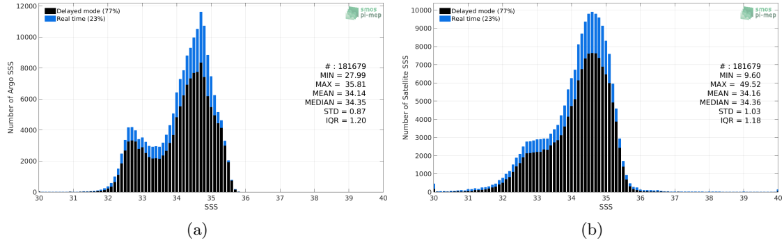
Figure 2: Histograms of SSS from Argo (a) and SMOS L3 v2 - Monthly - 0.25 Deg (CATDS-CECOS-IFREMER) (b) considering all match-up pairs per bins of 0.1 over the North Pacific Ocean Pi-MEP region and for the full satellite product period.
