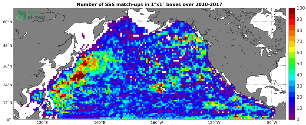
Figure 4: Number of SSS match-ups between Argo SSS and the SMOS-L3-CATDS-IFREMER-CECOS-V2-MONTHLY-0.25DEG SSS product for the North Pacific Ocean Pi-MEP region over 1^\circ \times 1^\circ boxes and for the full satellite product period.
