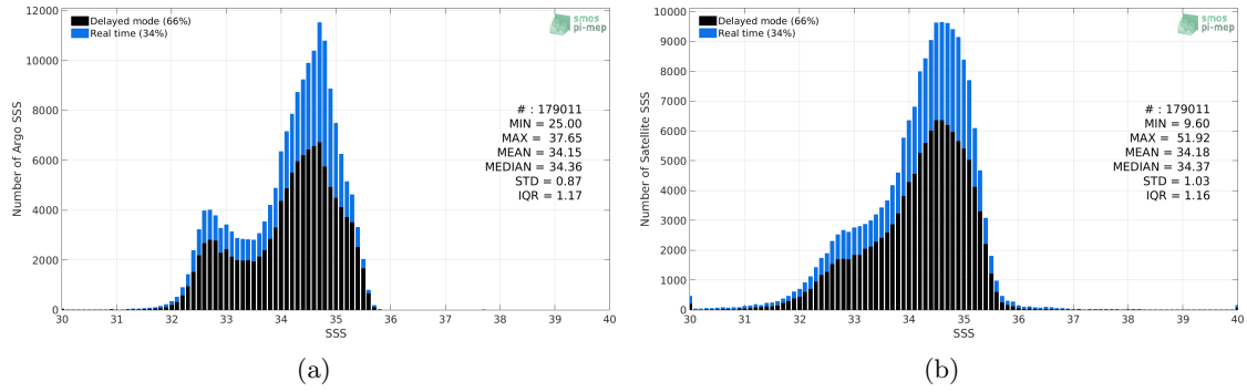
Figure 2: Histograms of SSS from Argo (a) and SMOS-L3-CATDS-IFREMER-CECOS-V2-MONTHLY-0.25DEG (b) considering all match-up pairs per bins of 0.1 over the North Pacific Ocean Pi-MEP region and for the full satellite product period.
