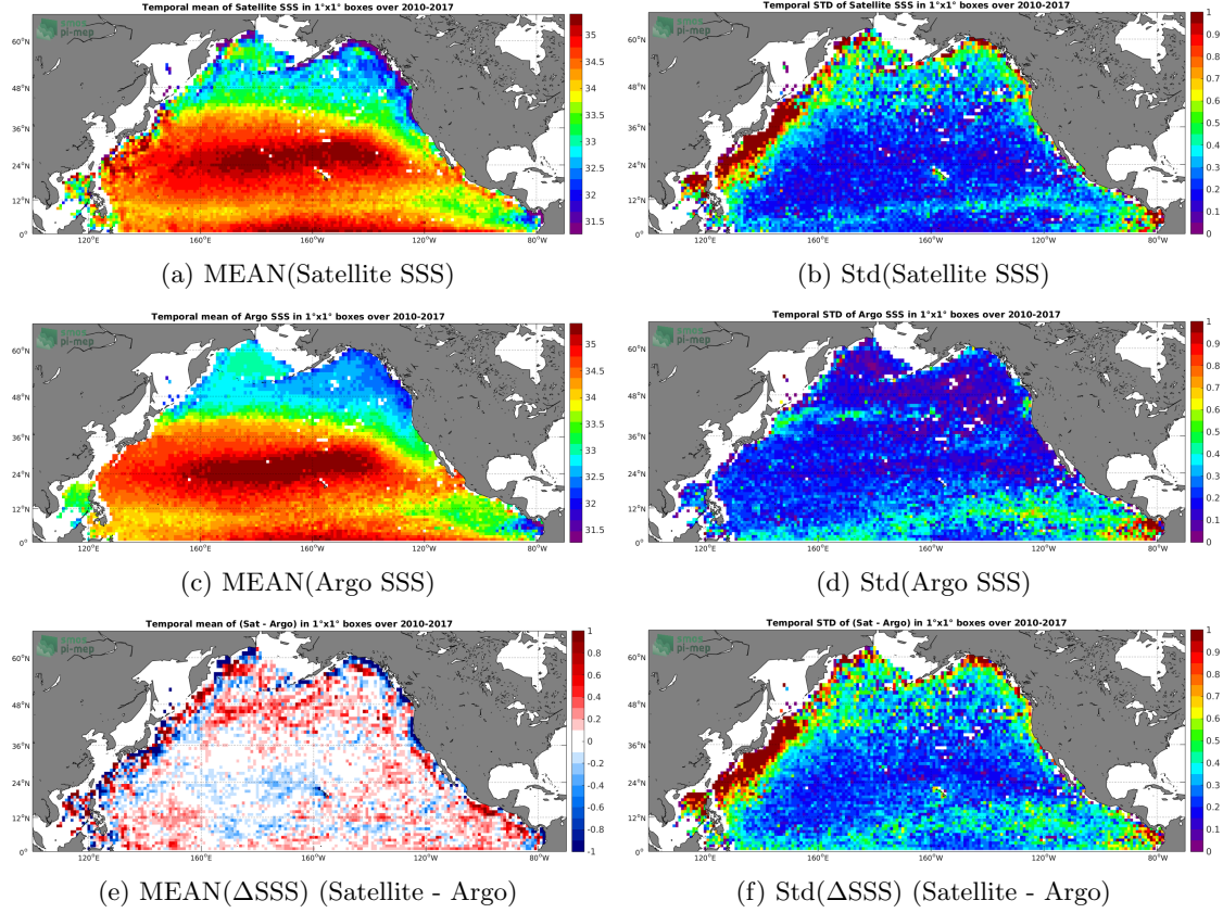
Figure 6: Temporal mean (left) and Std (right) of SSS from SMOS-L3-CATDS-IFREMER-CECOS-V2-MONTHLY-0.25DEG (top), Argo (middle), and of \Delta SSS (Satellite - Argo). Only match-up pairs are used to generate these maps.
