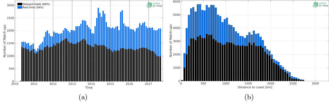
Figure 1: Number of match-ups between Argo and SMOS-L3-CATDS-IFREMER-CECOS-V2-MONTHLY-0.25DEG SSS as a function of time (a) and as function of the distance to coast (b) over the North Pacific Ocean Pi-MEP region and for the full satellite product period.
