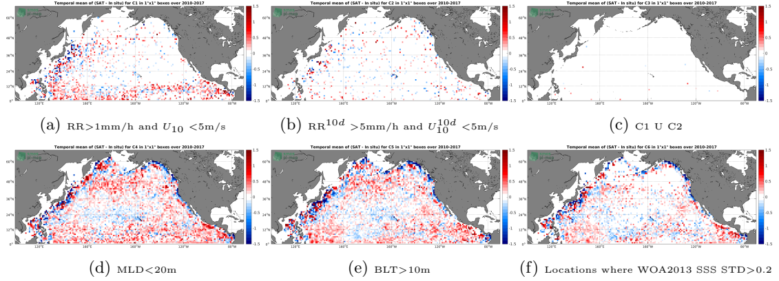
Figure 12: Temporal mean gridded over spatial boxes of size 1^\circ \times 1^\circ of \Delta\text{SSS} (SMOS-L3-CATDS-IFREMER-CECOS-V2-MONTHLY-0.25DEG - Argo) for 6 different subdatasets corresponding to: \text{RR} > 1\text{mm/h} and U_{10} < 5\text{m/s} (a), \text{RR}^{10d} > 5\text{mm/h} and U_{10}^{10d} < 5\text{m/s} (b), C1 U C2 (c), \text{MLD} < 20\text{m} (d), \text{BLT} > 10\text{m} (e), Locations where WOA2013 SSS STD > 0.2 (f).
