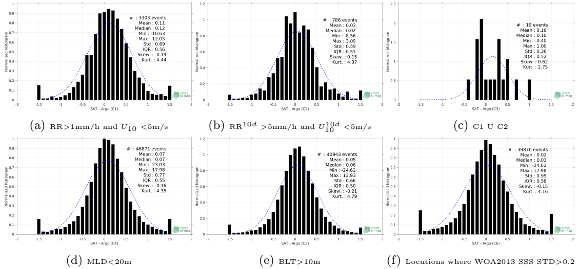
Figure 13: Normalized histogram of \Delta\text{SSS} (SMOS-L3-CATDS-IFREMER-CECOS-V2-MONTHLY-0.25DEG - Argo) for 6 different subdatasets corresponding to: \text{RR} > 1\text{mm/h} and U_{10} < 5\text{m/s} (a), \text{RR}^{10d} > 5\text{mm/h} and U_{10}^{10d} < 5\text{m/s} (b), C1 U C2 (c), \text{MLD} < 20\text{m} (d), \text{BLT} > 10\text{m} (e), Locations where WOA2013 SSS STD > 0.2 (f).
