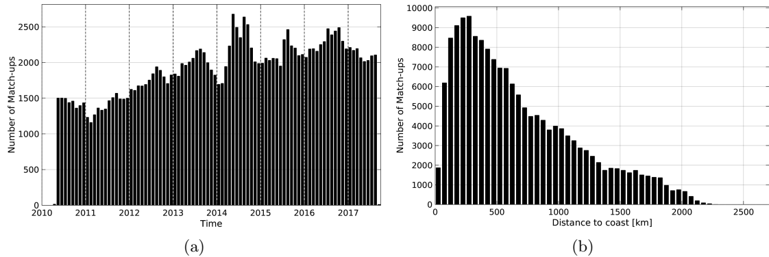
Figure 1: Number of match-ups between Argo and SMOS-L3-CATDS-IFREMER-CECOS-V2-MONTHLY-0.25DEG SSS as a function of time (a) and as function of the distance to coast (b) over the North Pacific Ocean Pi-MEP region and for the full satellite product period.
