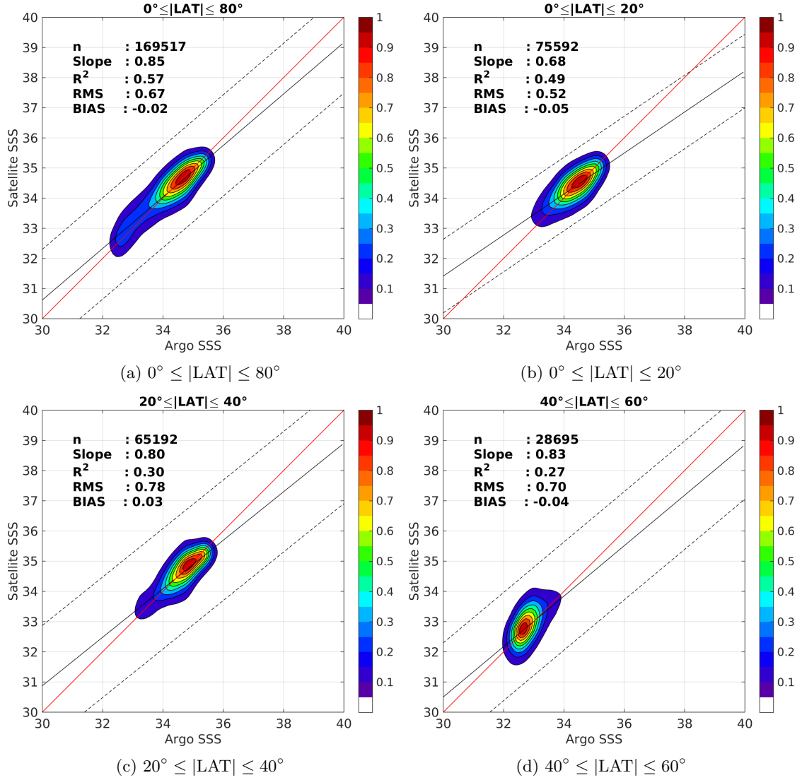
Figure 9: Contour maps of the concentration of SMOS-L3-CATDS-IFREMER-CECOS-V2-MONTHLY-0.25DEG SSS (y-axis) versus Argo SSS (x-axis) at match-up pairs for different latitude bands. For each plot, the red line shows x=y . The black thin and dashed lines indicate a linear fit through the data cloud and the \pm 95\% confidence levels, respectively. The number match-up pairs n , the slope and R^2 coefficient of the linear fit, the root mean square (RMS) and the mean bias between satellite and in situ data are indicated for each latitude band in each plots.
