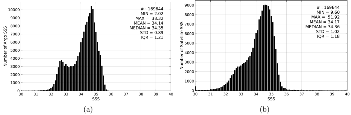
Figure 2: Histograms of SSS from Argo (a) and SMOS-L3-CATDS-IFREMER-CECOS-V2-MONTHLY-0.25DEG (b) considering all match-up pairs per bins of 0.1 over the North Pacific Ocean Pi-MEP region and for the full satellite product period.
