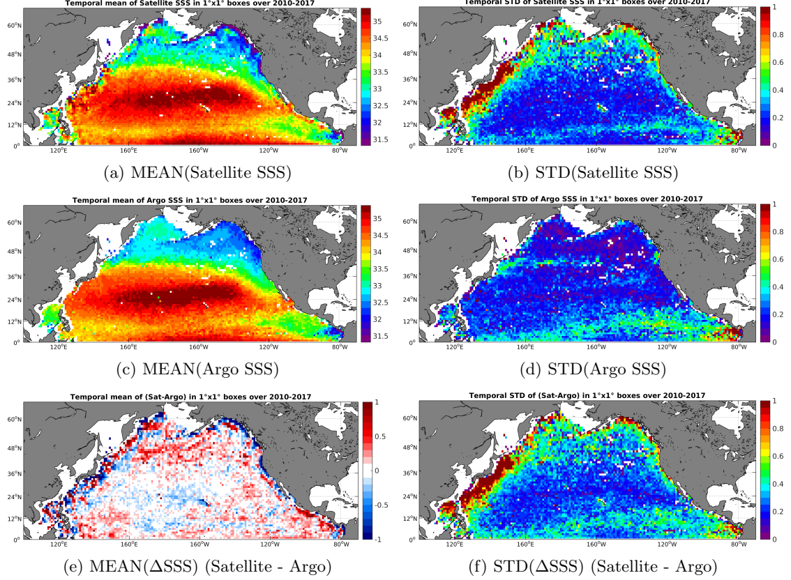
Figure 6: Temporal mean (left) and STD (right) of SSS from SMOS-L3-CATDS-IFREMER-CECOS-V2-MONTHLY-0.25DEG (top), Argo (middle), and of \Delta\text{SSS} (Satellite - Argo). Only match-up pairs are used to generate these maps.
