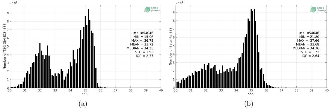
Figure 2: Histograms of SSS from TSG (SAMOS) (a) and SMOS SSS L3 v2 - Daily - 0.5 Deg (CATDS-CECOS-IFREMER) (b) considering all match-up pairs per bins of 0.1 over the North Pacific Ocean Pi-MEP region and for the full satellite product period.
