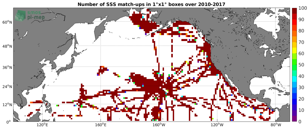
Figure 4: Number of SSS match-ups between TSG (SAMOS) SSS and the SMOS SSS L3 v2 - Daily - 0.5 Deg (CATDS-CECOS-IFREMER) SSS product for the North Pacific Ocean Pi-MEP region over 1^\circ \times 1^\circ boxes and for the full satellite product period.
