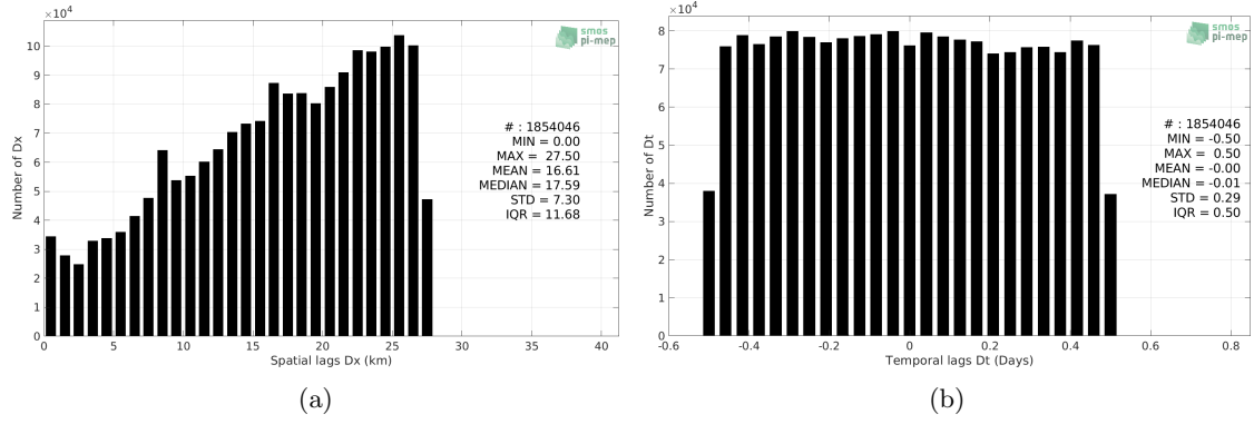
Figure 5: Histograms of the spatial (a) and temporal (b) lags between the location/time of the TSG (SAMOS) measurement and the date of the corresponding SMOS SSS L3 v2 - Daily - 0.5 Deg (CATDS-CECOS-IFREMER) SSS pixel.
