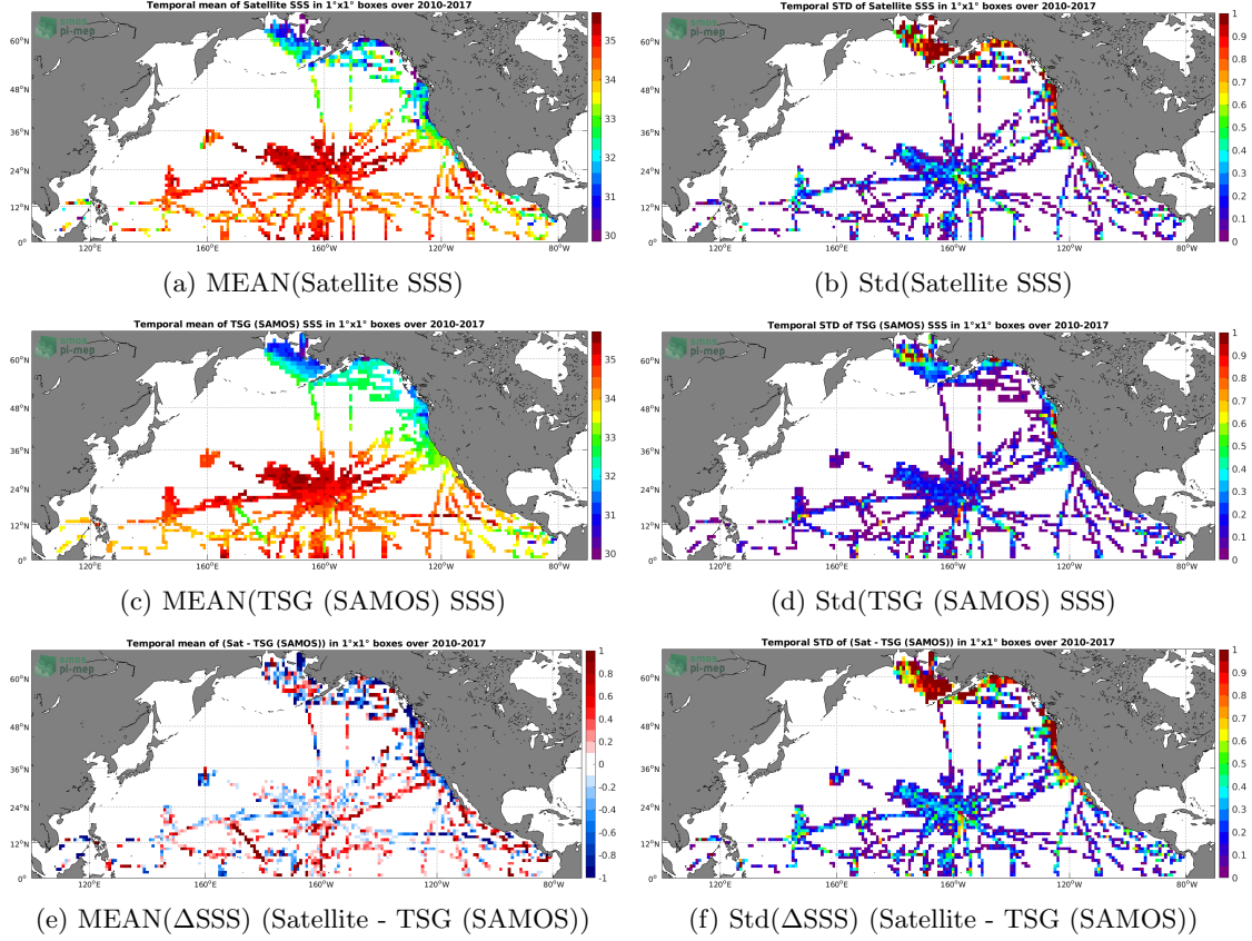
Figure 6: Temporal mean (left) and Std (right) of SSS from SMOS SSS L3 v2 - Daily - 0.5 Deg (CATDS-CECOS-IFREMER) (top), TSG (SAMOS) (middle), and of \Delta SSS (Satellite - TSG (SAMOS)). Only match-up pairs are used to generate these maps.
