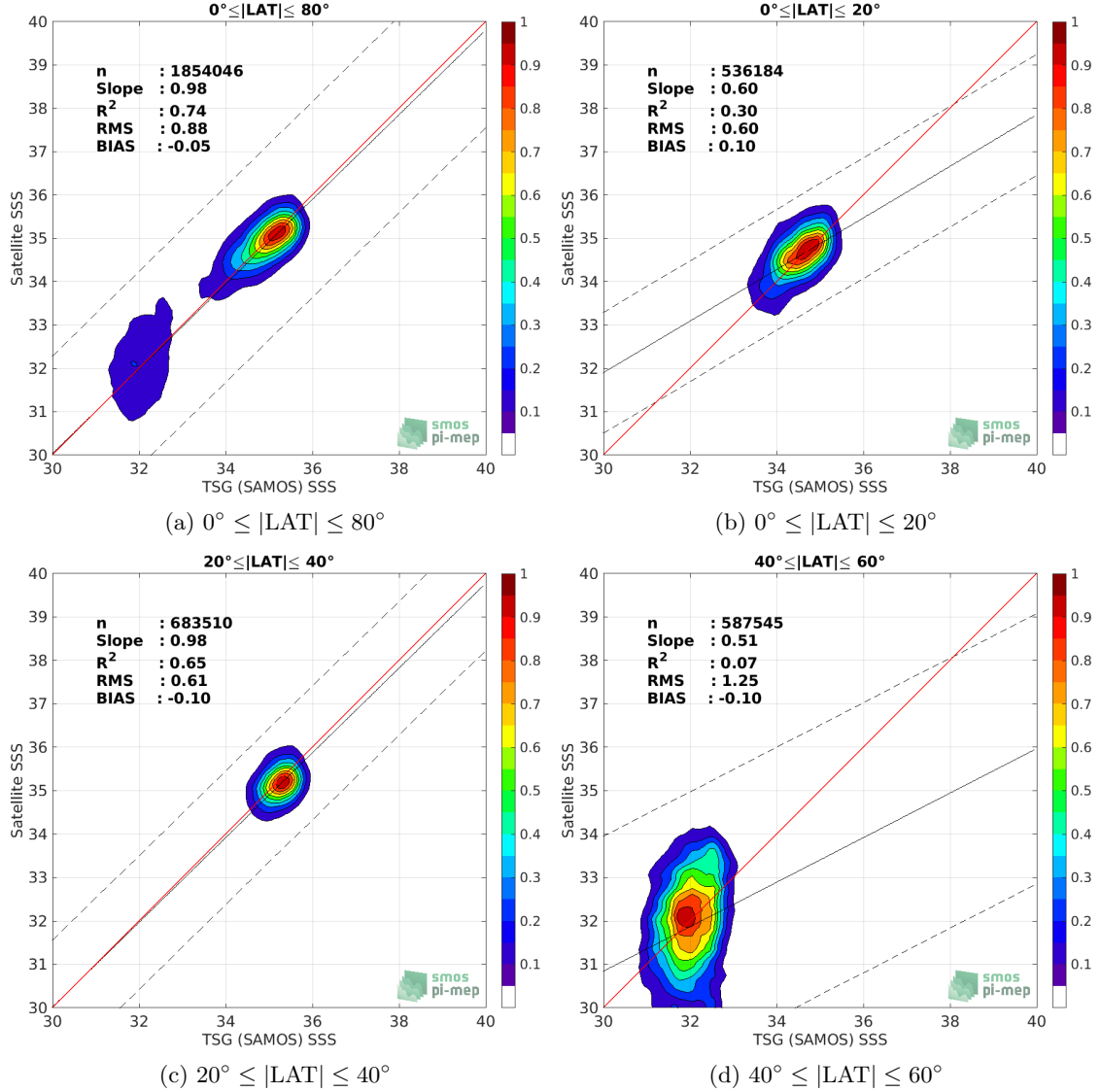
Figure 9: Contour maps of the concentration of SMOS SSS L3 v2 - Daily - 0.5 Deg (CATDS-CECOS-IFREMER) SSS (y-axis) versus TSG (SAMOS) SSS (x-axis) at match-up pairs for different latitude bands. For each plot, the red line shows x=y . The black thin and dashed lines indicate a linear fit through the data cloud and the \pm 95\% confidence levels, respectively. The number match-up pairs n , the slope and R^2 coefficient of the linear fit, the root mean square (RMS) and the mean bias between satellite and in situ data are indicated for each latitude band in each plots.
