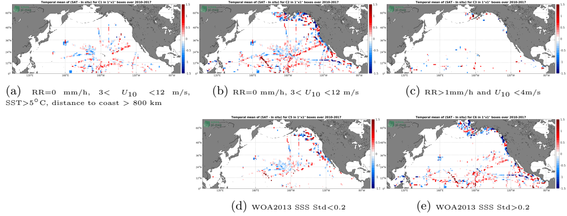
Figure 12: Temporal mean gridded over spatial boxes of size 1^\circ \times 1^\circ of \Delta SSS (SMOS SSS L3 v2 - Daily - 0.5 Deg (CATDS-CECOS-IFREMER) - TSG (SAMOS)) for 5 different subdatasets corresponding to: RR=0 mm/h, 3 < U_{10} < 12 m/s, SST > 5^\circ C , distance to coast > 800 km (a), RR=0 mm/h, 3 < U_{10} < 12 m/s (b), RR > 1 mm/h and U_{10} < 4 m/s (c), WOA2013 SSS Std < 0.2 (d), WOA2013 SSS Std > 0.2 (e).
