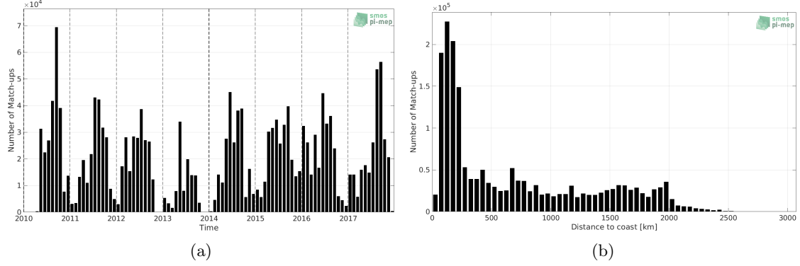
Figure 1: Number of match-ups between TSG (SAMOS) and SMOS SSS L3 v2 - Daily - 0.5 Deg (CATDS-CECOS-IFREMER) SSS as a function of time (a) and as function of the distance to coast (b) over the North Pacific Ocean Pi-MEP region and for the full satellite product period.
