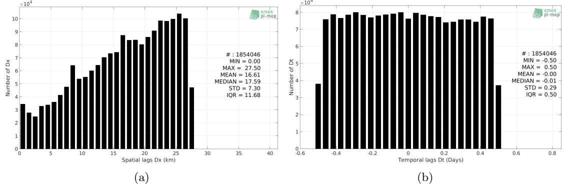
Figure 5: Histograms of the spatial (a) and temporal (b) lags between the time of the TSG (SAMOS) measurements and the date of the corresponding SMOS SSS L3 v2 - Daily - 0.5 Deg (CATDS-CECOS-IFREMER) SSS product.
