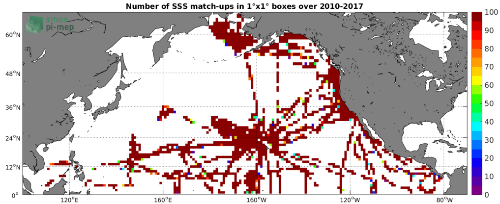
Figure 4: Number of SSS match-ups between TSG-SAMOS SSS and the SMOS L3 v2 - Daily - 0.5 Deg (CATDS-CECOS-IFREMER) SSS product for the North Pacific Ocean Pi-MEP region over 1°x1° boxes and for the full satellite product period.
