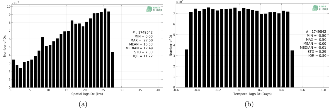
Figure 5: Histograms of the spatial (a) and temporal (b) lags between the time of the TSG-SAMOS measurements and the date of the corresponding SMOS L3 v2 - Daily - 0.5 Deg (CATDS-CECOS-IFREMER) SSS product.
