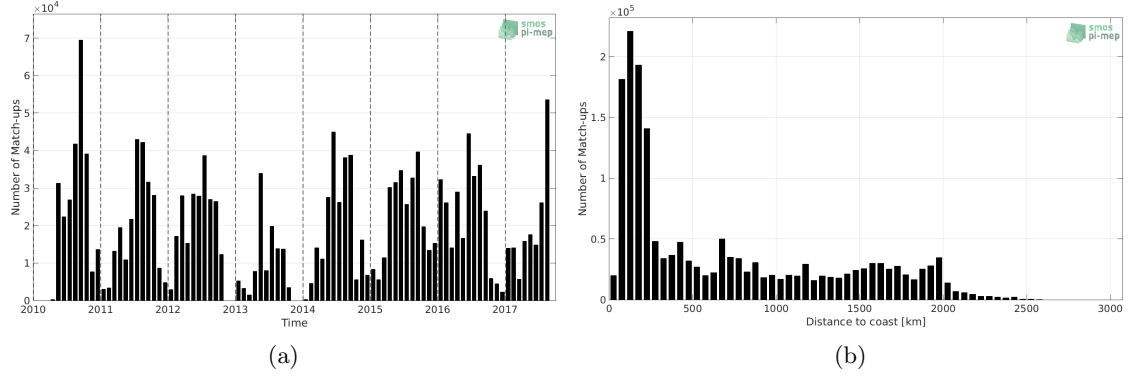
Figure 1: Number of match-ups between TSG-SAMOS and SMOS L3 v2 - Daily - 0.5 Deg (CATDS-CECOS-IFREMER) SSS as a function of time (a) and as function of the distance to coast (b) over the North Pacific Ocean Pi-MEP region and for the full satellite product period.
