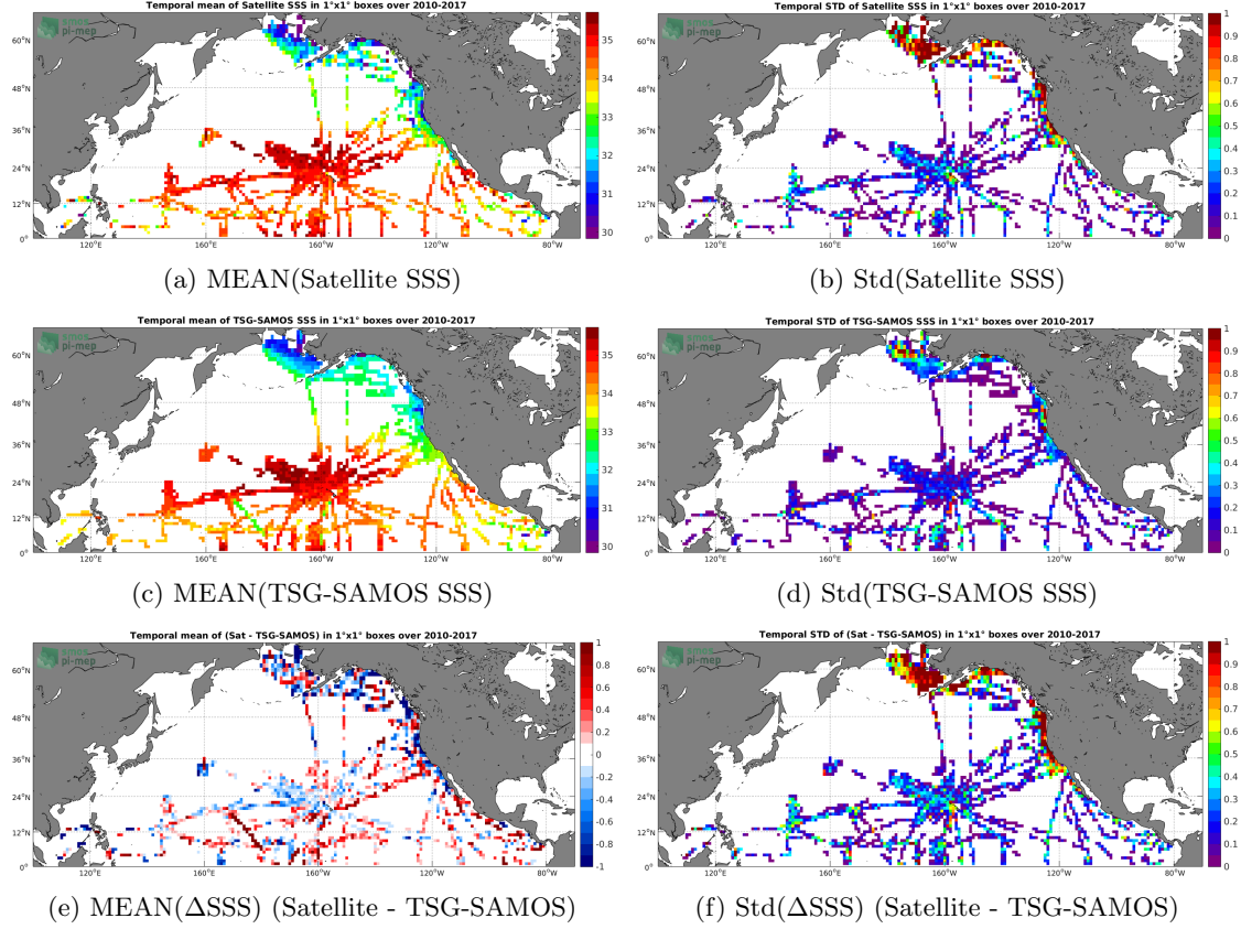
Figure 6: Temporal mean (left) and Std (right) of SSS from SMOS L3 v2 - Daily - 0.5 Deg (CATDS-CECOS-IFREMER) (top), TSG-SAMOS (middle), and of \Delta SSS (Satellite - TSG-SAMOS). Only match-up pairs are used to generate these maps.
