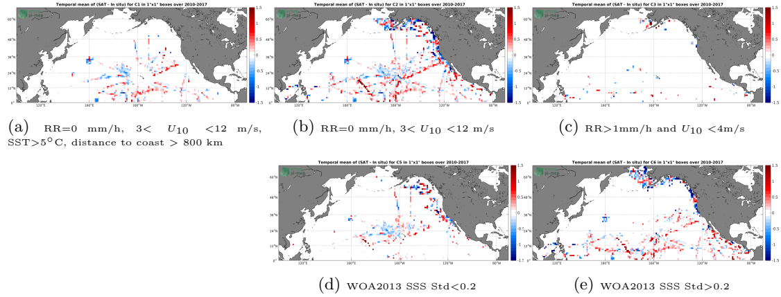
Figure 12: Temporal mean gridded over spatial boxes of size 1^\circ \times 1^\circ of \Delta SSS (SMOS L3 v2 - Daily - 0.5 Deg (CATDS-CECOS-IFREMER) - TSG-SAMOS) for 5 different subdatasets corresponding to: RR=0 mm/h, 3 < U_{10} < 12 m/s, SST > 5^\circ C , distance to coast > 800 km (a), RR=0 mm/h, 3 < U_{10} < 12 m/s (b), RR > 1 mm/h and U_{10} < 4 m/s (c), WOA2013 SSS Std < 0.2 (d), WOA2013 SSS Std > 0.2 (e).
