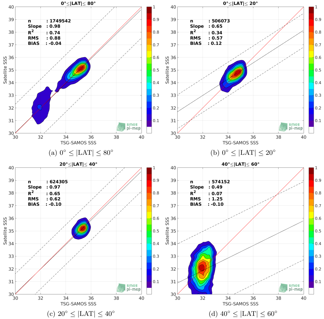
Figure 9: Contour maps of the concentration of SMOS L3 v2 - Daily - 0.5 Deg (CATDS-CECOS-IFREMER) SSS (y-axis) versus TSG-SAMOS SSS (x-axis) at match-up pairs for different latitude bands. For each plot, the red line shows x=y . The black thin and dashed lines indicate a linear fit through the data cloud and the \pm 95\% confidence levels, respectively. The number match-up pairs n , the slope and R^2 coefficient of the linear fit, the root mean square (RMS) and the mean bias between satellite and in situ data are indicated for each latitude band in each plots.
