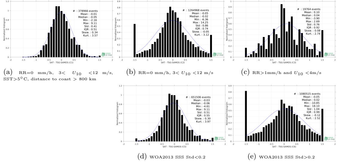
Figure 13: Normalized histogram of \Delta SSS (SMOS-L3-CATDS-CECOS-IFREMER-V2-1DAY-0.5DEG - TSG-SAMOS) for 5 different subdatasets corresponding to: RR=0 mm/h, 3 < U_{10} < 12 m/s, SST>5°C, distance to coast > 800 km (a), RR=0 mm/h, 3 < U_{10} < 12 m/s (b), RR>1mm/h and U_{10} < 4 m/s (c), WOA2013 SSS Std<0.2 (d), WOA2013 SSS Std>0.2 (e).
