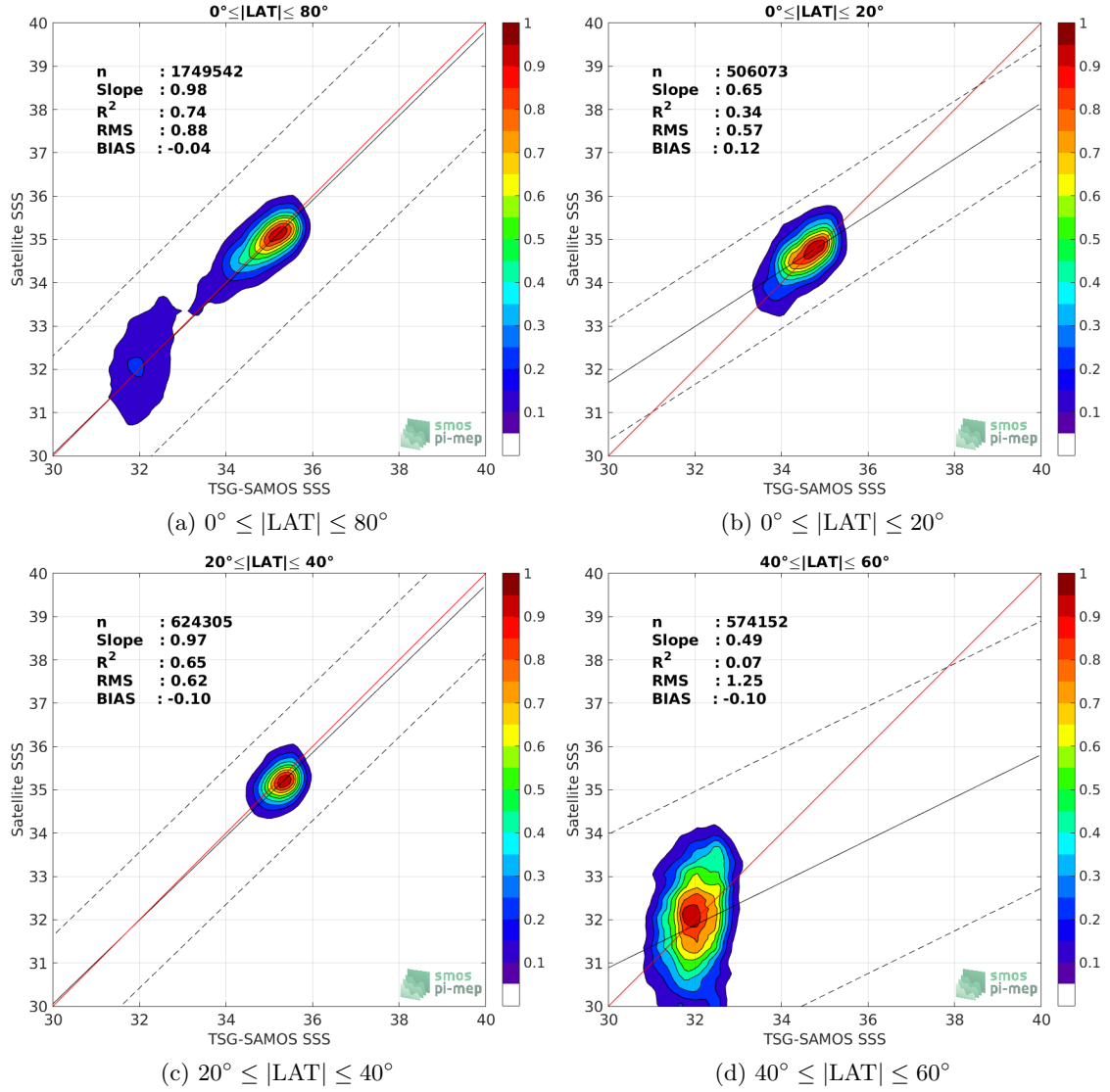
Figure 9: Contour maps of the concentration of SMOS-L3-CATDS-CECOS-IFREMER-V2-1DAY-0.5DEG SSS (y-axis) versus TSG-SAMOS SSS (x-axis) at match-up pairs for different latitude bands. For each plot, the red line shows x=y . The black thin and dashed lines indicate a linear fit through the data cloud and the \pm 95\% confidence levels, respectively. The number match-up pairs n , the slope and R^2 coefficient of the linear fit, the root mean square (RMS) and the mean bias between satellite and in situ data are indicated for each latitude band in each plots.
