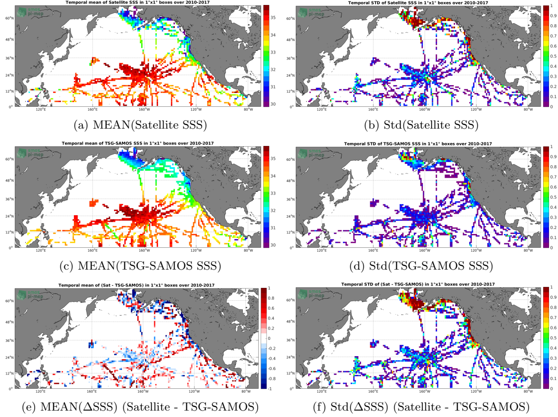
Figure 6: Temporal mean (left) and Std (right) of SSS from SMOS-L3-CATDS-CECOS-IFREMER-V2-1DAY-0.5DEG (top), TSG-SAMOS (middle), and of \Delta SSS (Satellite - TSG-SAMOS). Only match-up pairs are used to generate these maps.
