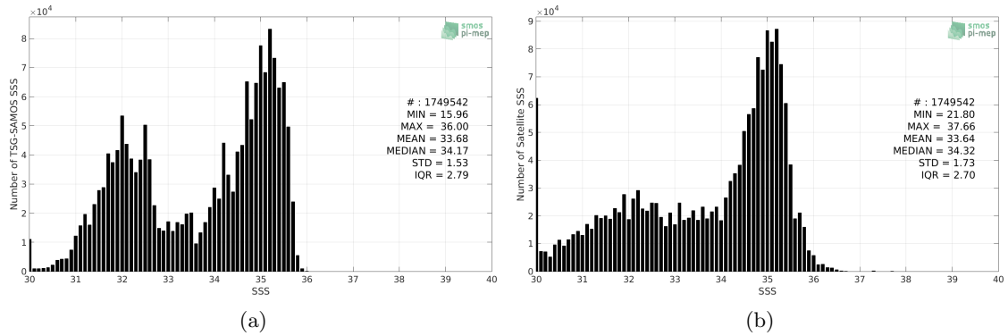
Figure 2: Histograms of SSS from TSG-SAMOS (a) and SMOS-L3-CATDS-CECOS-IFREMER-V2-1DAY-0.5DEG (b) considering all match-up pairs per bins of 0.1 over the North Pacific Ocean Pi-MEP region and for the full satellite product period.
