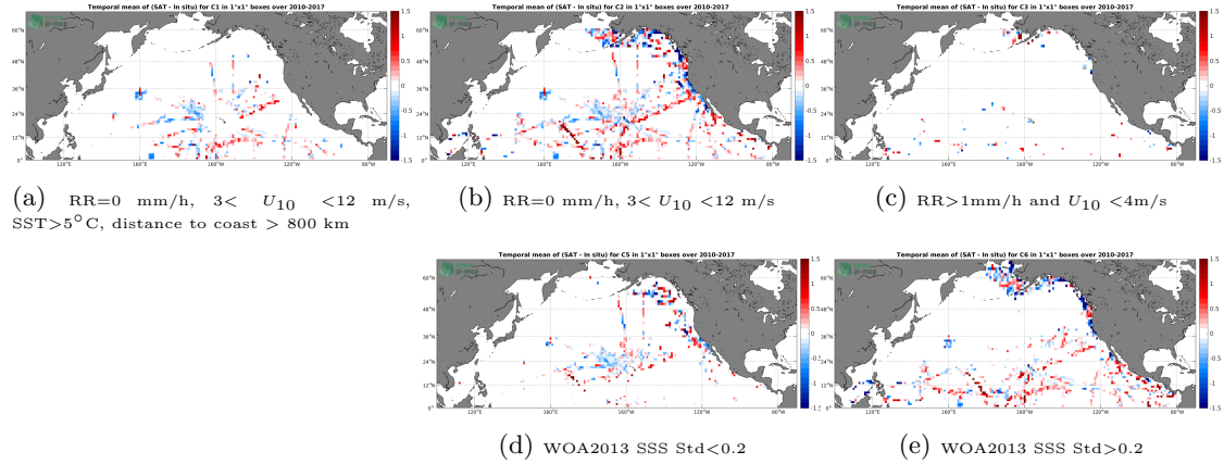
Figure 12: Temporal mean gridded over spatial boxes of size 1^\circ \times 1^\circ of \Delta SSS (SMOS-L3-CATDS-CECOS-IFREMER-V2-1DAY-0.5DEG - TSG-SAMOS) for 5 different subdatasets corresponding to: RR=0 mm/h, 3 < U_{10} < 12 m/s, SST > 5^\circ C , distance to coast > 800 km (a), RR=0 mm/h, 3 < U_{10} < 12 m/s (b), RR > 1 mm/h and U_{10} < 4 m/s (c), WOA2013 SSS Std < 0.2 (d), WOA2013 SSS Std > 0.2 (e).
