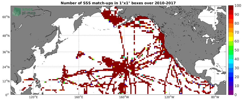
Figure 4: Number of SSS match-ups between TSG-SAMOS SSS and the SMOS-L3-CATDS-CECOS-IFREMER-V2-1DAY-0.5DEG SSS product for the North Pacific Ocean Pi-MEP region over 1°x1° boxes and for the full satellite product period.
