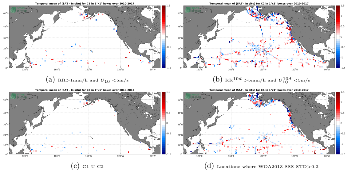
Figure 12: Temporal mean gridded over spatial boxes of size 1^\circ \times 1^\circ of \Delta SSS (SMOS-L3-CATDS-CECOS-IFREMER-V2-1DAY-0.5DEG - TSG-SAMOS) for 4 different subdatasets corresponding to: RR > 1mm/h and U_{10} < 5\text{m/s} (a), RR^{10d} > 5\text{mm/h} and U_{10}^{10d} < 5\text{m/s} (b), C1 U C2 (c), Locations where WOA2013 SSS STD > 0.2 (d).
