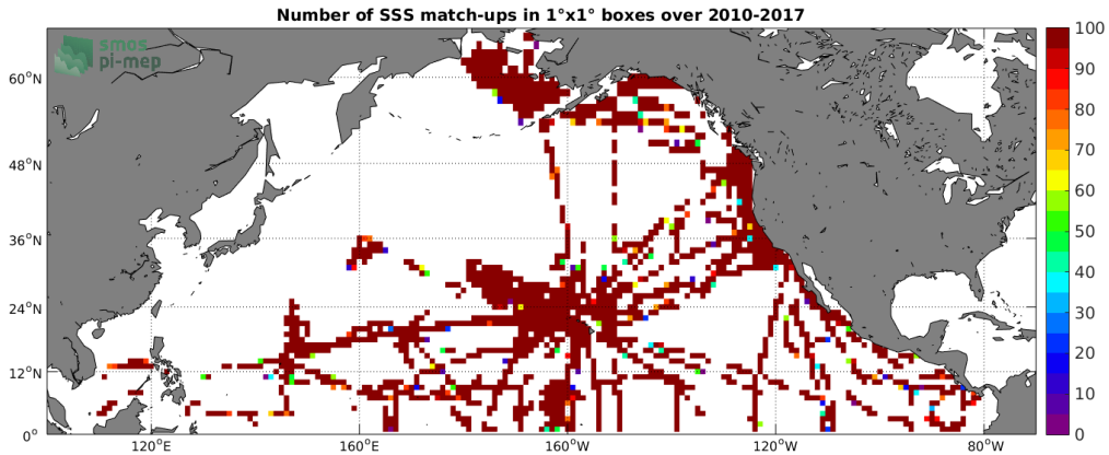
Figure 4: Number of SSS match-ups between TSG-SAMOS SSS and the SMOS-L3-CATDS-CECOS-IFREMER-V2-1DAY-0.5DEG SSS product for the North Pacific Ocean Pi-MEP region over 1^\circ \times 1^\circ boxes and for the full satellite product period.
