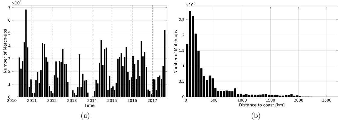
Figure 1: Number of match-ups between TSG-SAMOS and SMOS-L3-CATDS-CECOS-IFREMER-V2-1DAY-0.5DEG SSS as a function of time (a) and as function of the distance to coast (b) over the North Pacific Ocean Pi-MEP region and for the full satellite product period.
