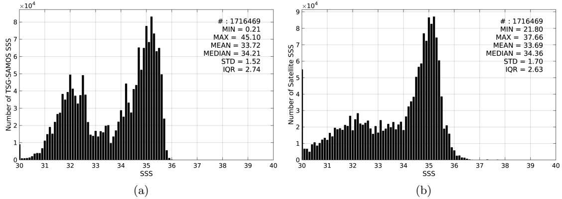
Figure 2: Histograms of SSS from TSG-SAMOS (a) and SMOS-L3-CATDS-CECOS-IFREMER-V2-1DAY-0.5DEG (b) considering all match-up pairs per bins of 0.1 over the North Pacific Ocean Pi-MEP region and for the full satellite product period.
