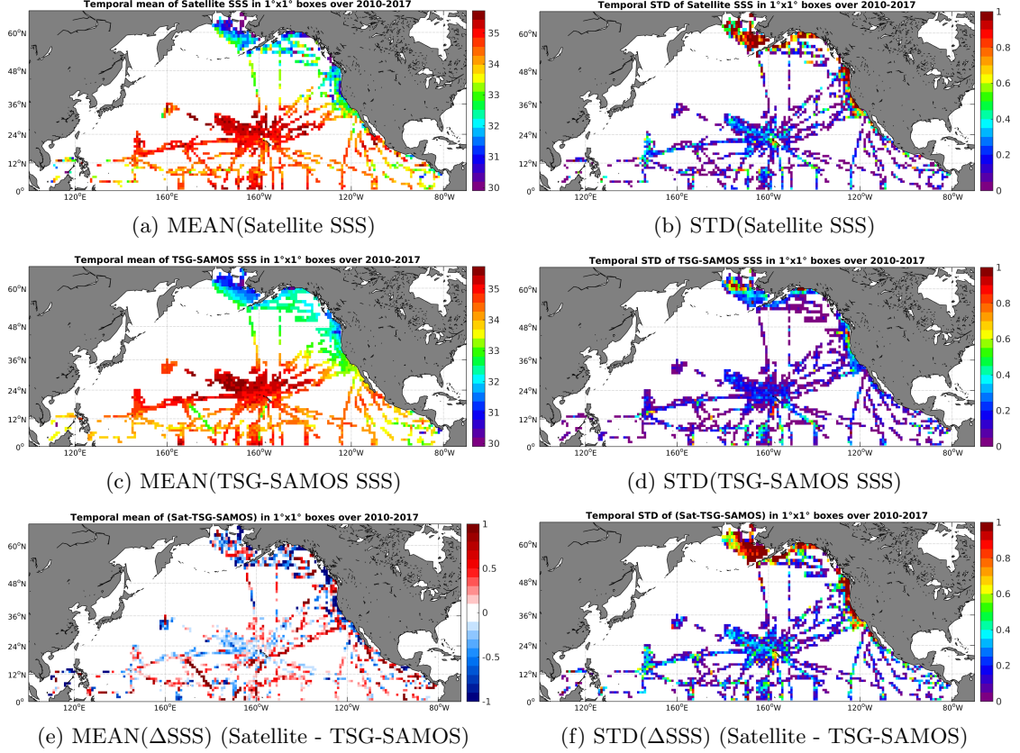
Figure 6: Temporal mean (left) and STD (right) of SSS from SMOS-L3-CATDS-CECOS-IFREMER-V2-1DAY-0.5deg (top), TSG-SAMOS (middle), and of \Delta\text{SSS} (Satellite - TSG-SAMOS). Only match-up pairs are used to generate these maps.
