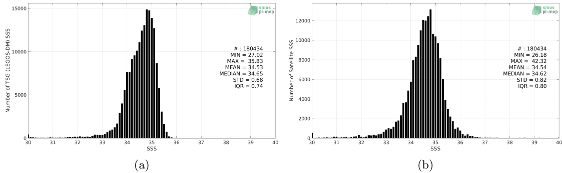
Figure 2: Histograms of SSS from TSG (LEGOS-DM) (a) and SMOS SSS L3 v2 - Daily - 0.5 Deg (CATDS-CECOS-IFREMER) (b) considering all match-up pairs per bins of 0.1 over the North Pacific Ocean Pi-MEP region and for the full satellite product period.
