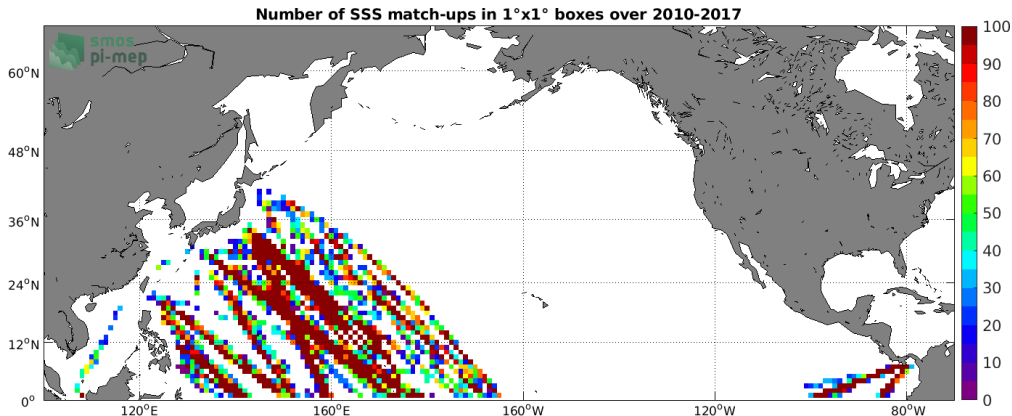
Figure 4: Number of SSS match-ups between TSG (LEGOS-DM) SSS and the SMOS SSS L3 v2 - Daily - 0.5 Deg (CATDS-CECOS-IFREMER) SSS product for the North Pacific Ocean Pi-MEP region over 1^\circ \times 1^\circ boxes and for the full satellite product period.
