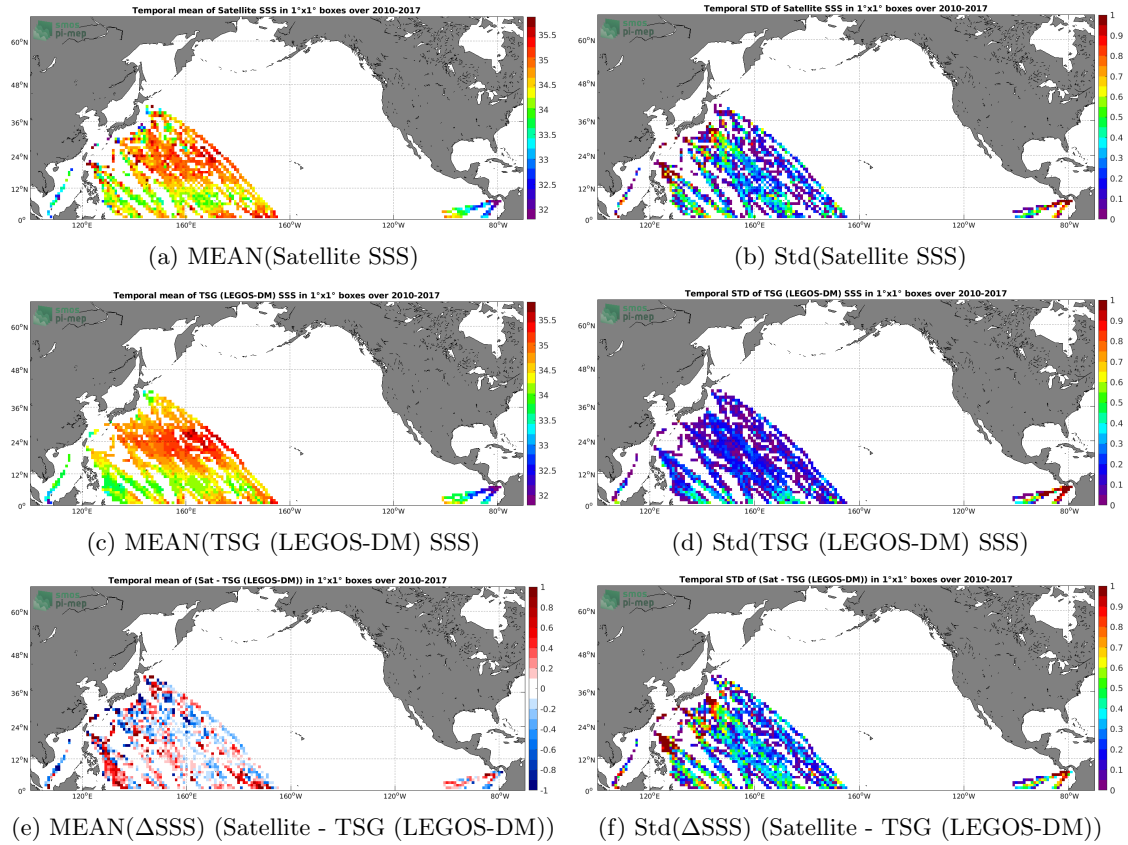
Figure 6: Temporal mean (left) and Std (right) of SSS from SMOS SSS L3 v2 - Daily - 0.5 Deg (CATDS-CECOS-IFREMER) (top), TSG (LEGOS-DM) (middle), and of \Delta SSS (Satellite - TSG (LEGOS-DM)). Only match-up pairs are used to generate these maps.
