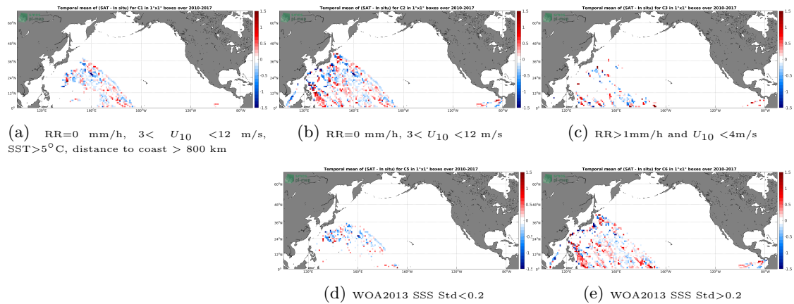
Figure 12: Temporal mean gridded over spatial boxes of size 1^\circ \times 1^\circ of \Delta SSS (SMOS SSS L3 v2 - Daily - 0.5 Deg (CATDS-CECOS-IFREMER) - TSG (LEGOS-DM)) for 5 different subdatasets corresponding to:RR=0 mm/h, 3 < U_{10} < 12 m/s, SST >5^\circ\text{C} , distance to coast > 800 km (a), RR=0 mm/h, 3 < U_{10} < 12 m/s (b), RR >1 mm/h and U_{10} < 4 m/s (c), WOA2013 SSS Std <0.2 (d), WOA2013 SSS Std >0.2 (e).
