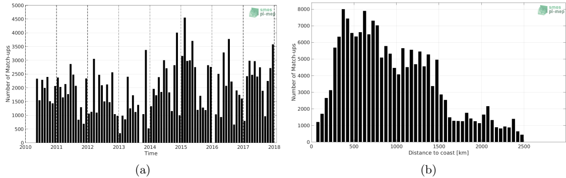
Figure 1: Number of match-ups between TSG (LEGOS-DM) and SMOS SSS L3 v2 - Daily - 0.5 Deg (CATDS-CECOS-IFREMER) SSS as a function of time (a) and as function of the distance to coast (b) over the North Pacific Ocean Pi-MEP region and for the full satellite product period.
