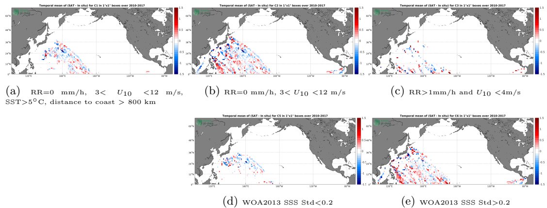
Figure 12: Temporal mean gridded over spatial boxes of size 1^\circ \times 1^\circ of \Delta SSS (SMOS L3 v2 - Daily - 0.5 Deg (CATDS-CECOS-IFREMER) - TSG-LEGOS-DM) for 5 different subdatasets corresponding to:RR=0 mm/h, 3 < U_{10} < 12 m/s, SST>5°C, distance to coast > 800 km (a), RR=0 mm/h, 3 < U_{10} < 12 m/s (b), RR>1mm/h and U_{10} < 4 m/s (c), WOA2013 SSS Std<0.2 (d), WOA2013 SSS Std>0.2 (e).
