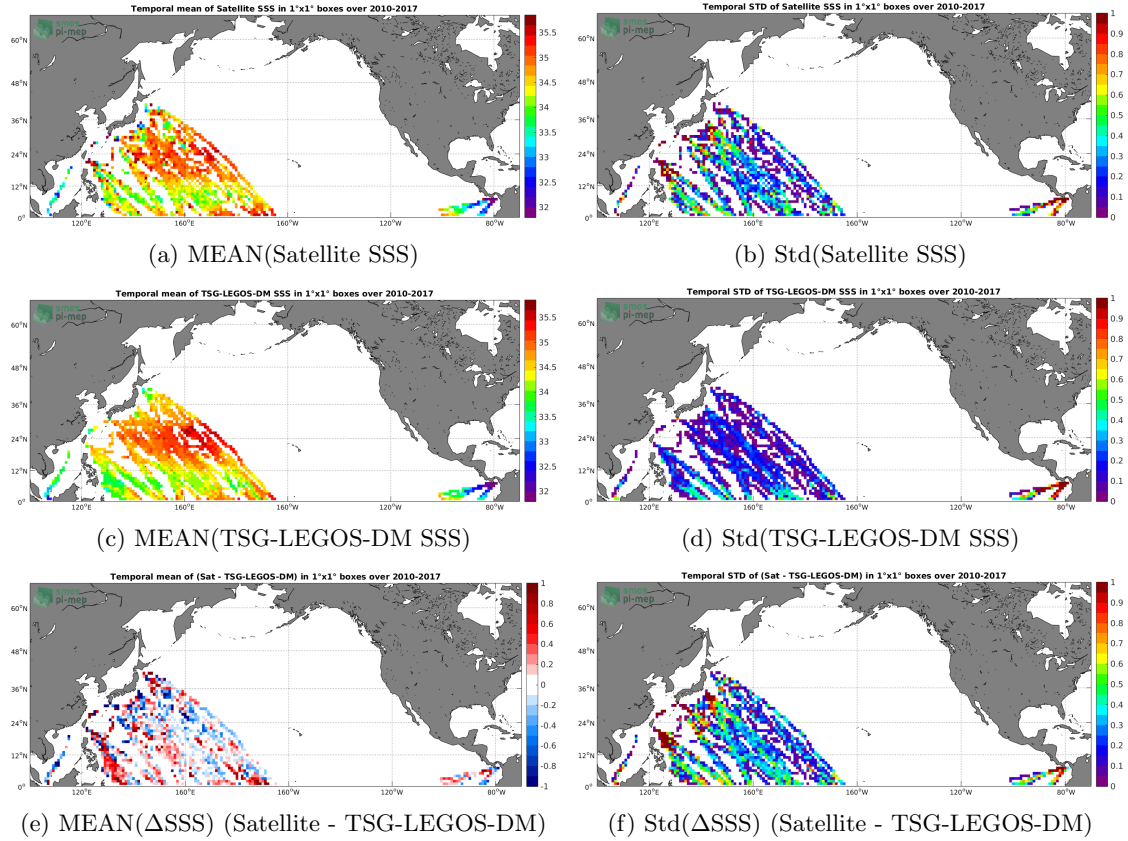
Figure 6: Temporal mean (left) and Std (right) of SSS from SMOS L3 v2 - Daily - 0.5 Deg (CATDS-CECOS-IFREMER) (top), TSG-LEGOS-DM (middle), and of \Delta SSS (Satellite - TSG-LEGOS-DM). Only match-up pairs are used to generate these maps.
