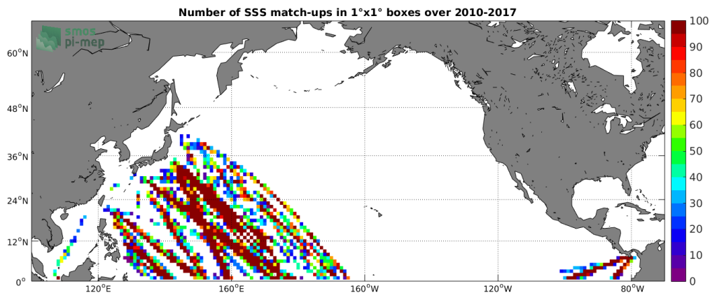
Figure 4: Number of SSS match-ups between TSG-LEGOS-DM SSS and the SMOS L3 v2 - Daily - 0.5 Deg (CATDS-CECOS-IFREMER) SSS product for the North Pacific Ocean Pi-MEP region over 1^\circ \times 1^\circ boxes and for the full satellite product period.
