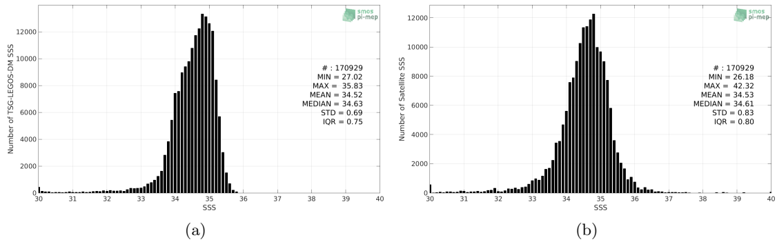
Figure 2: Histograms of SSS from TSG-LEGOS-DM (a) and SMOS L3 v2 - Daily - 0.5 Deg (CATDS-CECOS-IFREMER) (b) considering all match-up pairs per bins of 0.1 over the North Pacific Ocean Pi-MEP region and for the full satellite product period.
