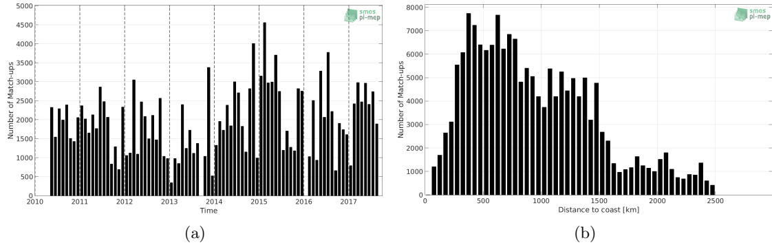
Figure 1: Number of match-ups between TSG-LEGOS-DM and SMOS L3 v2 - Daily - 0.5 Deg (CATDS-CECOS-IFREMER) SSS as a function of time (a) and as function of the distance to coast (b) over the North Pacific Ocean Pi-MEP region and for the full satellite product period.
