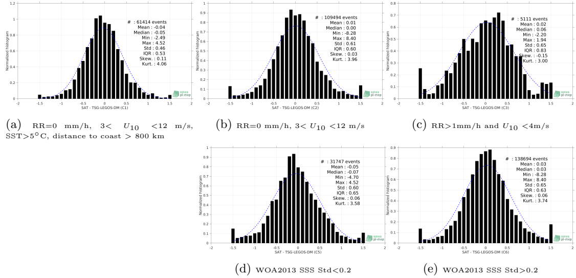
Figure 13: Normalized histogram of \Delta SSS (SMOS-L3-CATDS-CECOS-IFREMER-V2-1DAY-0.5DEG - TSG-LEGOS-DM) for 5 different subdatasets corresponding to: RR=0 mm/h, 3 < U_{10} < 12 m/s, SST>5°C, distance to coast > 800 km (a), RR=0 mm/h, 3 < U_{10} < 12 m/s (b), RR>1mm/h and U_{10} < 4 m/s (c), WOA2013 SSS Std<0.2 (d), WOA2013 SSS Std>0.2 (e).
