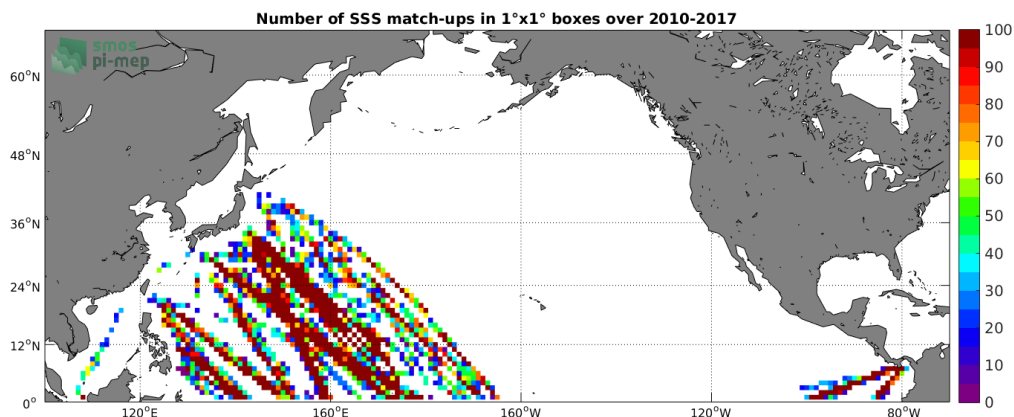
Figure 4: Number of SSS match-ups between TSG-LEGOS-DM SSS and the SMOS-L3-CATDS-CECOS-IFREMER-V2-1DAY-0.5DEG SSS product for the North Pacific Ocean Pi-MEP region over 1^\circ \times 1^\circ boxes and for the full satellite product period.
