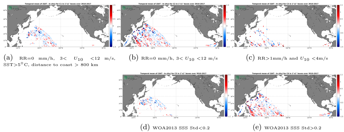
Figure 12: Temporal mean gridded over spatial boxes of size 1^\circ \times 1^\circ of \Delta SSS (SMOS-L3-CATDS-CECOS-IFREMER-V2-1DAY-0.5DEG - TSG-LEGOS-DM) for 5 different subdatasets corresponding to:RR=0 mm/h, 3 < U_{10} < 12 m/s, SST >5^\circ C, distance to coast > 800 km (a), RR=0 mm/h, 3 < U_{10} < 12 m/s (b), RR >1 mm/h and U_{10} < 4 m/s (c), WOA2013 SSS Std <0.2 (d), WOA2013 SSS Std >0.2 (e).
