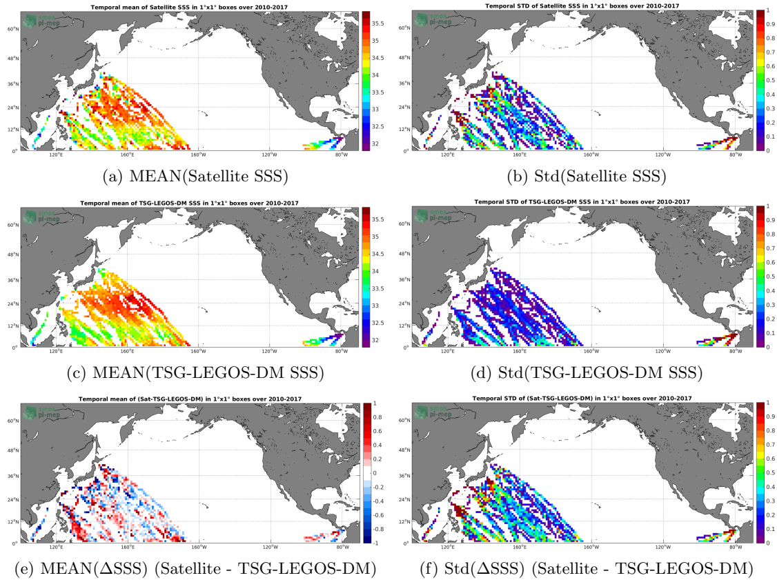
Figure 6: Temporal mean (left) and Std (right) of SSS from SMOS-L3-CATDS-CECOS-IFREMER-V2-1DAY-0.5DEG (top), TSG-LEGOS-DM (middle), and of \Delta SSS (Satellite - TSG-LEGOS-DM). Only match-up pairs are used to generate these maps.
