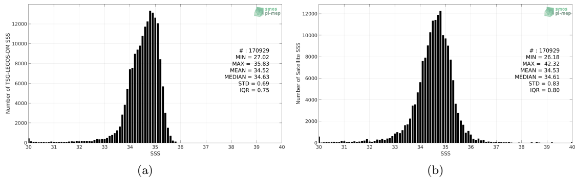
Figure 2: Histograms of SSS from TSG-LEGOS-DM (a) and SMOS-L3-CATDS-CECOS-IFREMER-V2-1DAY-0.5DEG (b) considering all match-up pairs per bins of 0.1 over the North Pacific Ocean Pi-MEP region and for the full satellite product period.
