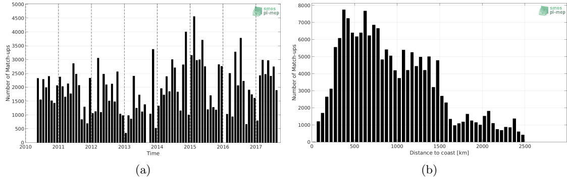
Figure 1: Number of match-ups between TSG-LEGOS-DM and SMOS-L3-CATDS-CECOS-IFREMER-V2-1DAY-0.5DEG SSS as a function of time (a) and as function of the distance to coast (b) over the North Pacific Ocean Pi-MEP region and for the full satellite product period.
