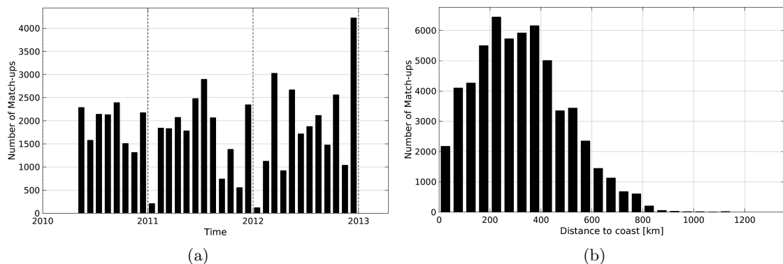
Figure 1: Number of match-ups between TSG-LEGOS-DM and SMOS-L3-CATDS-CECOS-IFREMER-V2-1DAY-0.5deg SSS as a function of time (a) and as function of the distance to coast (b) over the North Pacific Ocean Pi-MEP region and for the full satellite product period.
