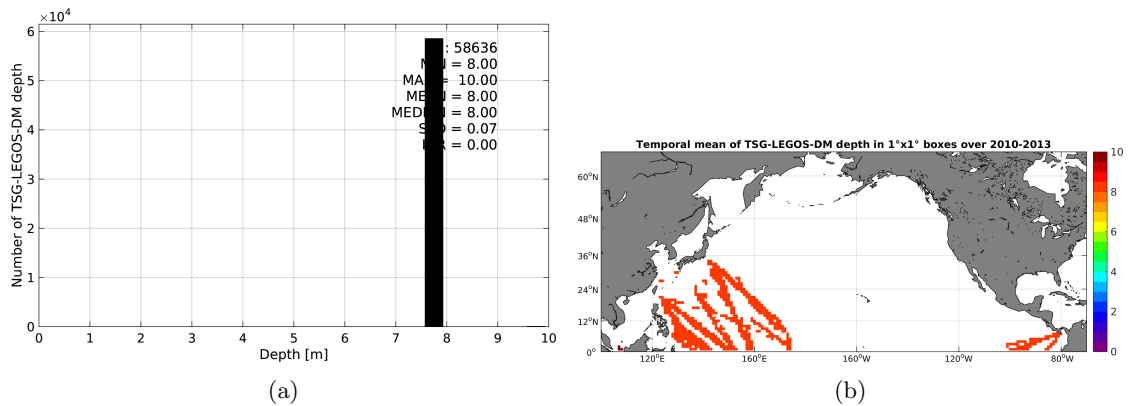
Figure 3: Histograms of the depth of the upper level SSS measurements from TSG-LEGOS-DM in the Match-up DataBase for the North Pacific Ocean Pi-MEP region (a) and temporal mean spatial distribution of pressure of the in situ SSS data over 1^\circ \times 1^\circ boxes and for the full satellite product period (b).
