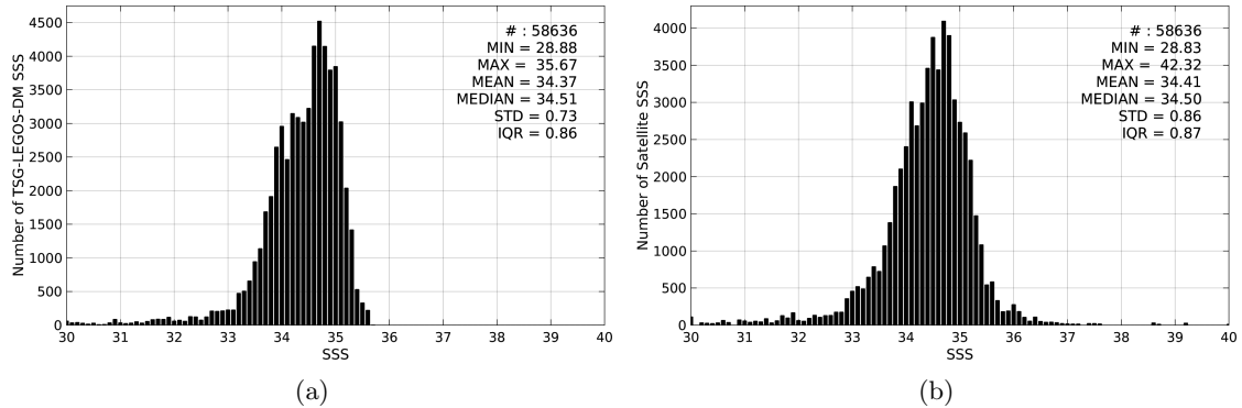
Figure 2: Histograms of SSS from TSG-LEGOS-DM (a) and SMOS-L3-CATDS-CECOS-IFREMER-V2-1DAY-0.5deg (b) considering all match-up pairs per bins of 0.1 over the North Pacific Ocean Pi-MEP region and for the full satellite product period.
