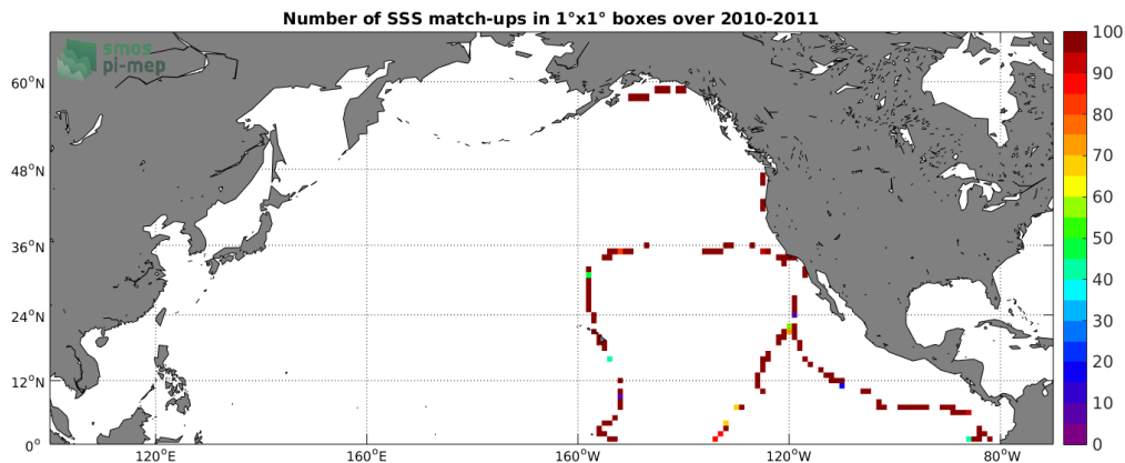
Figure 4: Number of SSS match-ups between TSG-GOSUD-Sailing-ship SSS and the SMOS L3 v2 - Daily - 0.5 Deg (CATDS-CECOS-IFREMER) SSS product for the North Pacific Ocean Pi-MEP region over 1^\circ \times 1^\circ boxes and for the full satellite product period.
