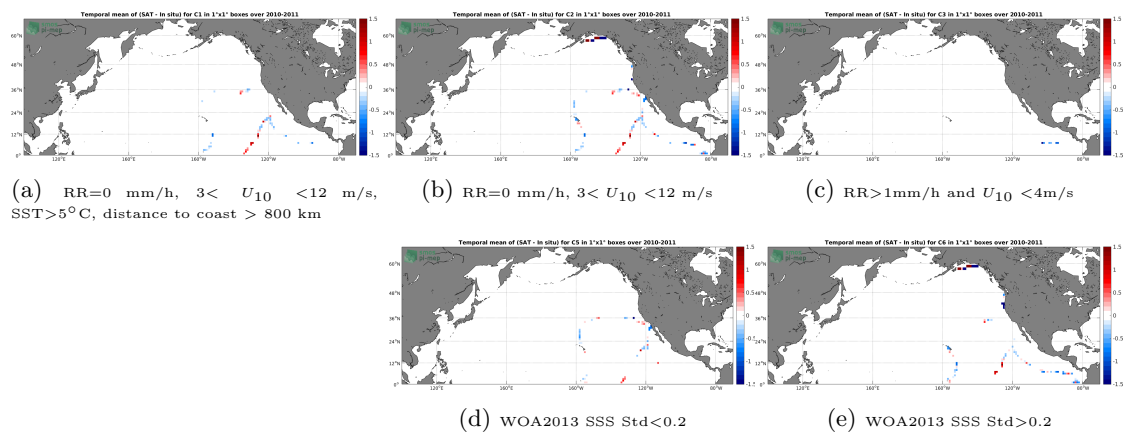
Figure 12: Temporal mean gridded over spatial boxes of size 1^\circ \times 1^\circ of \Delta SSS (SMOS L3 v2 - Daily - 0.5 Deg (CATDS-CECOS-IFREMER) - TSG-GOSUD-Sailing-ship) for 5 different subdatasets corresponding to:RR=0 mm/h, 3 < U_{10} < 12 m/s, SST>5°C, distance to coast > 800 km (a), RR=0 mm/h, 3 < U_{10} < 12 m/s (b), RR>1mm/h and U_{10} < 4 m/s (c), WOA2013 SSS Std<0.2 (d), WOA2013 SSS Std>0.2 (e).
