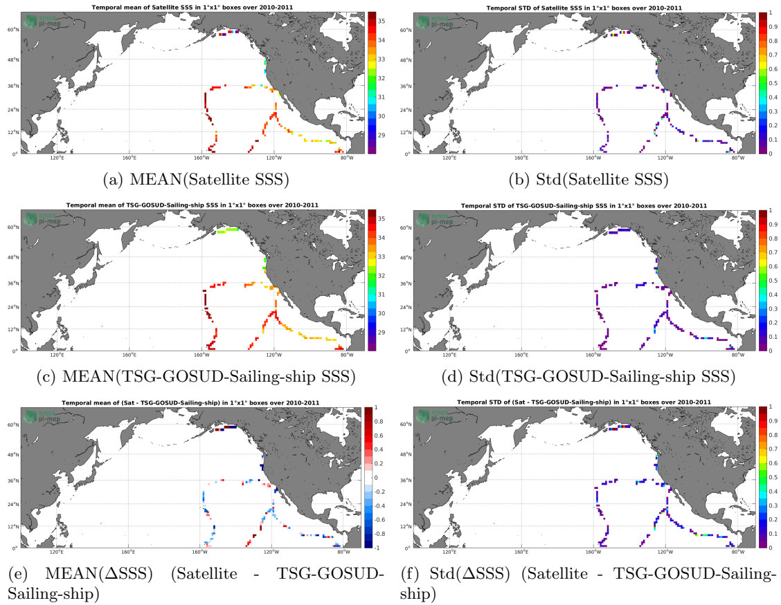
Figure 6: Temporal mean (left) and Std (right) of SSS from SMOS L3 v2 - Daily - 0.5 Deg (CATDS-CECOS-IFREMER) (top), TSG-GOSUD-Sailing-ship (middle), and of \Delta SSS (Satellite - TSG-GOSUD-Sailing-ship). Only match-up pairs are used to generate these maps.
