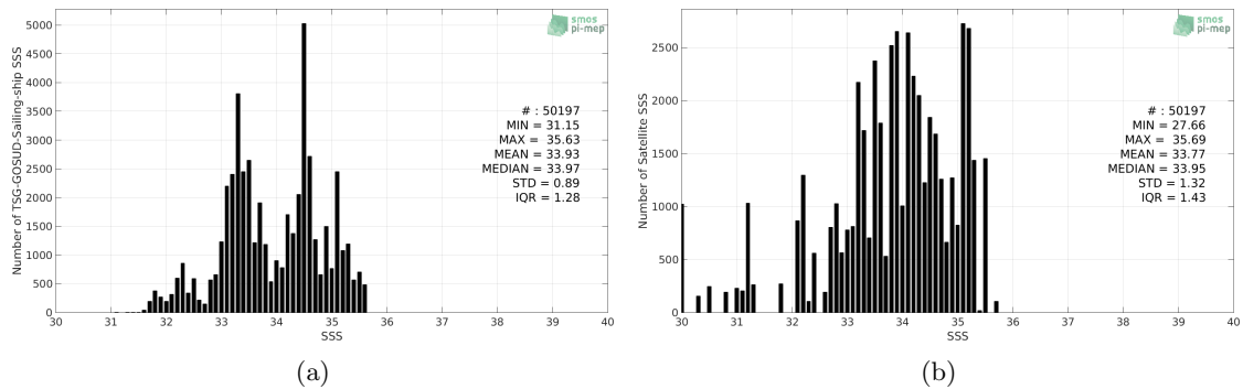
Figure 2: Histograms of SSS from TSG-GOSUD-Sailing-ship (a) and SMOS L3 v2 - Daily - 0.5 Deg (CATDS-CECOS-IFREMER) (b) considering all match-up pairs per bins of 0.1 over the North Pacific Ocean Pi-MEP region and for the full satellite product period.
