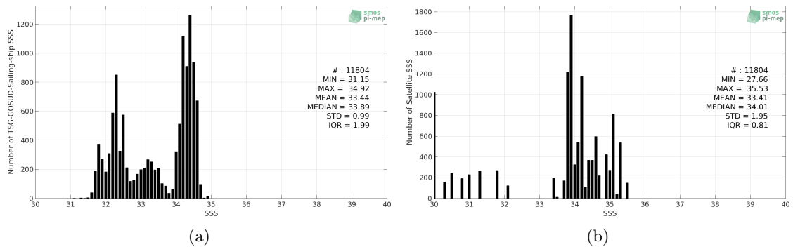
Figure 2: Histograms of SSS from TSG-GOSUD-Sailing-ship (a) and SMOS-L3-CATDS-CECOS-IFREMER-V2-1DAY-0.5DEG (b) considering all match-up pairs per bins of 0.1 over the North Pacific Ocean Pi-MEP region and for the full satellite product period.
