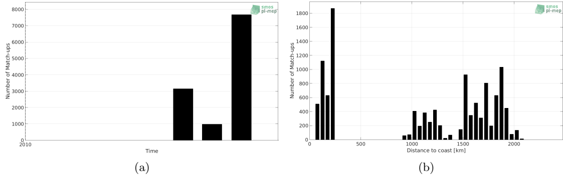
Figure 1: Number of match-ups between TSG-GOSUD-Sailing-ship and SMOS-L3-CATDS-CECOS-IFREMER-V2-1DAY-0.5DEG SSS as a function of time (a) and as function of the distance to coast (b) over the North Pacific Ocean Pi-MEP region and for the full satellite product period.
