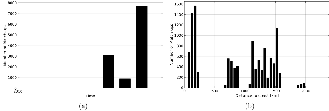
Figure 1: Number of match-ups between TSG-GOSUD-Sailing-ship and SMOS-L3-CATDS-CECOS-IFREMER-V2-1DAY-0.5DEG SSS as a function of time (a) and as function of the distance to coast (b) over the North Pacific Ocean Pi-MEP region and for the full satellite product period.
