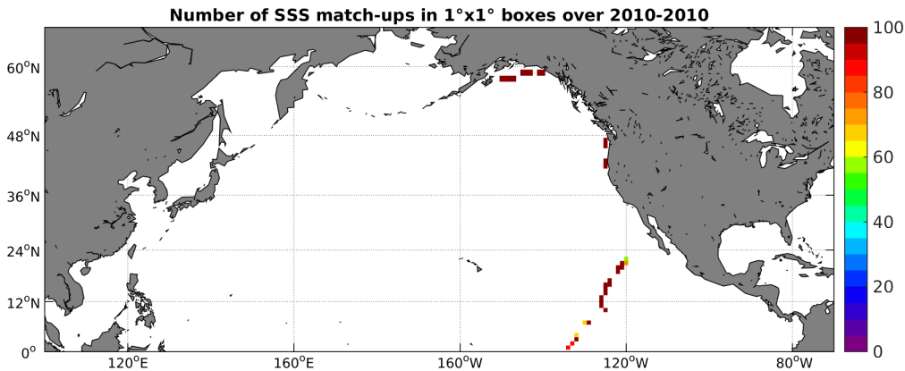
Figure 4: Number of SSS match-ups between TSG-GOSUD-Sailing-ship SSS and the SMOS-L3-CATDS-CECOS-IFREMER-V2-1DAY-0.5DEG SSS product for the North Pacific Ocean Pi-MEP region over 1^\circ \times 1^\circ boxes and for the full satellite product period.
