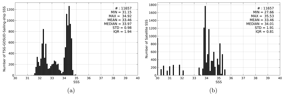
Figure 2: Histograms of SSS from TSG-GOSUD-Sailing-ship (a) and SMOS-L3-CATDS-CECOS-IFREMER-V2-1DAY-0.5DEG (b) considering all match-up pairs per bins of 0.1 over the North Pacific Ocean Pi-MEP region and for the full satellite product period.
