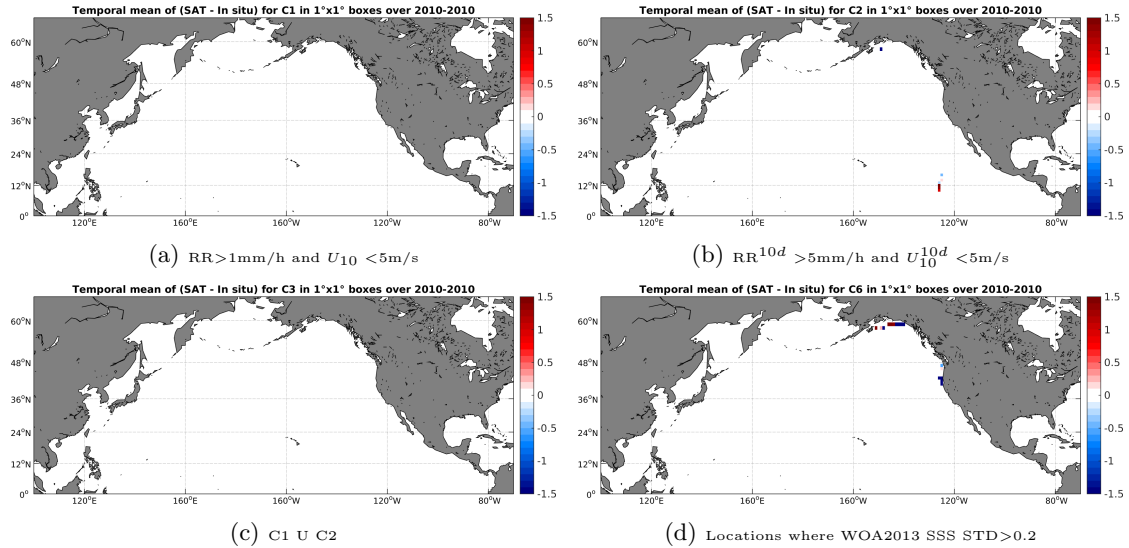
Figure 12: Temporal mean gridded over spatial boxes of size 1^\circ \times 1^\circ of \Delta SSS (SMOS-L3-CATDS-CECOS-IFREMER-V2-1DAY-0.5DEG - TSG-GOSUD-Sailing-ship) for 4 different subdatasets corresponding to: RR > 1mm/h and U_{10} < 5 m/s (a), RR^{10d} > 5 mm/h and U_{10}^{10d} < 5 m/s (b), C1 U C2 (c), Locations where WOA2013 SSS STD > 0.2 (d).
