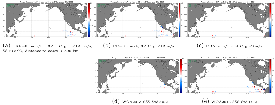
Figure 12: Temporal mean gridded over spatial boxes of size 1^\circ \times 1^\circ of \Delta SSS (SMOS SSS L3 v2 - Daily - 0.5 Deg (CATDS-CECOS-IFREMER) - TSG (GOSUD-Research-vessel)) for 5 different subdatasets corresponding to:RR=0 mm/h, 3 < U_{10} < 12 m/s, SST >5^\circ\text{C} , distance to coast > 800 km (a), RR=0 mm/h, 3 < U_{10} < 12 m/s (b), RR >1 mm/h and U_{10} < 4 m/s (c), WOA2013 SSS Std <0.2 (d), WOA2013 SSS Std >0.2 (e).
