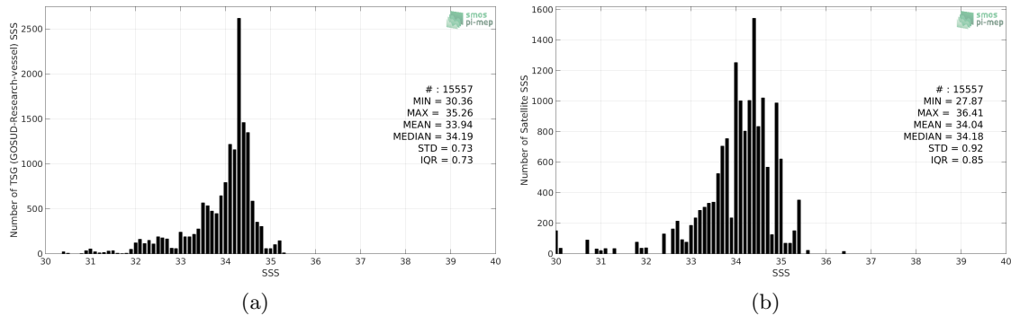
Figure 2: Histograms of SSS from TSG (GOSUD-Research-vessel) (a) and SMOS SSS L3 v2 - Daily - 0.5 Deg (CATDS-CECOS-IFREMER) (b) considering all match-up pairs per bins of 0.1 over the North Pacific Ocean Pi-MEP region and for the full satellite product period.
