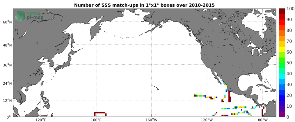
Figure 4: Number of SSS match-ups between TSG (GOSUD-Research-vessel) SSS and the SMOS SSS L3 v2 - Daily - 0.5 Deg (CATDS-CECOS-IFREMER) SSS product for the North Pacific Ocean Pi-MEP region over 1^\circ \times 1^\circ boxes and for the full satellite product period.
