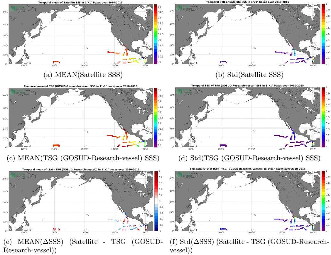
Figure 6: Temporal mean (left) and Std (right) of SSS from SMOS SSS L3 v2 - Daily - 0.5 Deg (CATDS-CECOS-IFREMER) (top), TSG (GOSUD-Research-vessel) (middle), and of \Delta SSS (Satellite - TSG (GOSUD-Research-vessel)). Only match-up pairs are used to generate these maps.
