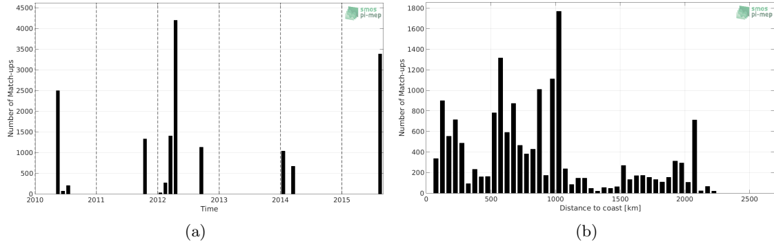
Figure 1: Number of match-ups between TSG-GOSUD-Research-vessel and SMOS-L3-CATDS-CECOS-IFREMER-V2-1DAY-0.5DEG SSS as a function of time (a) and as function of the distance to coast (b) over the North Pacific Ocean Pi-MEP region and for the full satellite product period.
