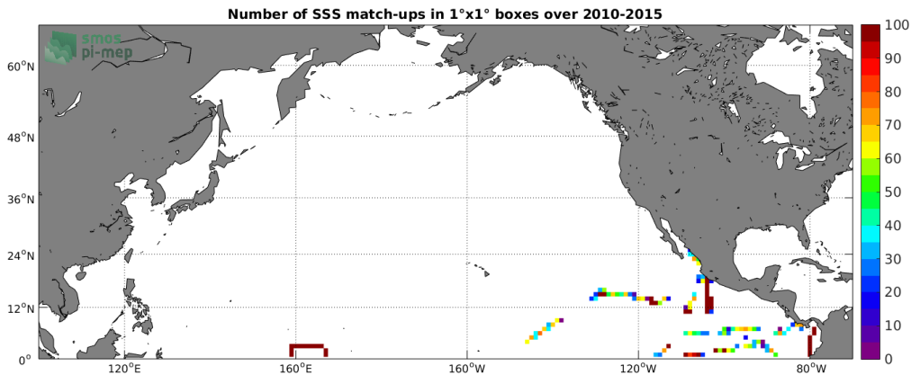
Figure 4: Number of SSS match-ups between TSG-GOSUD-Research-vessel SSS and the SMOS-L3-CATDS-CECOS-IFREMER-V2-1DAY-0.5DEG SSS product for the North Pacific Ocean Pi-MEP region over 1^\circ \times 1^\circ boxes and for the full satellite product period.
