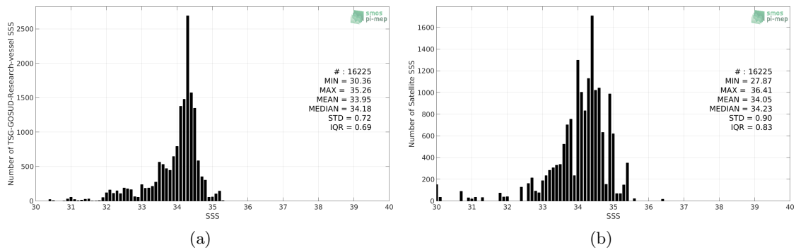
Figure 2: Histograms of SSS from TSG-GOSUD-Research-vessel (a) and SMOS-L3-CATDS-CECOS-IFREMER-V2-1DAY-0.5DEG (b) considering all match-up pairs per bins of 0.1 over the North Pacific Ocean Pi-MEP region and for the full satellite product period.
