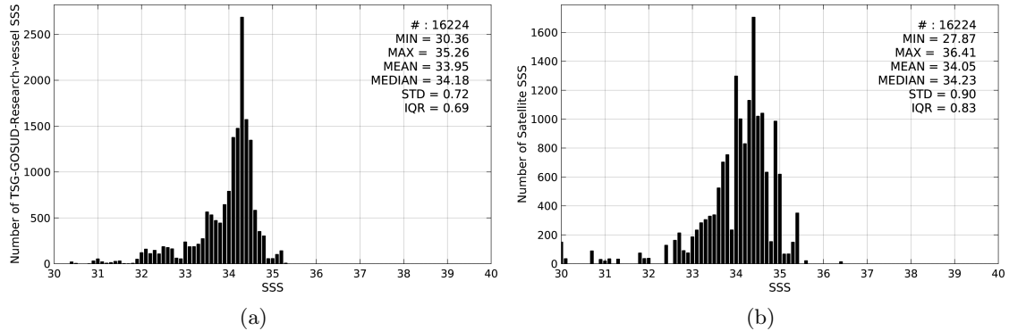
Figure 2: Histograms of SSS from TSG-GOSUD-Research-vessel (a) and SMOS-L3-CATDS-CECOS-IFREMER-V2-1DAY-0.5deg (b) considering all match-up pairs per bins of 0.1 over the North Pacific Ocean Pi-MEP region and for the full satellite product period.
