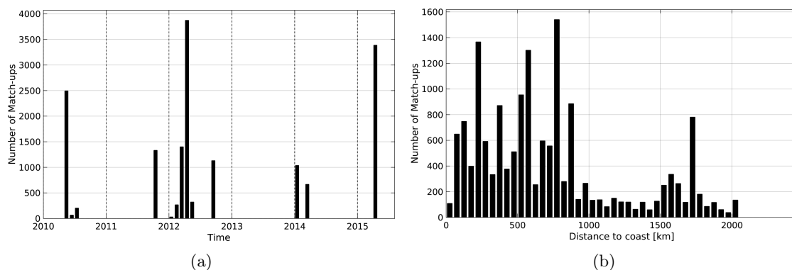
Figure 1: Number of match-ups between TSG-GOSUD-Research-vessel and SMOS-L3-CATDS-CECOS-IFREMER-V2-1DAY-0.5deg SSS as a function of time (a) and as function of the distance to coast (b) over the North Pacific Ocean Pi-MEP region and for the full satellite product period.
