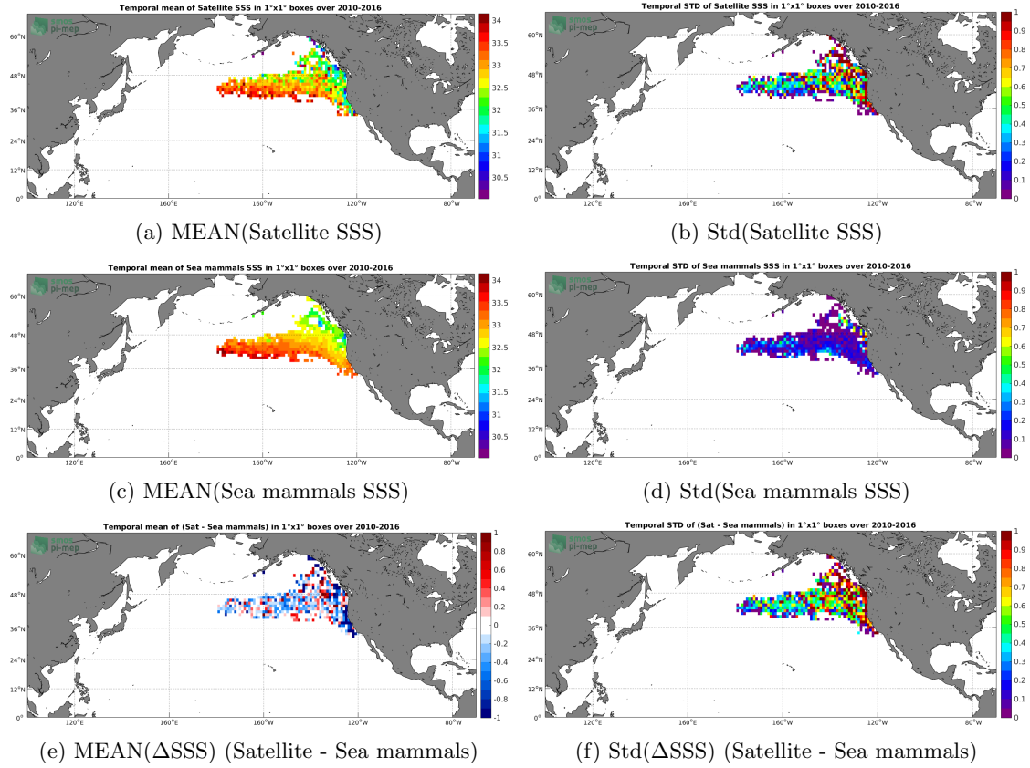
Figure 6: Temporal mean (left) and Std (right) of SSS from SMOS SSS L3 v2 - Daily - 0.5 Deg (CATDS-CECOS-IFREMER) (top), Sea mammals (middle), and of \Delta SSS (Satellite - Sea mammals). Only match-up pairs are used to generate these maps.
