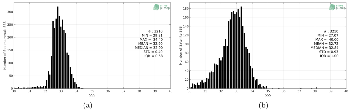
Figure 2: Histograms of SSS from Sea mammals (a) and SMOS SSS L3 v2 - Daily - 0.5 Deg (CATDS-CECOS-IFREMER) (b) considering all match-up pairs per bins of 0.1 over the North Pacific Ocean Pi-MEP region and for the full satellite product period.
