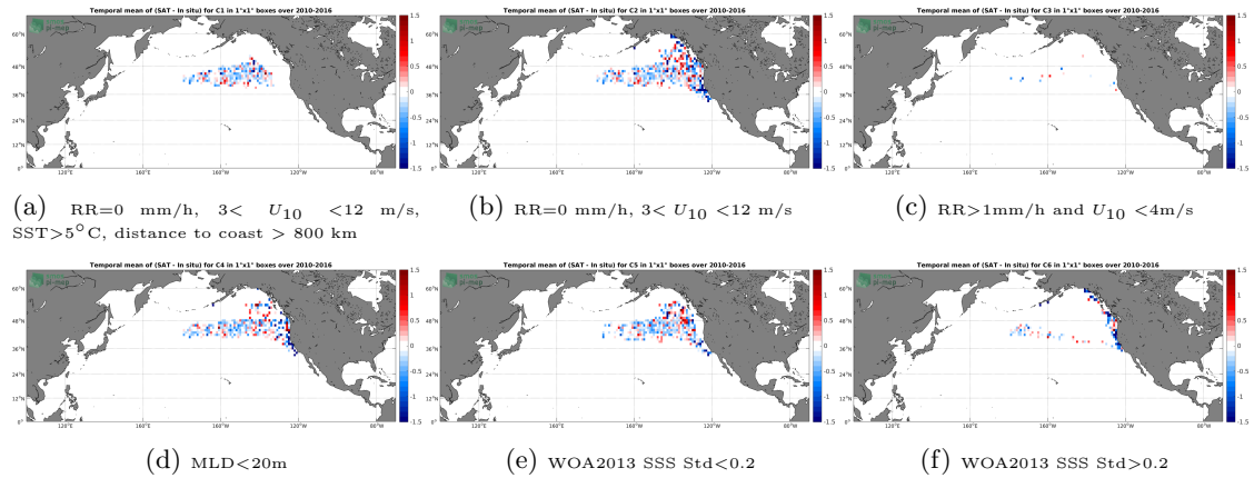
Figure 12: Temporal mean gridded over spatial boxes of size 1^{\circ}\times 1^{\circ} of \Delta\text{SSS} (SMOS SSS L3 v2 - Daily - 0.5 Deg (CATDS-CECOS-IFREMER) - Sea mammals) for 6 different subdatasets corresponding to:RR=0 mm/h, 3 < U_{10} < 12 m/s, SST >5^{\circ}\text{C} , distance to coast > 800 km (a), RR=0 mm/h, 3 < U_{10} < 12 m/s (b), RR >1 mm/h and U_{10} < 4 m/s (c),MLD <20 m (d),WOA2013 SSS Std <0.2 (e),WOA2013 SSS Std >0.2 (f).
