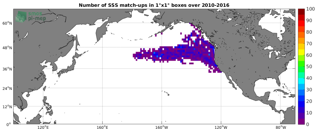
Figure 4: Number of SSS match-ups between Sea mammals SSS and the SMOS SSS L3 v2 - Daily - 0.5 Deg (CATDS-CECOS-IFREMER) SSS product for the North Pacific Ocean Pi-MEP region over 1^\circ \times 1^\circ boxes and for the full satellite product period.
