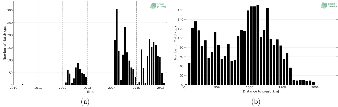
Figure 1: Number of match-ups between Sea mammals and SMOS SSS L3 v2 - Daily - 0.5 Deg (CATDS-CECOS-IFREMER) SSS as a function of time (a) and as function of the distance to coast (b) over the North Pacific Ocean Pi-MEP region and for the full satellite product period.
