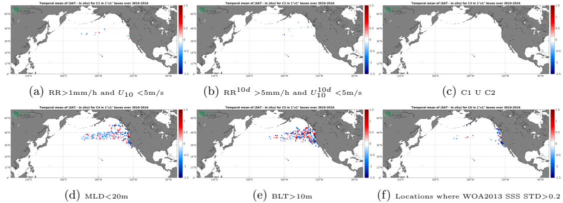
Figure 12: Temporal mean gridded over spatial boxes of size 1°x1° of \Delta SSS (SMOS-L3-CATDS-CECOS-IFREMER-V2-1DAY-0.5DEG - Sea mammals) for 6 different subdatasets corresponding to:RR>1mm/h and U_{10} < 5m/s (a), RR^{10d} > 5mm/h and U_{10}^{10d} < 5m/s (b), C1 U C2 (c),MLD<20m (d),BLT>10m (e),Locations where WOA2013 SSS STD>0.2 (f).
