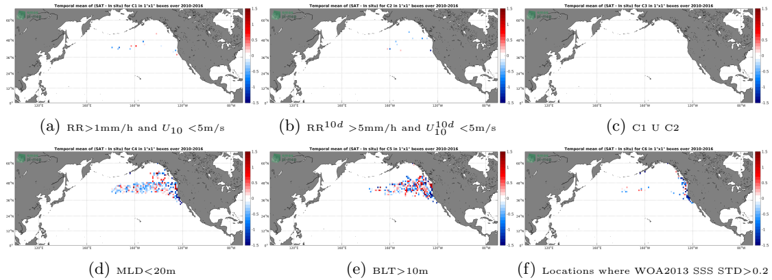
Figure 12: Temporal mean gridded over spatial boxes of size 1°x1° of ΔSSS (SMOS-L3-CATDS-CECOS-IFREMER-V2-1DAY-0.5DEG - Sea mammals) for 6 different subdatasets corresponding to:RR>1mm/h and U_{10} < 5\text{m/s} (a), RR^{10d} > 5\text{mm/h} and U_{10}^{10d} < 5\text{m/s} (b), C1 U C2 (c),MLD<20m (d),BLT>10m (e),Locations where WOA2013 SSS STD>0.2 (f).
