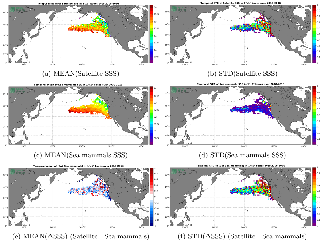
Figure 6: Temporal mean (left) and STD (right) of SSS from SMOS-L3-CATDS-CECOS-IFREMER-V2-1DAY-0.5DEG (top), Sea mammals (middle), and of \Delta SSS (Satellite - Sea mammals). Only match-up pairs are used to generate these maps.
