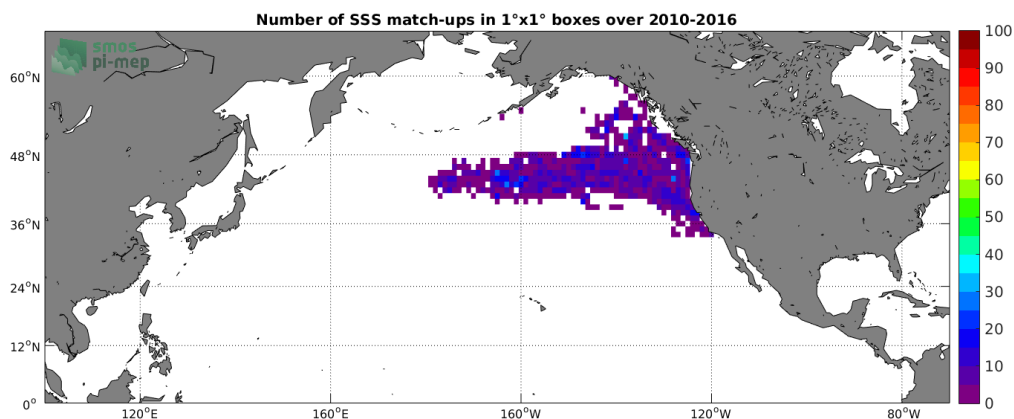
Figure 4: Number of SSS match-ups between Sea mammals SSS and the SMOS-L3-CATDS-CECOS-IFREMER-V2-1DAY-0.5DEG SSS product for the North Pacific Ocean Pi-MEP region over 1°x1° boxes and for the full satellite product period.
