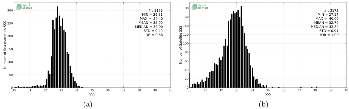
Figure 2: Histograms of SSS from Sea mammals (a) and SMOS-L3-CATDS-CECOS-IFREMER-V2-1DAY-0.5DEG (b) considering all match-up pairs per bins of 0.1 over the North Pacific Ocean Pi-MEP region and for the full satellite product period.
