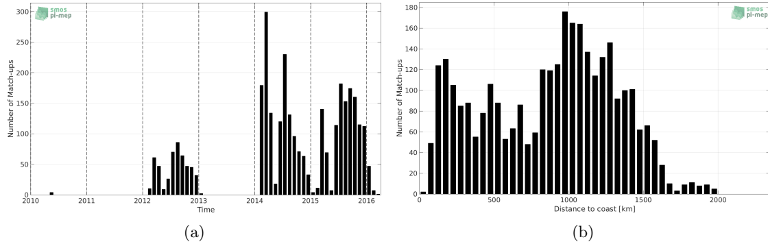
Figure 1: Number of match-ups between Sea mammals and SMOS-L3-CATDS-CECOS-IFREMER-V2-1DAY-0.5DEG SSS as a function of time (a) and as function of the distance to coast (b) over the North Pacific Ocean Pi-MEP region and for the full satellite product period.
