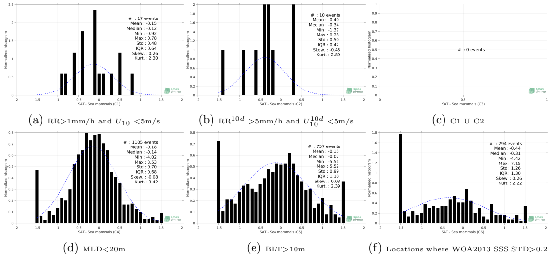
Figure 13: Normalized histogram of ΔSSS (SMOS-L3-CATDS-CECOS-IFREMER-V2-1DAY-0.5DEG - Sea mammals) for 6 different subdatasets corresponding to: RR>1mm/h and U_{10} < 5\text{m/s} (a), RR^{10d} > 5\text{mm/h} and U_{10}^{10d} < 5\text{m/s} (b), C1 U C2 (c),MLD<20m (d),BLT>10m (e),Locations where WOA2013 SSS STD>0.2 (f).
