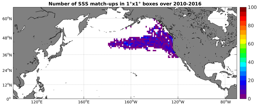
Figure 4: Number of SSS match-ups between Sea mammals SSS and the SMOS-L3-CATDS-CECOS-IFREMER-V2-1DAY-0.5deg SSS product for the North Pacific Ocean Pi-MEP region over 1^\circ \times 1^\circ boxes and for the full satellite product period.
