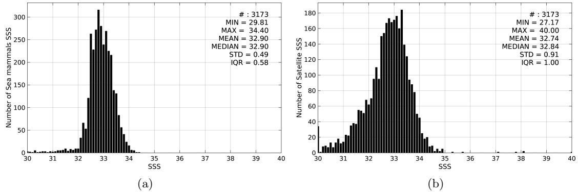
Figure 2: Histograms of SSS from Sea mammals (a) and SMOS-L3-CATDS-CECOS-IFREMER-V2-1DAY-0.5deg (b) considering all match-up pairs per bins of 0.1 over the North Pacific Ocean Pi-MEP region and for the full satellite product period.
