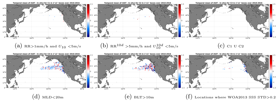
Figure 12: Temporal mean gridded over spatial boxes of size 1^\circ \times 1^\circ of \Delta SSS (SMOS-L3-CATDS-CECOS-IFREMER-V2-1DAY-0.5deg - Sea mammals) for 6 different subdatasets corresponding to: RR > 1\text{mm/h} and U_{10} < 5\text{m/s} (a), RR^{10d} > 5\text{mm/h} and U_{10}^{10d} < 5\text{m/s} (b), C1 U C2 (c), MLD < 20\text{m} (d), BLT > 10\text{m} (e), Locations where WOA2013 SSS STD > 0.2 (f).
