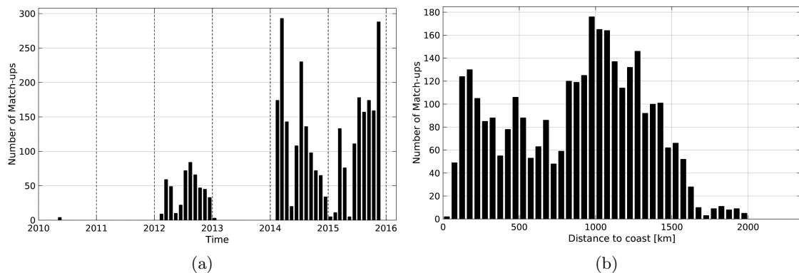
Figure 1: Number of match-ups between Sea mammals and SMOS-L3-CATDS-CECOS-IFREMER-V2-1DAY-0.5deg SSS as a function of time (a) and as function of the distance to coast (b) over the North Pacific Ocean Pi-MEP region and for the full satellite product period.
