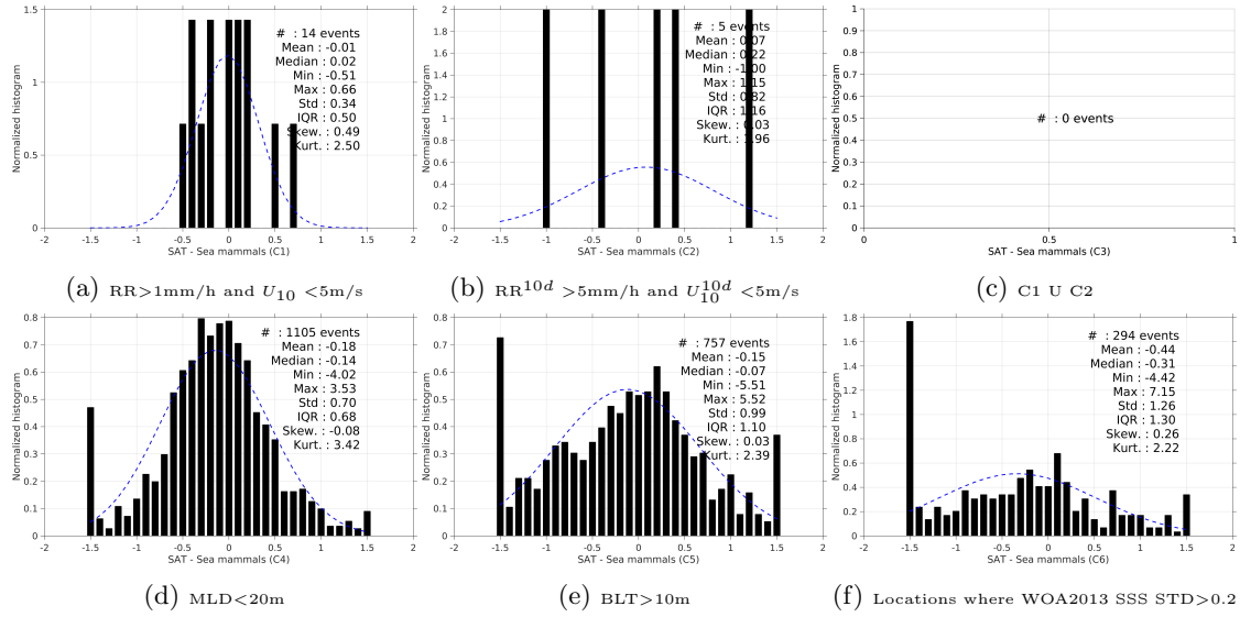
Figure 13: Normalized histogram of \Delta\text{SSS} (SMOS-L3-CATDS-CECOS-IFREMER-V2-1DAY-0.5deg - Sea mammals) for 6 different subdatasets corresponding to: RR > 1mm/h and U_{10} < 5\text{m/s} (a), RR^{10d} > 5\text{mm/h} and U_{10}^{10d} < 5\text{m/s} (b), C1 U C2 (c), MLD < 20m (d), BLT > 10m (e), Locations where WOA2013 SSS STD > 0.2 (f).
